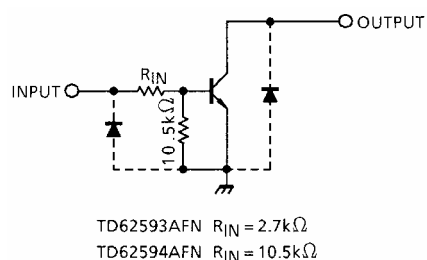
TD62593AFN, TD62594AFN
