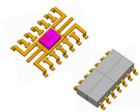
Figure 17. Internal construction of the package simulation.
