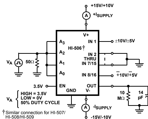
FIGURE 4B. TEST CIRCUIT
