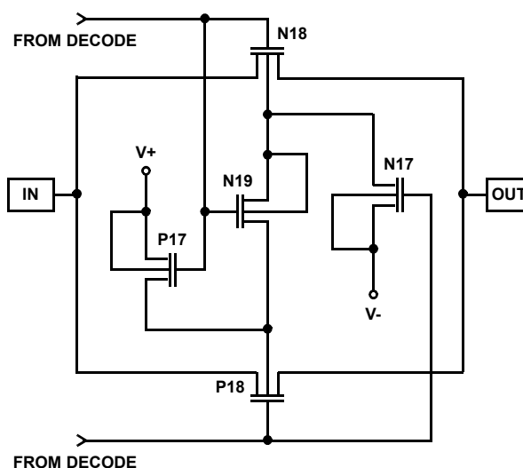
MULTIPLEX SWITCH
