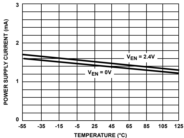
FIGURE 10A. HI-506/HI-507
