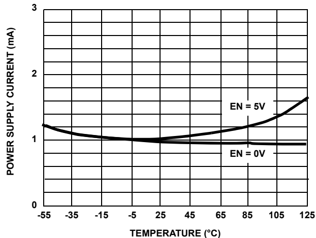
FIGURE 10B. HI-508/HI-509
