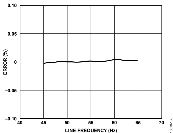
Figure 29. Voltage Channel RMS Error vs. Line Frequency
