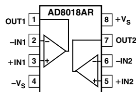
8-Lead SOIC (Thermal Coastline)
