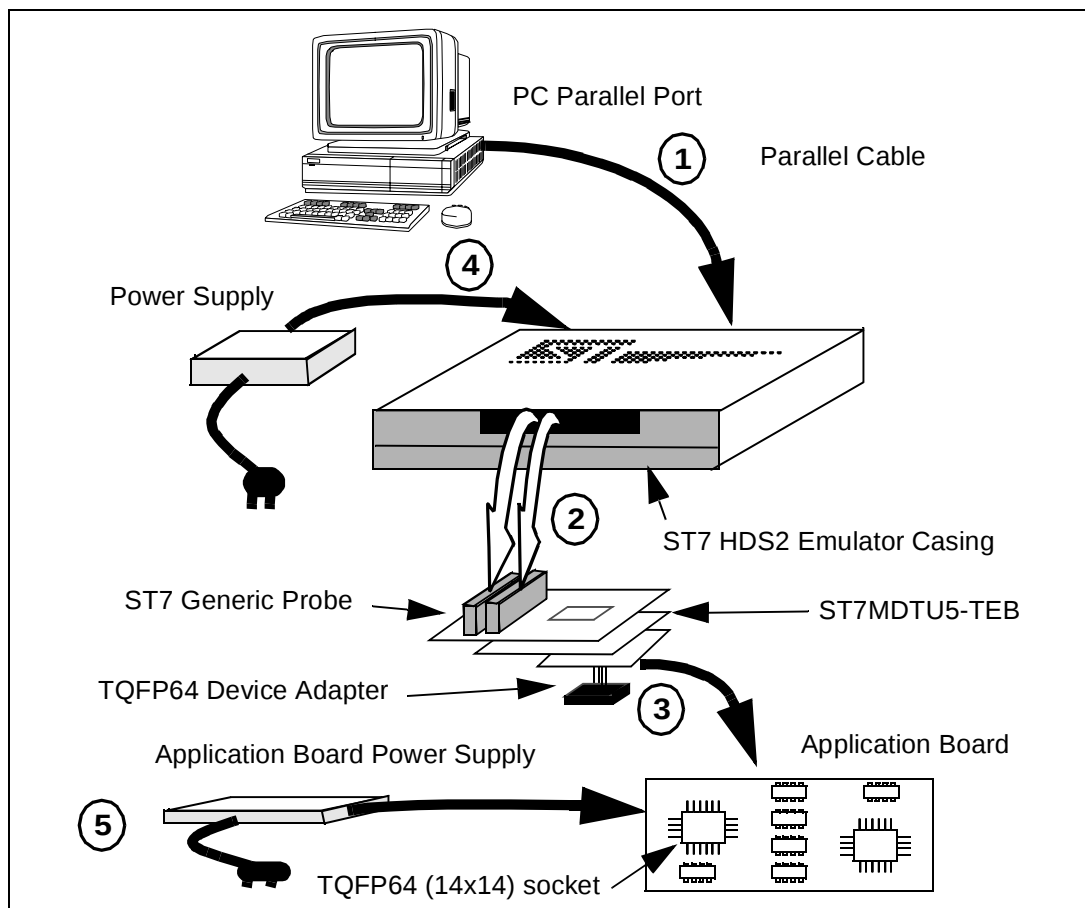
Figure 3: ST7MDTU5-EMU2B connection flow
