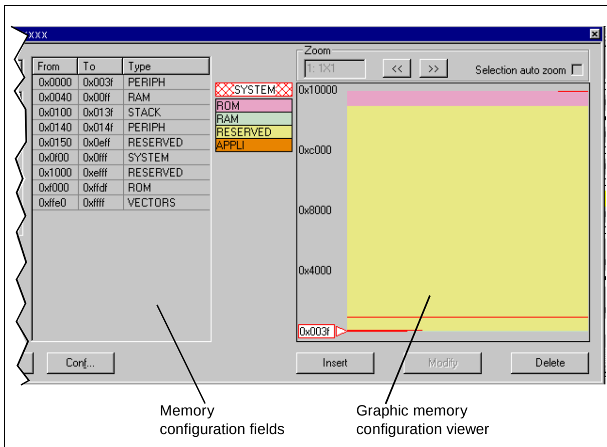
Figure 24: Memory mapping
