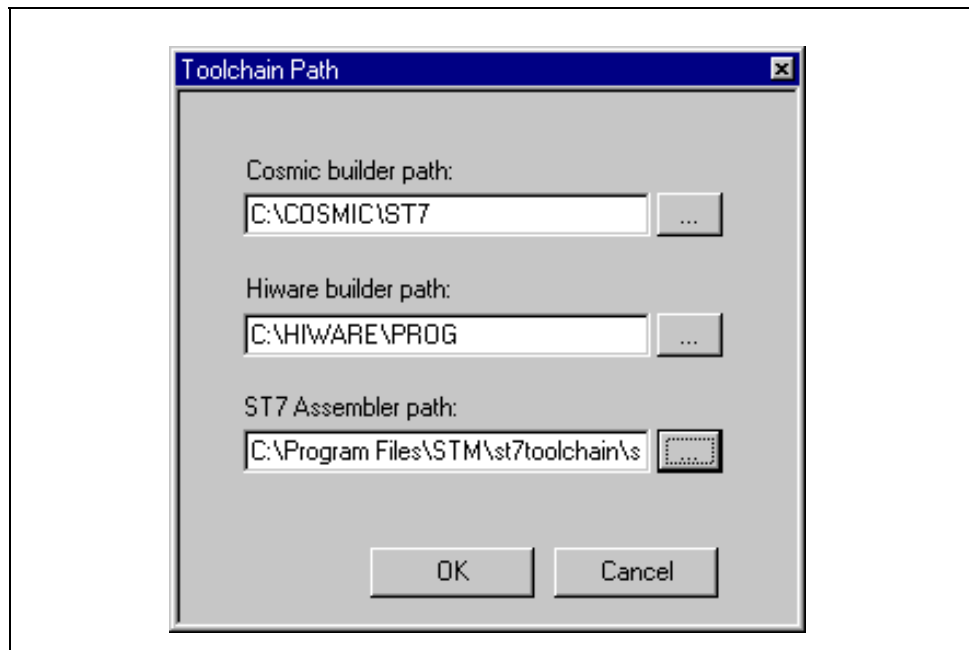
Figure 20: Toolchain paths
