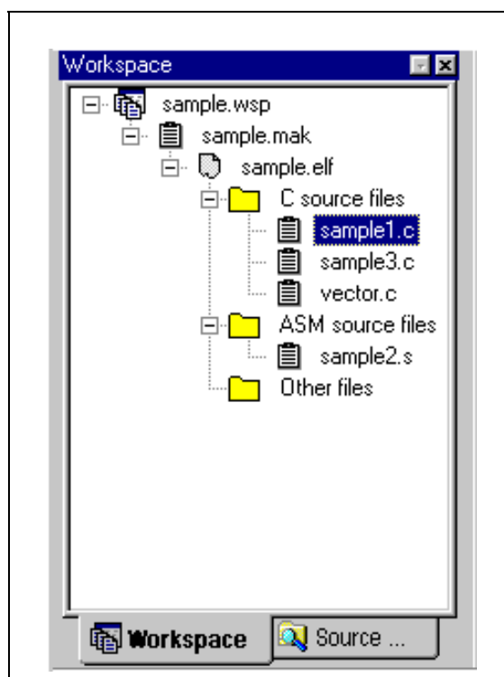
Figure 13: Workspace window
