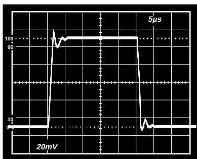
Figure 22d. Unity Gain Inverter Small Signal Pulse Response C_i = 1000 \text{ pF}
