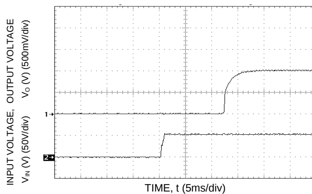
Figure 47. Typical Start-Up with application of V_{in} .
