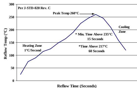
Figure 74. Recommended linear reflow profile using Sn/Ag/Cu solder.
