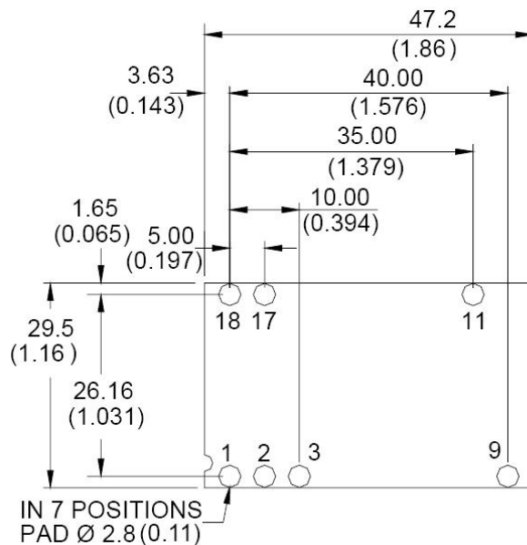
Surface Mount Pad Layout – Component side view
