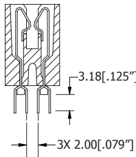
STAGGERED DIP SOLDER (HH)
