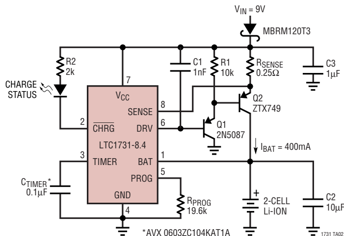
Linear Charger Using a PNP Transistor
