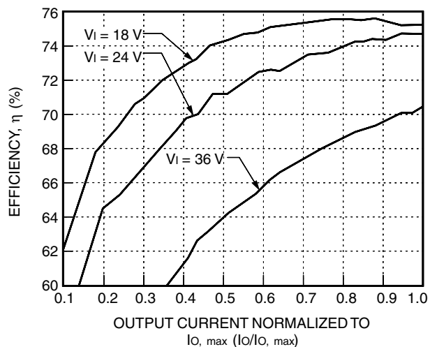
Figure 7. LC005B Typical Efficiency vs. Normalized Output Current at T_c = 25^\circ\text{C}
