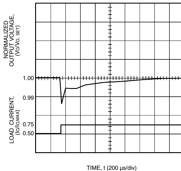
Figure 12. Typical Output Voltage for Step Load Change from 50% to 75% of I_o = I_{o, \max} at T_c = 25^\circ\text{C}
