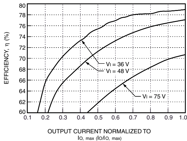
Figure 10. LW005B Typical Efficiency vs. Normalized Output Current at T_c = 25^\circ\text{C}
