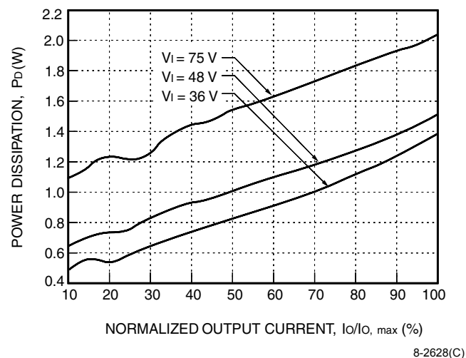
Figure 28. LW005B Power Dissipation vs. Output Current
