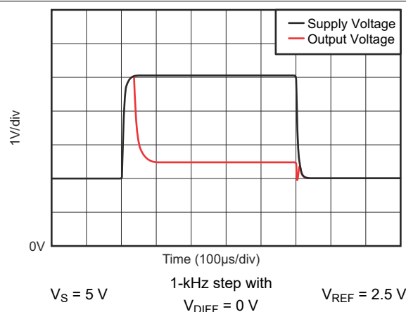
Figure 5-22. Brownout Recovery
