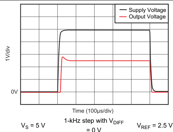
Figure 5-21. Start-Up Response
