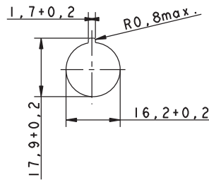
→ Illumination Color of mushroom Order no. no opaque red 1.30.074.281/0300
