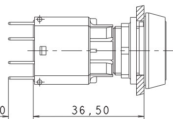
with contact block / lamp socket
