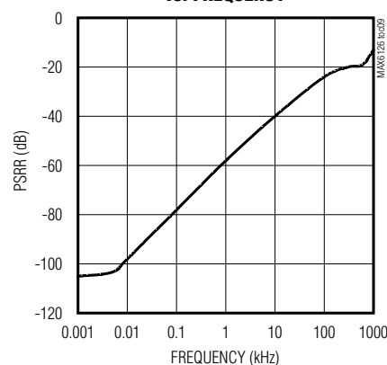
MAX6126_21 POWER-SUPPLY REJECTION RATIO vs. FREQUENCY
