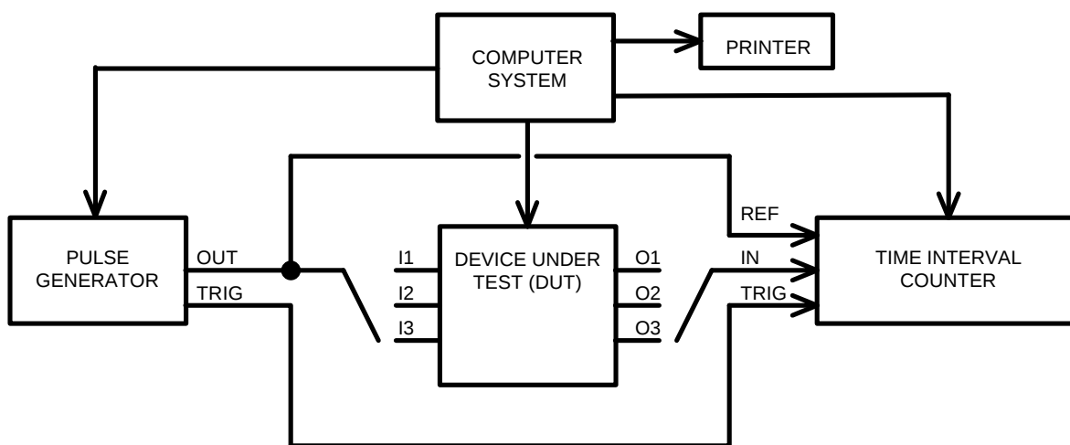
Test Setup
