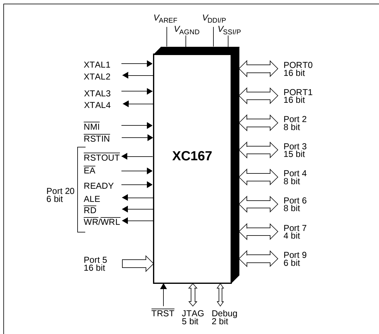
Figure 1 Logic Symbol
