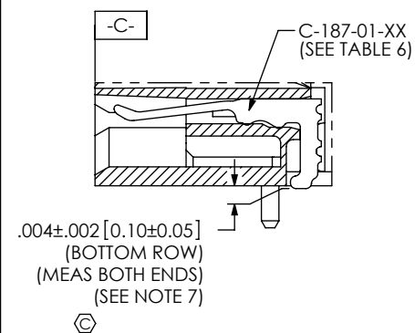
BOTTOM ROW - TAIL DETAIL (LOCATE ASSEMBLY ON DATUM -C- FOR MEASUREMENT)
