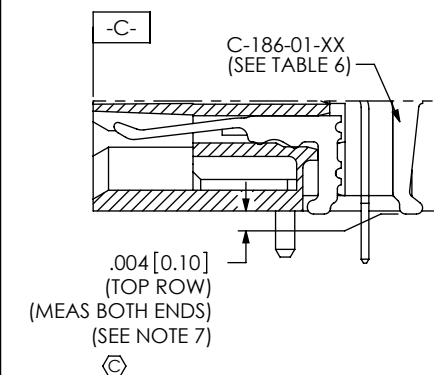
TOP ROW - TAIL DETAIL (LOCATE ASSEMBLY ON DATUM -C- FOR MEASUREMENT)
