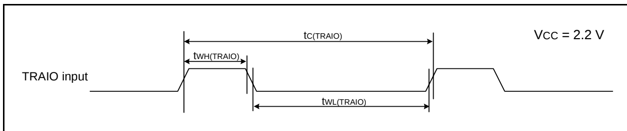
Figure 5.25 TRAIO Input Timing Diagram when V_{CC} = 2.2\text{ V}
