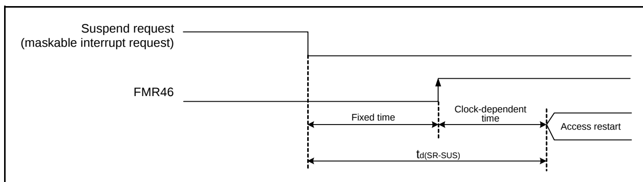
Figure 5.17 Time delay until Suspend
