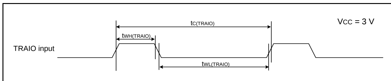
Figure 5.22 TRAIO Input Timing Diagram when V_{CC} = 3\text{ V}
