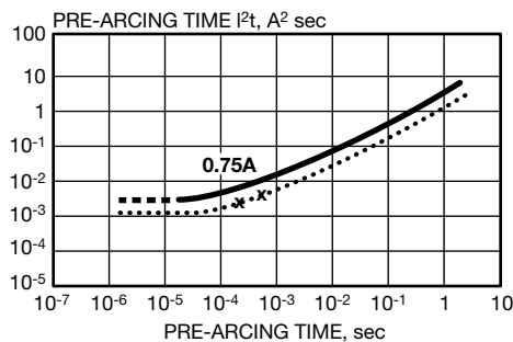
Fig. 5b. Choice of fuse, example #5.
