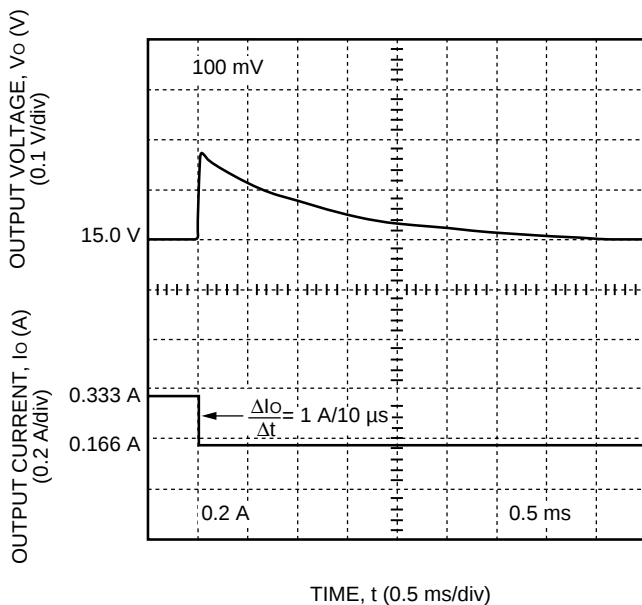
Figure 6. DC025 Dual-Output-Series Typical 15 V Output Voltage Response to a Step Load Change from 50% to 25% of I_{o,max} at V_i = V_{i,nom} and T_c = 25^\circ\text{C}
