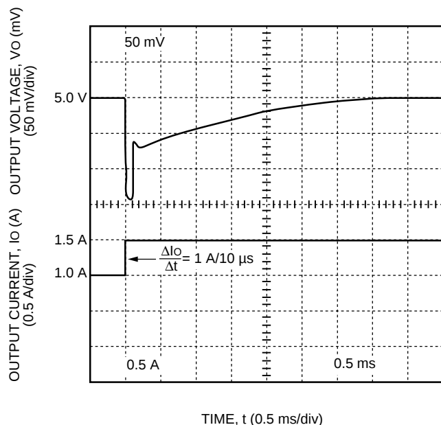
Figure 7. DC025 Dual-Output-Series Typical 5 V Output Voltage Response to a Step Load Change from 50% to 75% of I_{o,max} at V_i = V_{i,nom} and T_c = 25^\circ\text{C}
