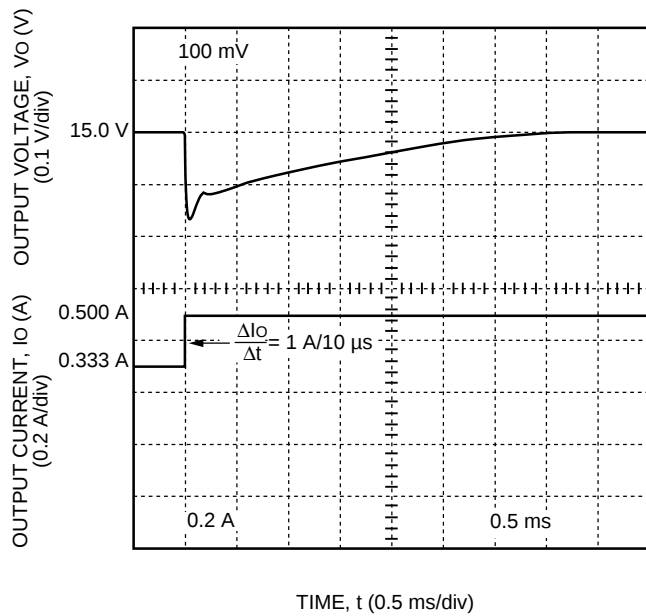
Figure 9. DC025 Dual-Output-Series Typical 15 V Output Voltage Response to a Step Load Change from 50% to 75% of I_{o,max} at V_i = V_{i,nom} and T_c = 25^\circ\text{C}
