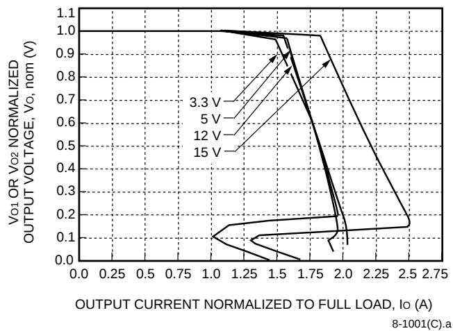
Figure 2. DC025 Dual-Output-Series Normalized Output Current vs. Normalized Output Voltage at V_i = 28\text{ V} and T_c = 25^\circ\text{C}
