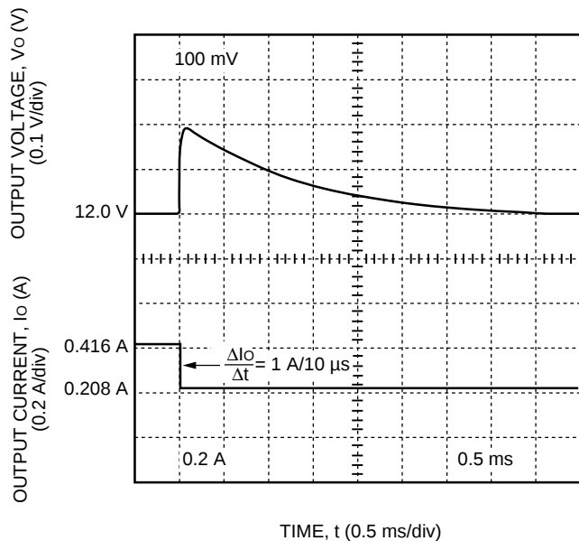
Figure 5. DC025 Dual-Output-Series Typical 12 V Output Voltage Response to a Step Load Change from 50% to 25% of I_{o,max} at V_i = V_{i,nom} and T_c = 25^\circ\text{C}
