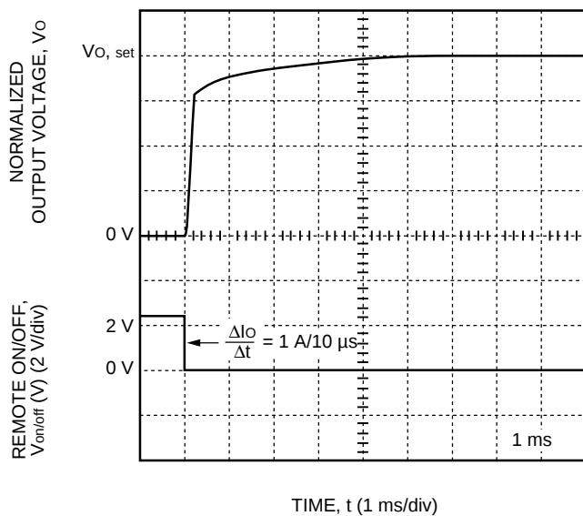
Figure 10. DC025 Dual-Output-Series Typical Output Voltage Rise Time with Remote On/Off at V_i = V_{i,nom} , I_o = 0.8 (I_{o,max}) , and T_c = 25^\circ\text{C}
