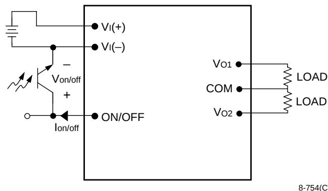
Figure 14. Remote On/Off Implementation
