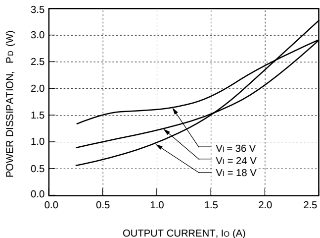
Figure 16. 3.3 V Output Power Dissipation vs. Output Current
