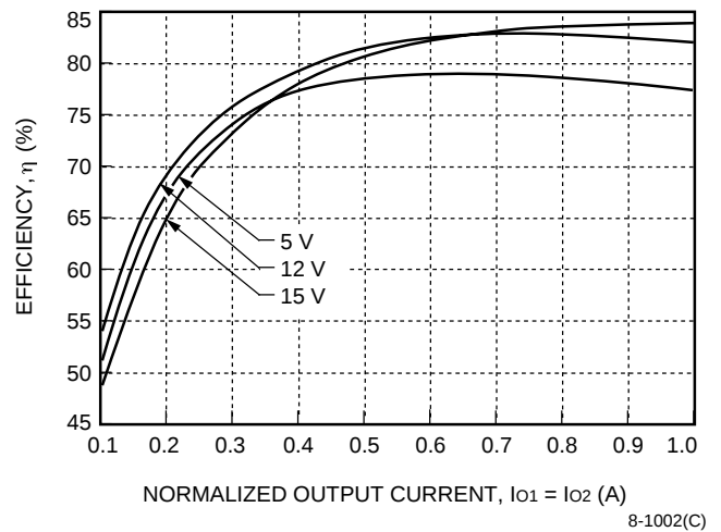
Figure 3. DC025 Dual-Output-Series Efficiency vs. Normalized Output Currents at V_i = 28\text{ V} and T_c = 25^\circ\text{C}
