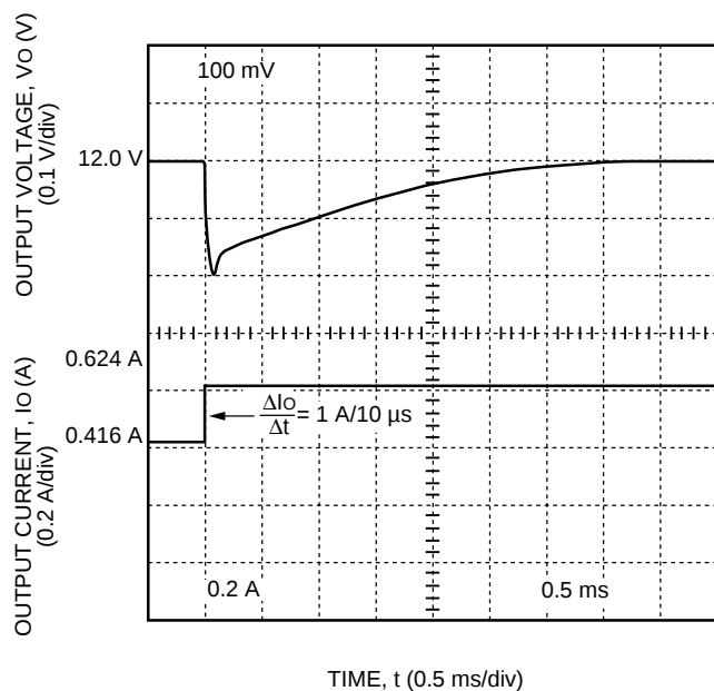
Figure 8. DC025 Dual-Output-Series Typical 12 V Output Voltage Response to a Step Load Change from 50% to 75% of I_{o,max} at V_i = V_{i,nom} and T_c = 25^\circ\text{C}
