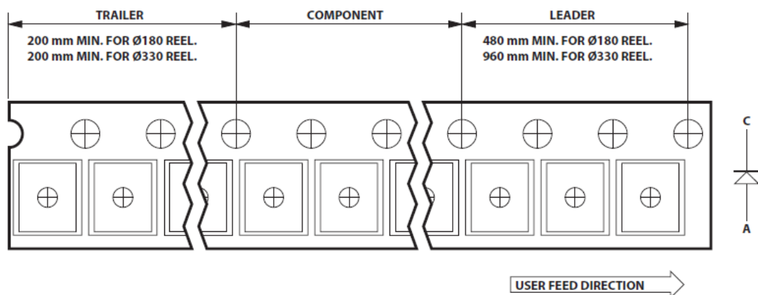
Figure 9. Tape leader and trailer dimensions
