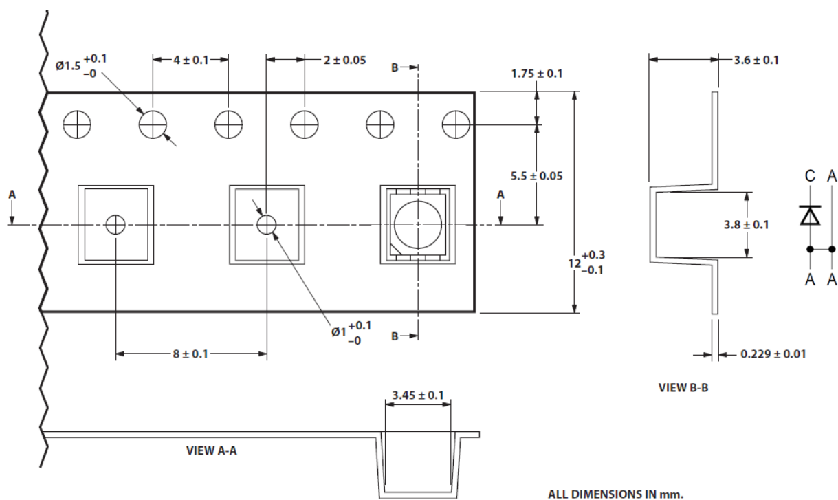
Figure 10. Tape dimensions
