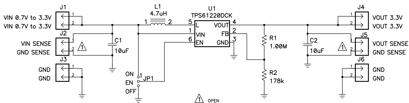
Figure 4. TPS61220EVM-319 Schematic
