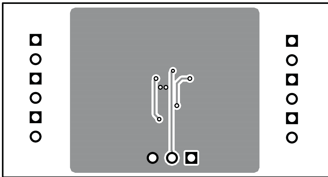
Figure 3. Bottom Layer
