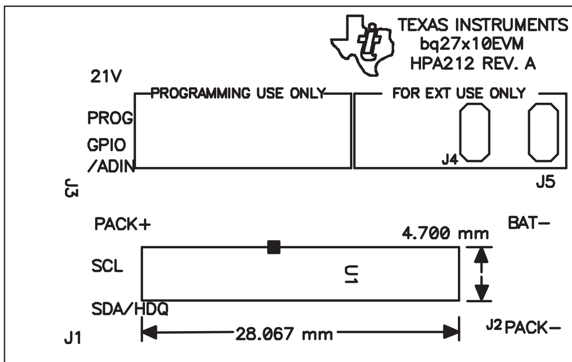
Figure 3. bq27x10EVM Silkscreen
