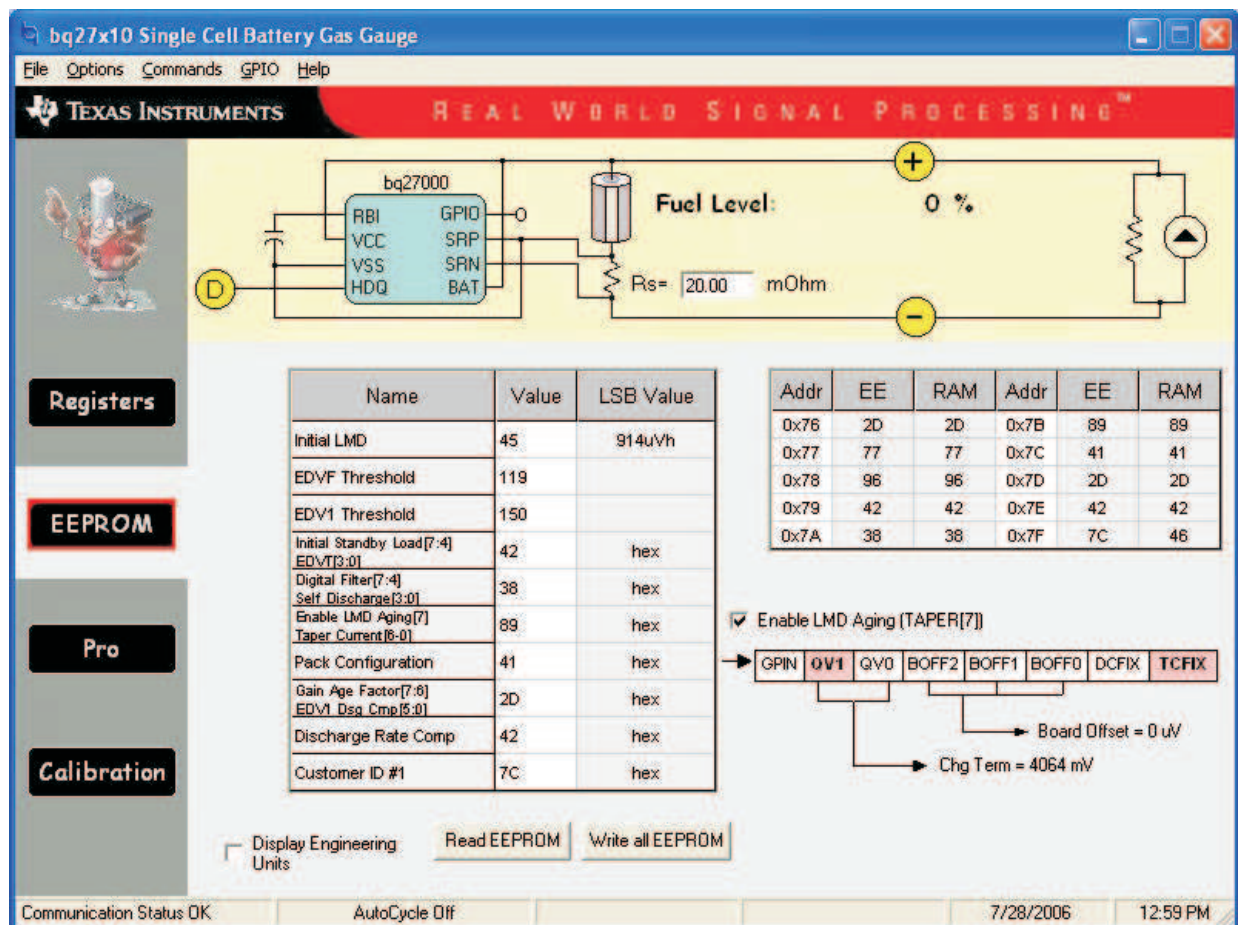
Figure 10. EEPROM Screen
