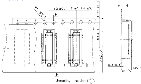
(20, 30, 40 contacts)
