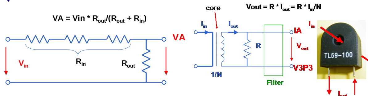
Figure 27: Resistive Voltage Divider (left), Current Transformer (right)
