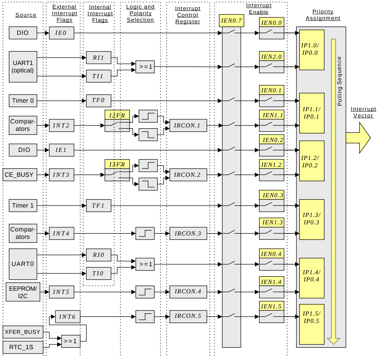
Figure 7: Interrupt Structure
