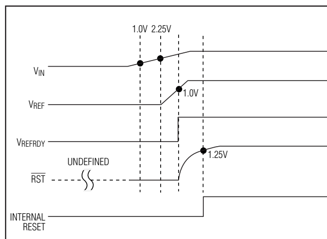
Figure 9. Reset Function Sequence
