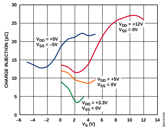
Figure 18. Charge Injection vs. Source Voltage
