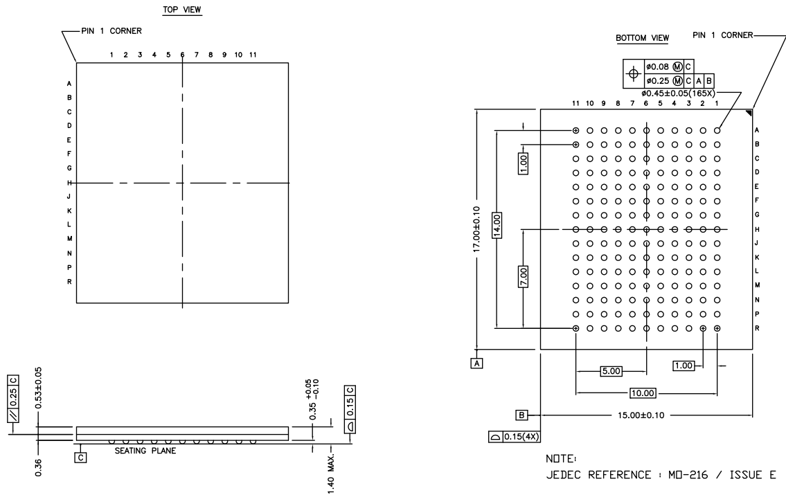
Figure 12. 165-Ball FBGA (15 x 17 x 1.4 mm), 51-85165
