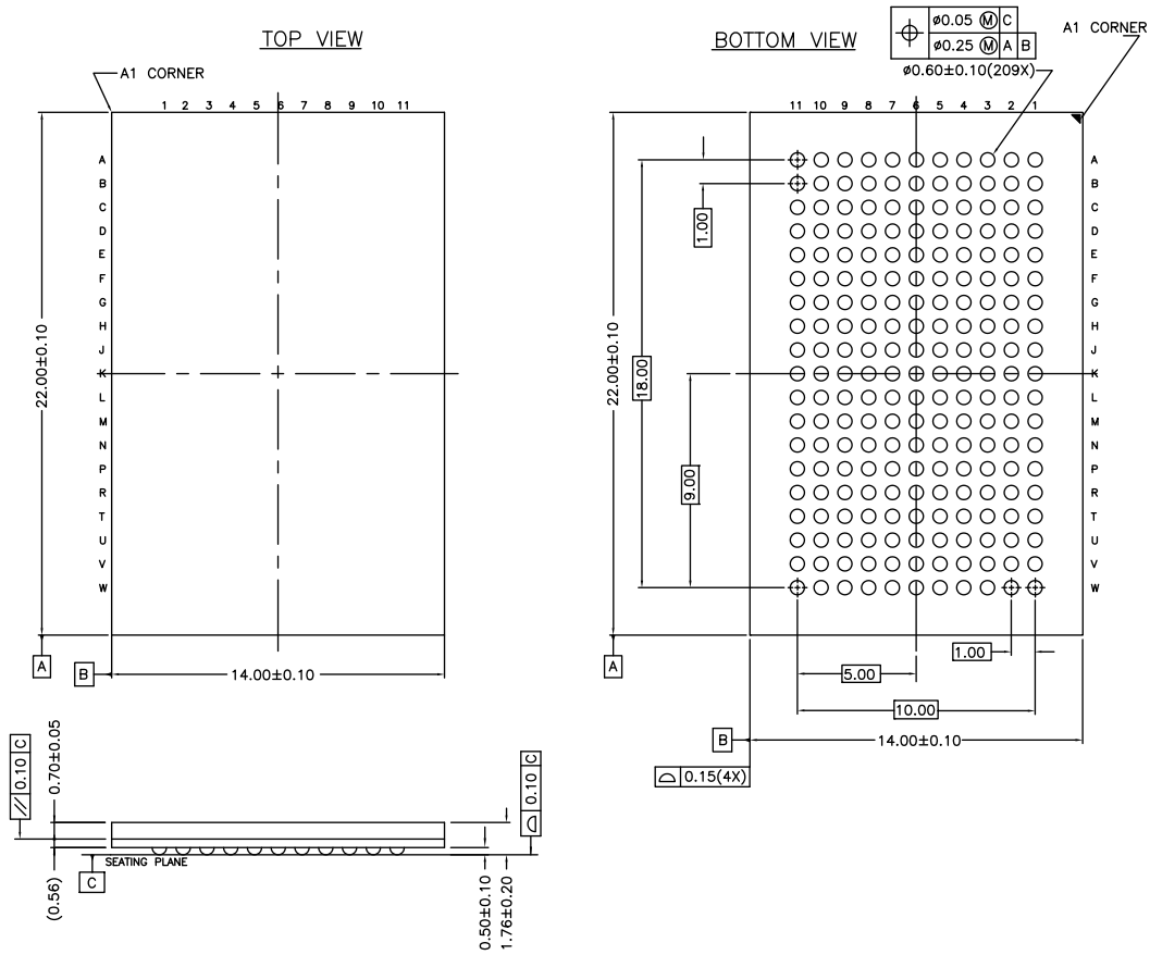
Figure 13. 209-Ball FBGA (14 x 22 x 1.76 mm), 51-85167
