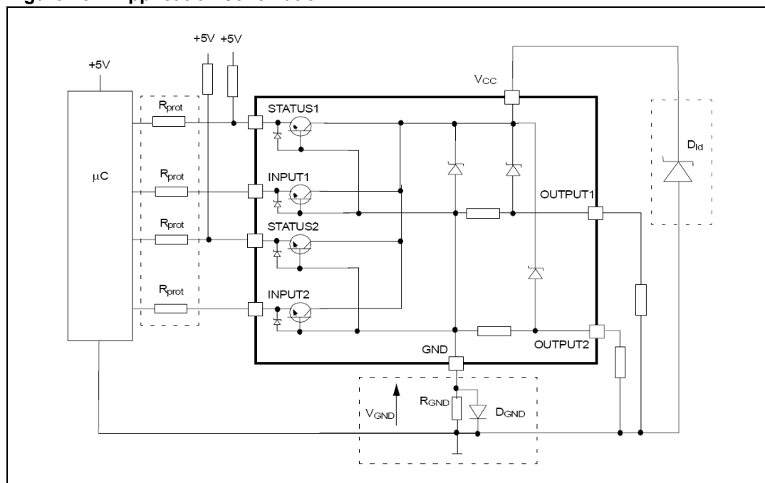
Figure 26. Application schematic
