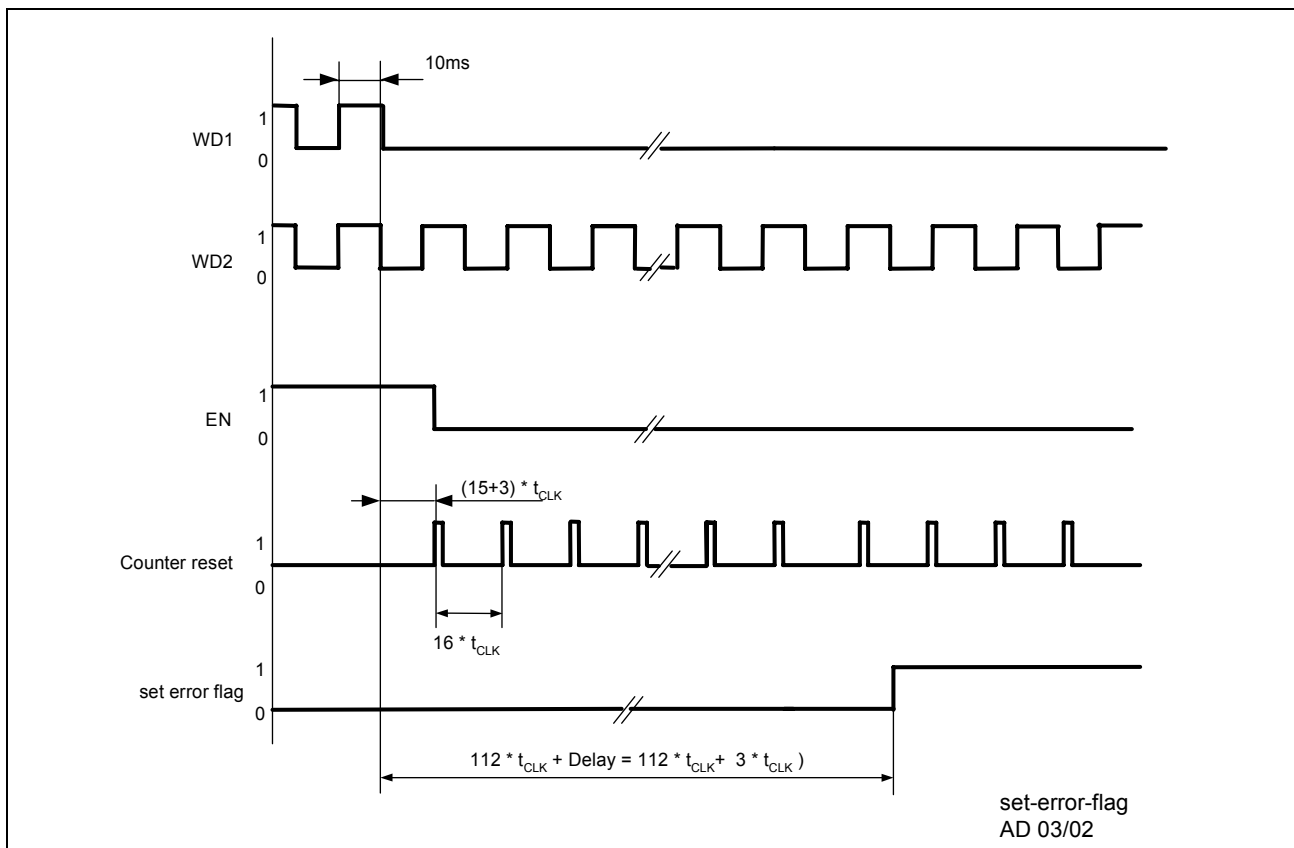
Figure 10 Missing watchdog signals for more than 120 \cdot t_{CLK} (typ. 120ms) sets the failure register
