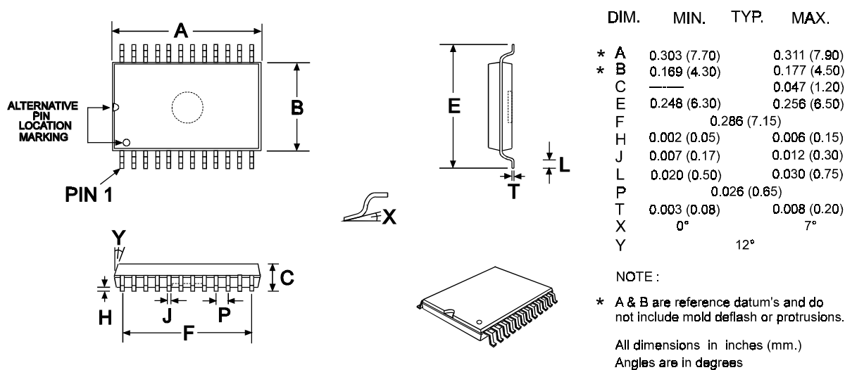
Figure 9 E2 Mechanical Outline: Order as part no. CMX469AE2
