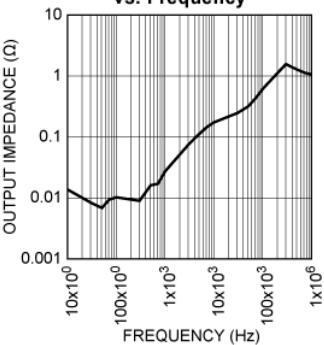
MIC2930x Output Impedance vs. Frequency
