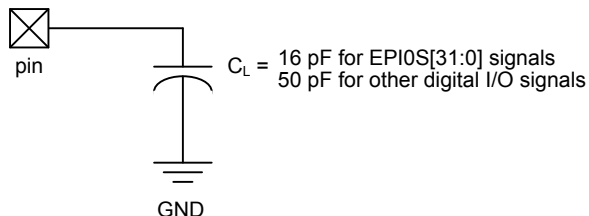
Figure 25-1. Load Conditions
