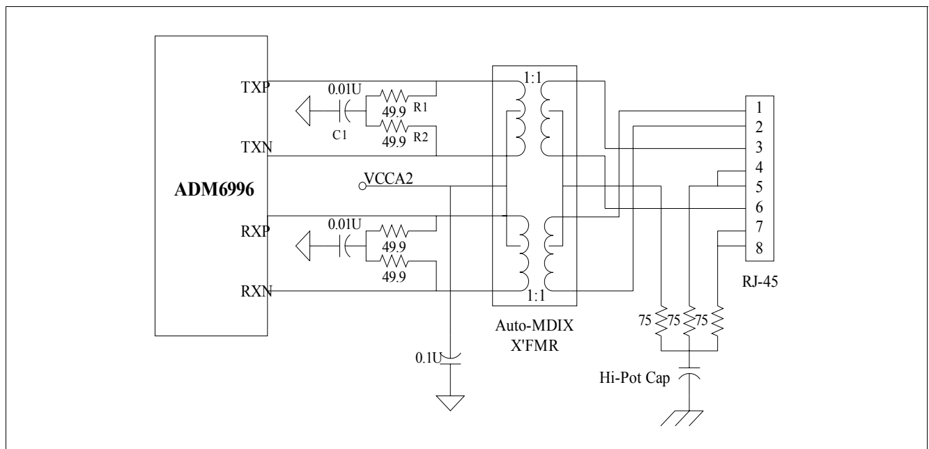
Figure 17 TP Interface
