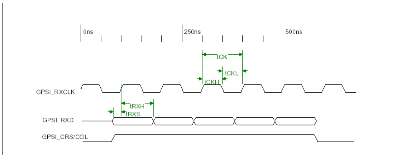
Figure 30 GPSI (7-wire) Input Timing
