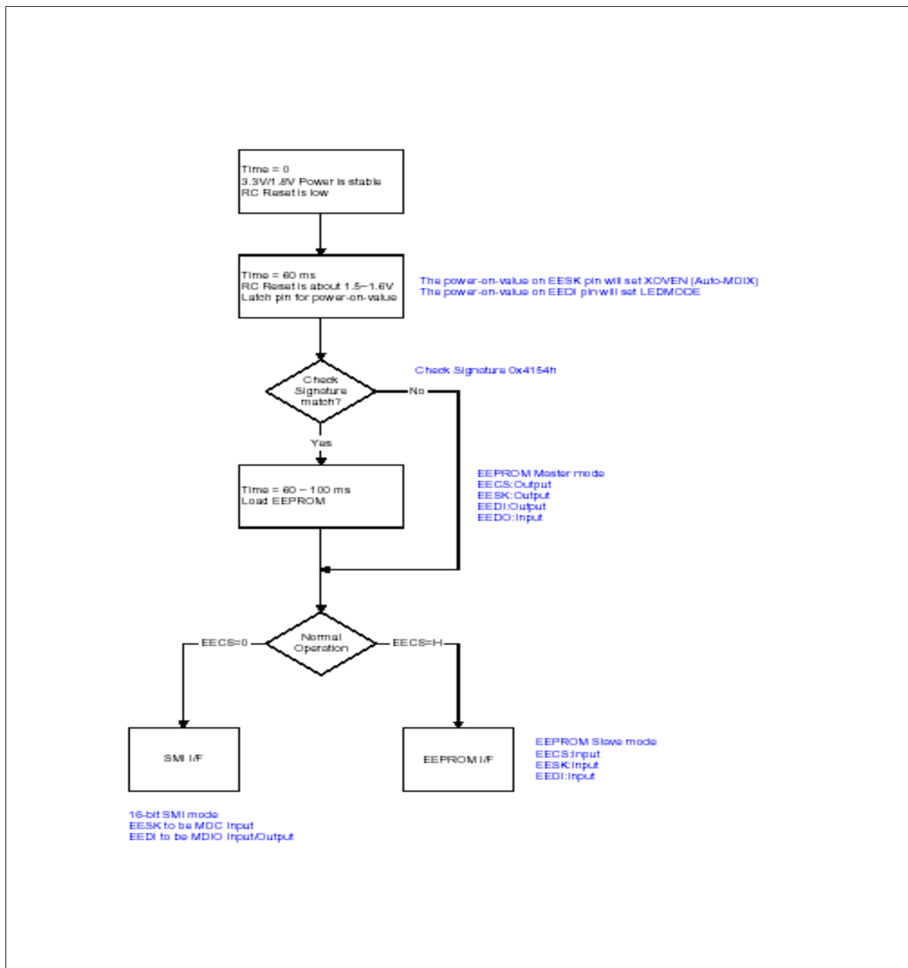
Figure 13 The Power-On-Sequence of Samurai
