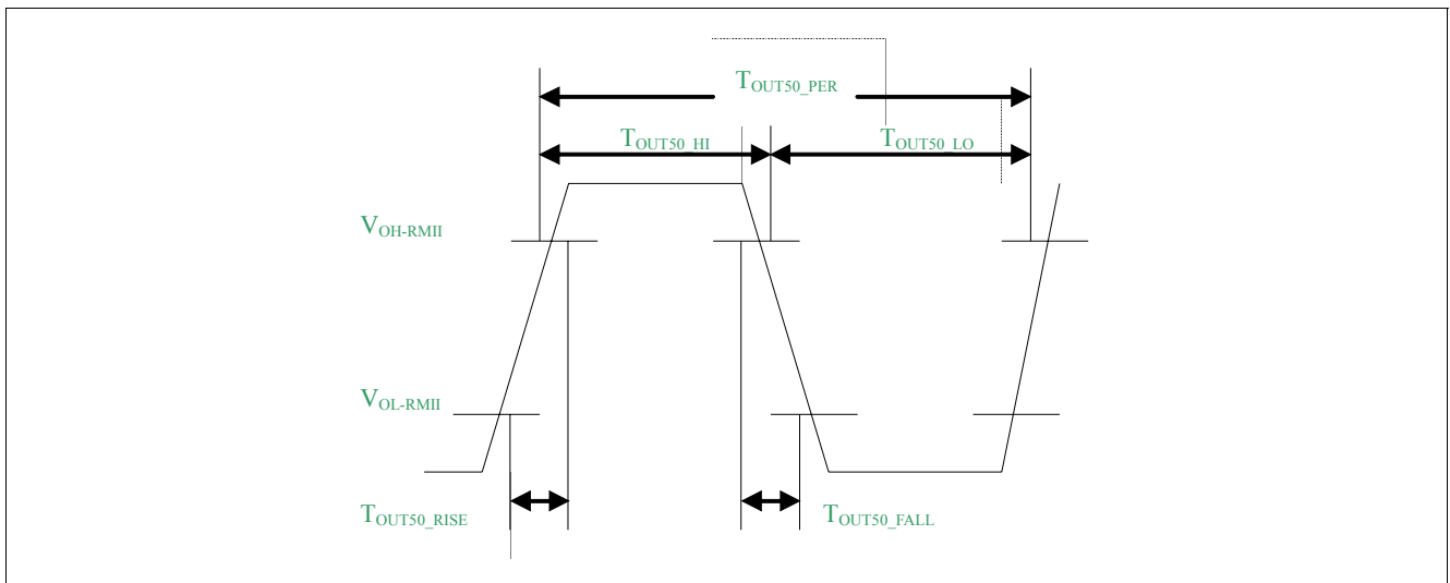
Figure 27 RMII REFCLK Output Timing
