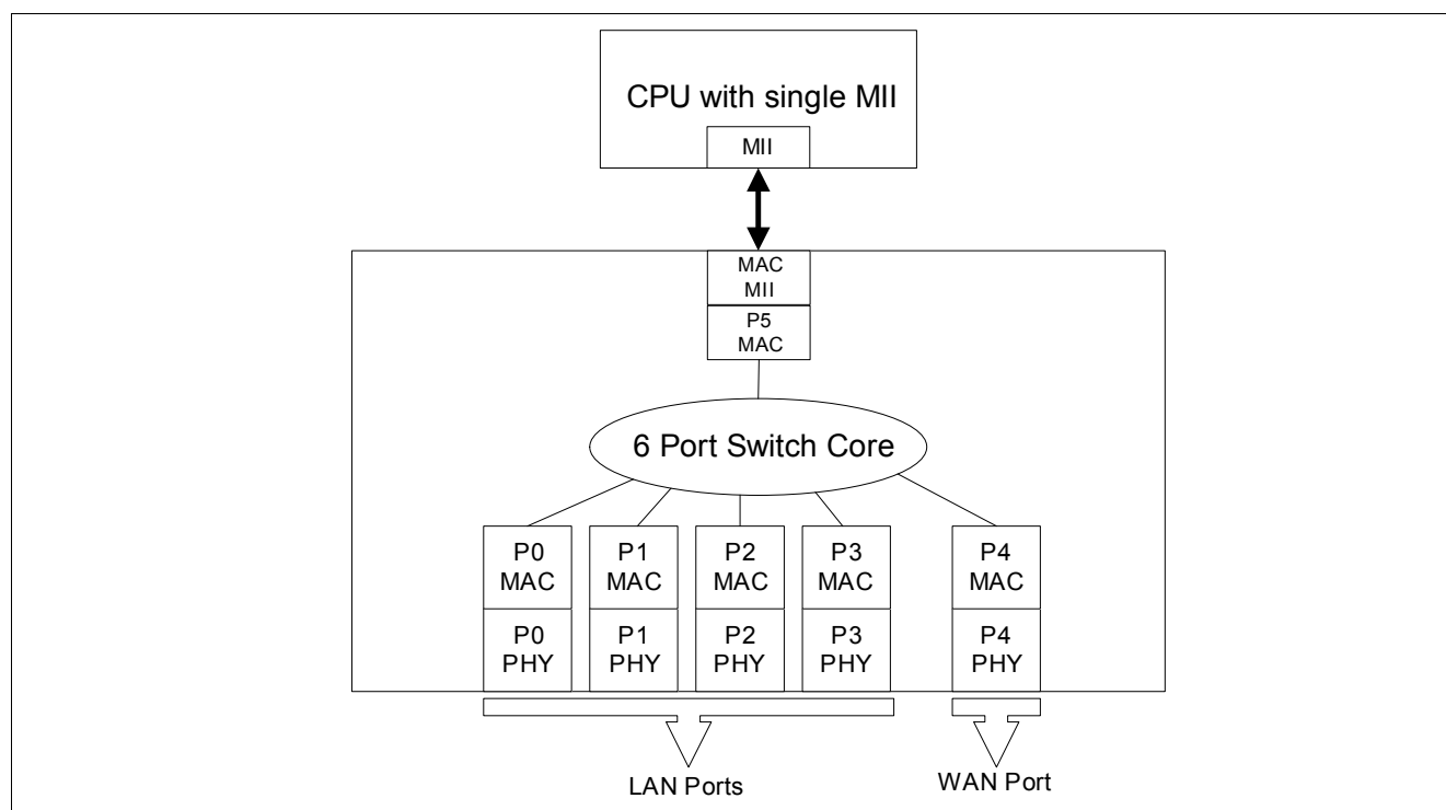
Figure 6 ADM6996M/MX to CPU with single MII Connection
