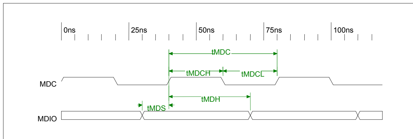
Figure 33 MDC/MDIO Timing
