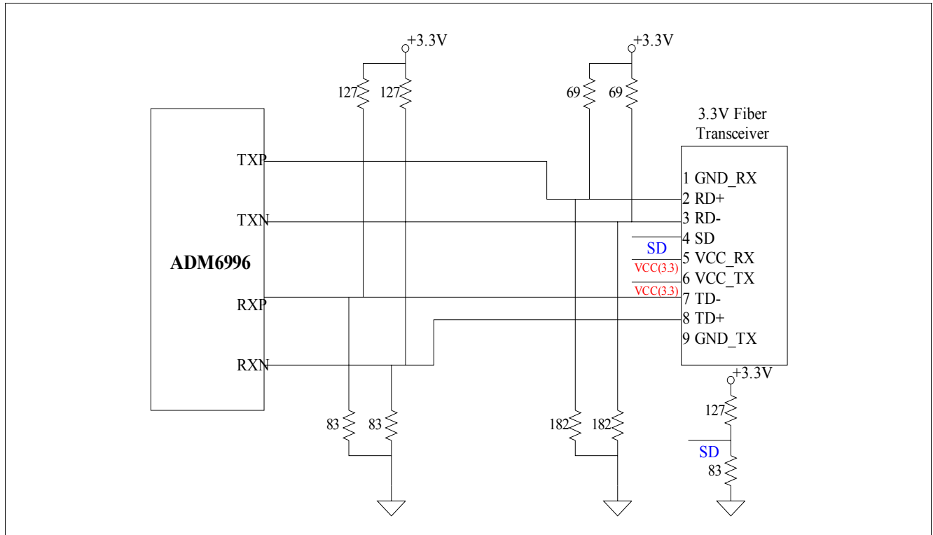
Figure 18 FX Interface
