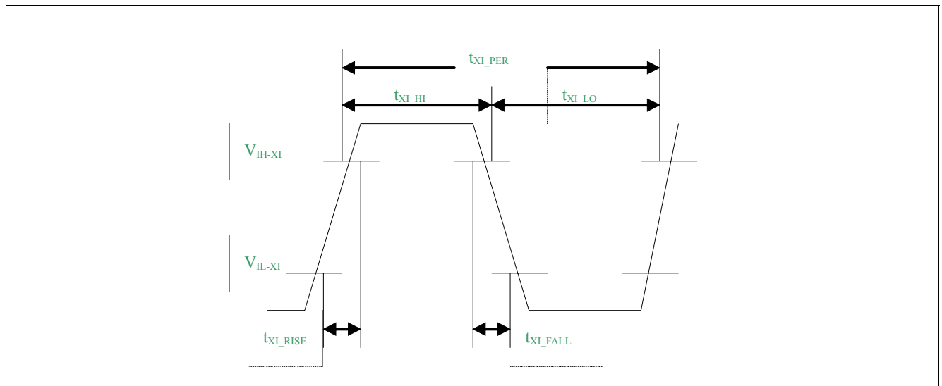
Figure 19 XTAL/OSC Timing
