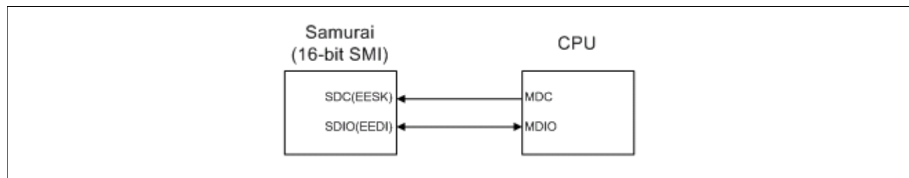
Figure 16 SMI Interface
