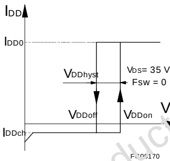
Figure 8. Shutdown Action
