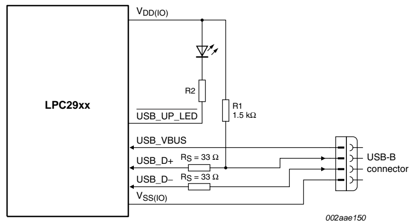
Fig 33. LPC2930 USB interface on a bus-powered device
