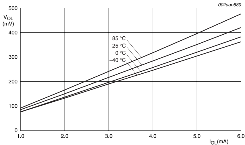
Fig 21. Typical LOW-level output voltage versus LOW-level output current
