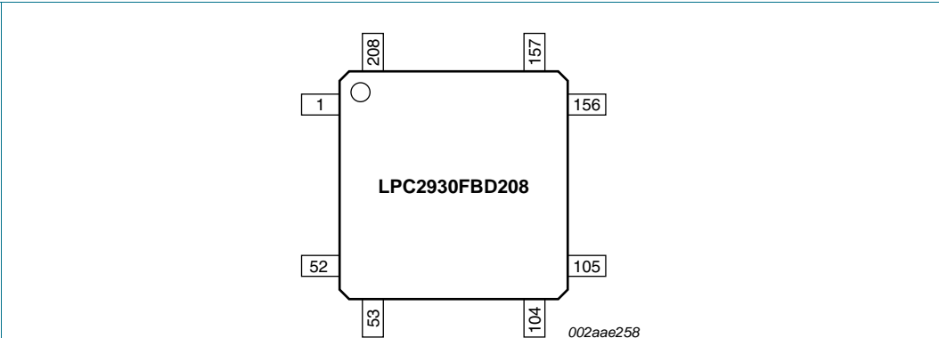
Fig 2. Pin configuration for LQFP208 package
