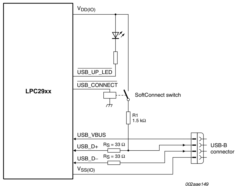
Fig 32. LPC2930 USB interface on a self-powered device
