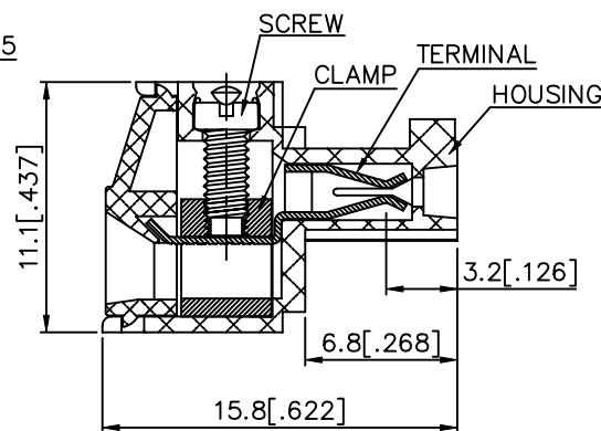
SECTION P-P
