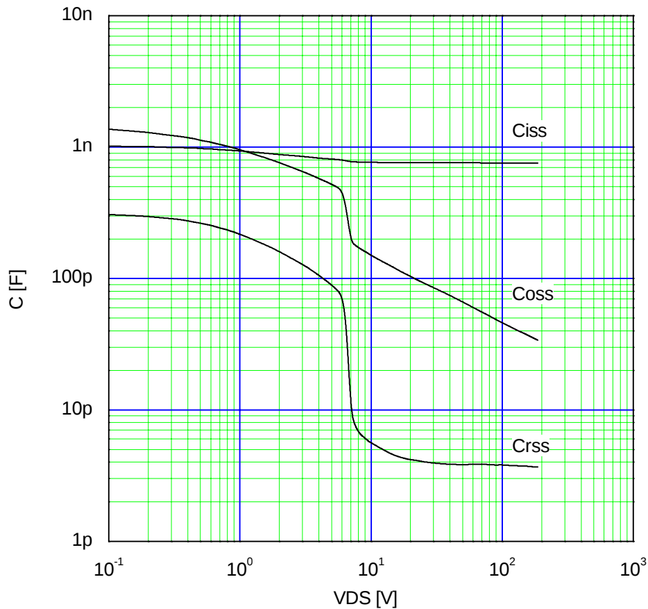
Typical Capacitance C=f(V_{DS}): V_{GS}=0V, f=1\text{MHz}
