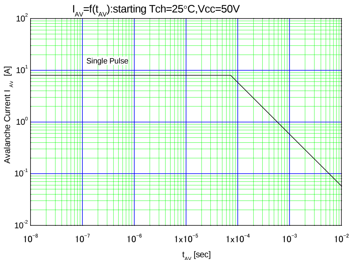
Maximum Avalanche Current Pulsewidth I_{AV}=f(t_{AV}): \text{starting Tch}=25^{\circ}C, V_{CC}=50V
