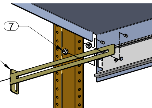
DETAIL B
