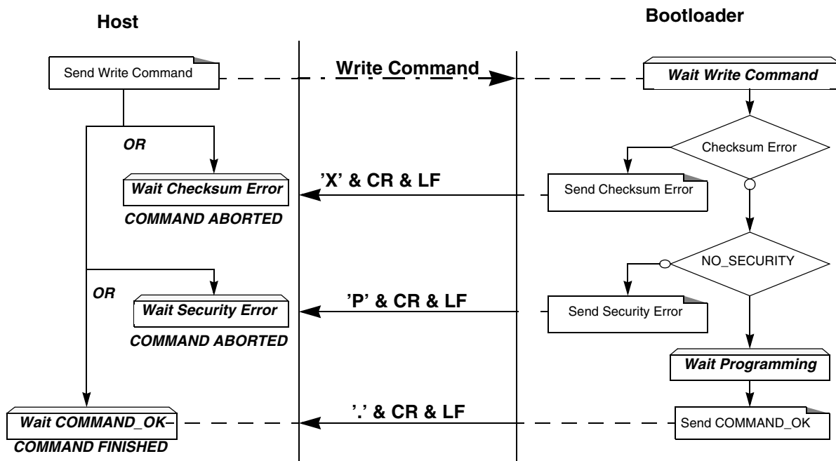
Figure 24-13. Write/Program Flow
