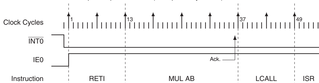
Figure 9-5. Maximum Interrupt Response Time (Compatibility Mode)
