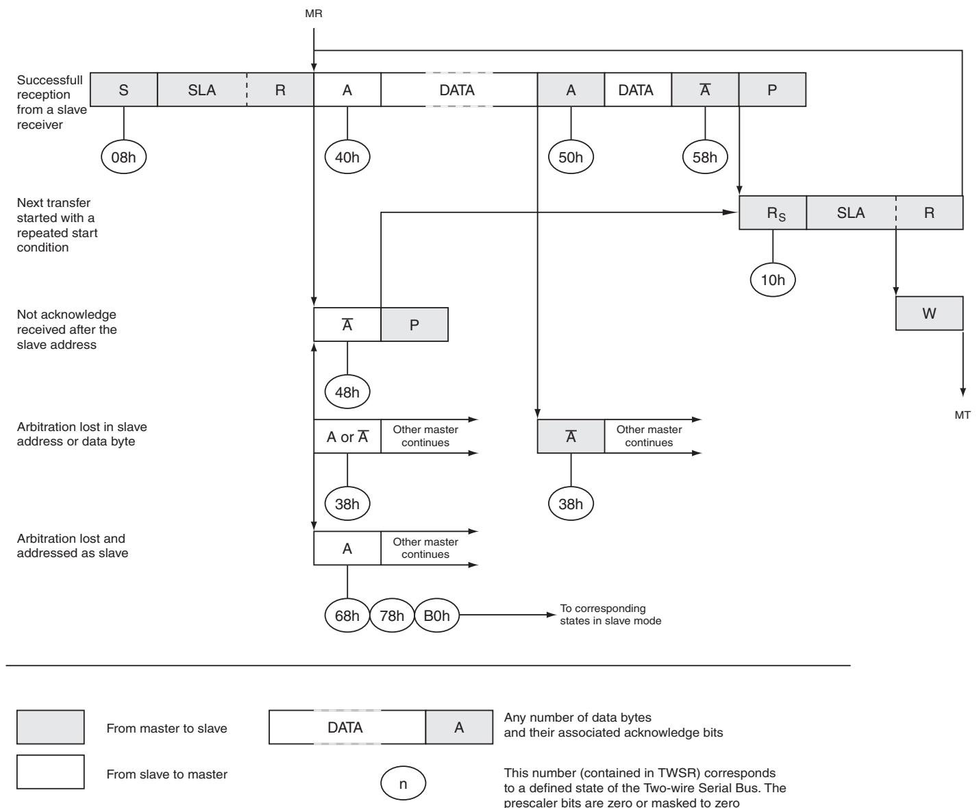
Figure 19-12. Format and States in Master Receiver Mode
