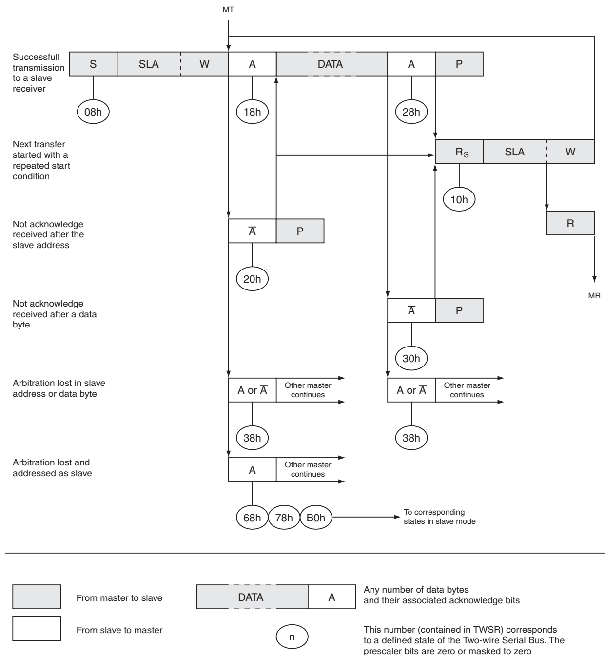
Figure 19-11. Format and States in Master Transmitter Mode
