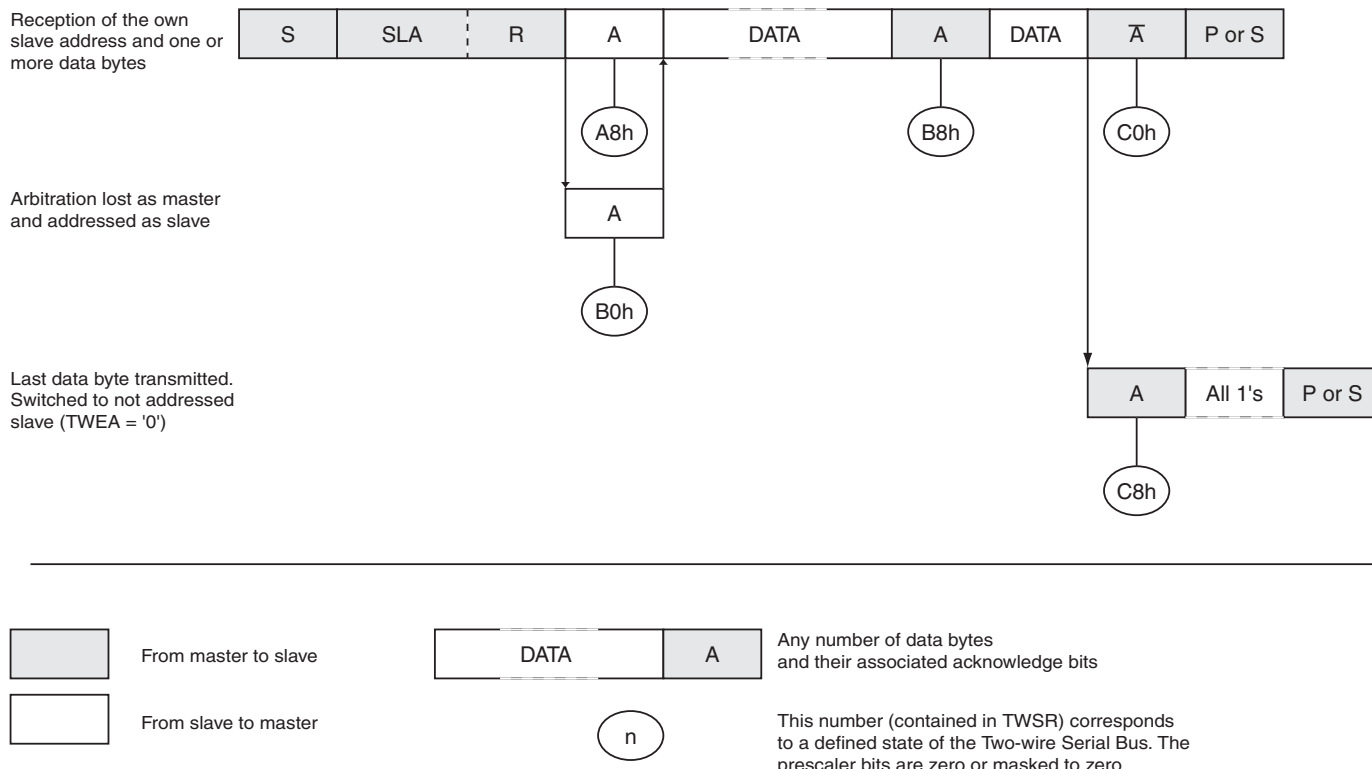
Figure 19-14. Format and States in Slave Transmitter Mode
