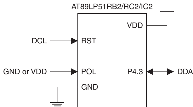
Figure 23-1. AT89LP51RB2/RC2/IC2 On-Chip Debug Connections
