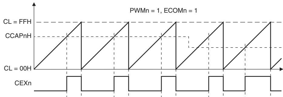
Figure 15-8. PCA PWM Waveform
