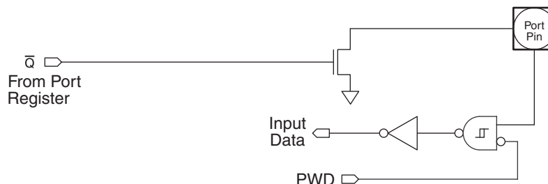
Figure 12-4. Open-Drain Output
