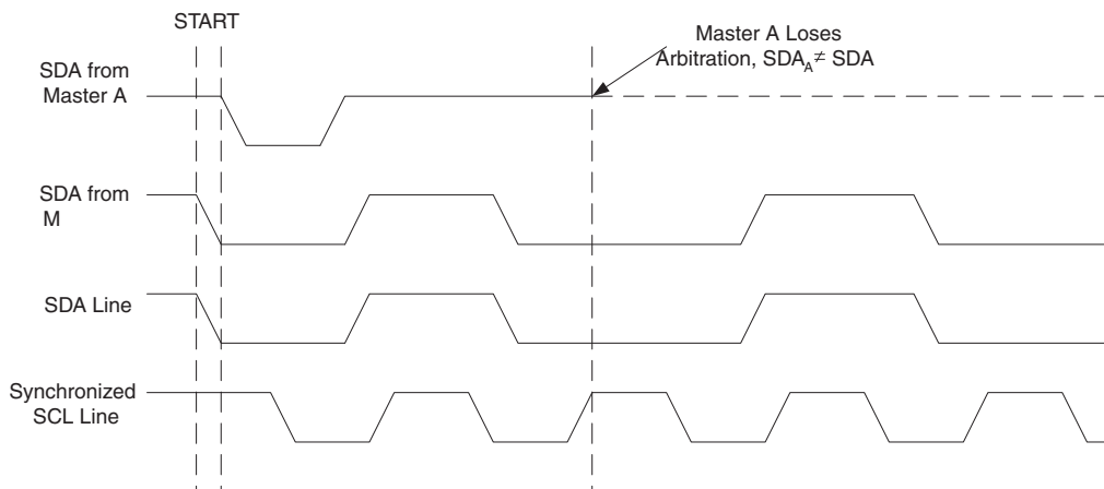
Figure 19-8. Arbitration between Two Masters
