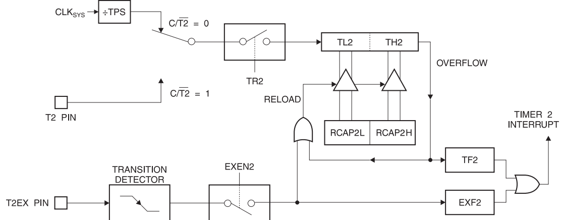
Figure 14-2. Timer 2 Diagram: Auto-Reload Mode (DCEN = 0)
