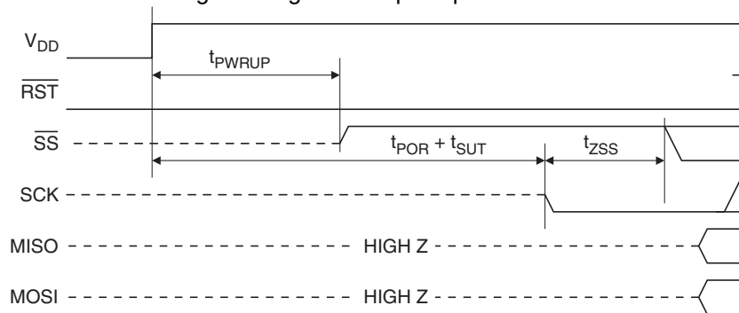
Figure 24-22. Serial Programming Power-up Sequence
