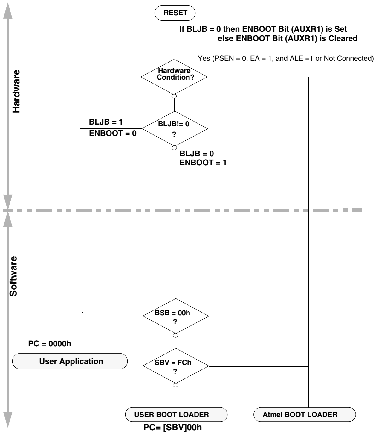
Figure 24-9. Bootloader Process
