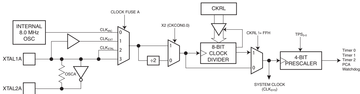
Figure 6-1. AT89LP51RB2/RC2 Clock Subsystem Diagram
