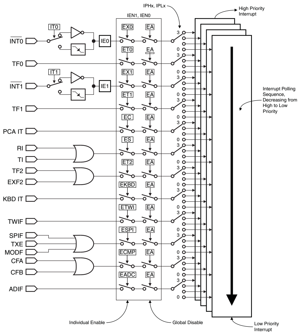
Figure 9-1. Interrupt Control Subsystem
