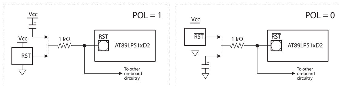
Figure 7-5. Recommended Reset Output Schematics
