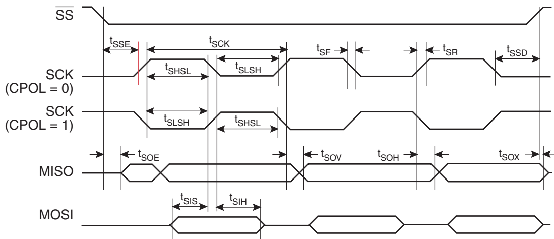
Figure 25-13. SPI Slave Timing (CPHA = 1)
