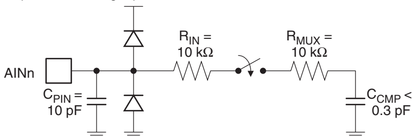
Figure 20-2. Equivalent Analog Input Model
