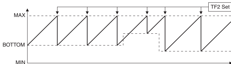
Figure 14-3. Timer 2 Waveform: Auto-Reload Mode (DCEN = 0)
