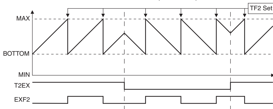
Figure 14-4. Timer 2 Waveform: Auto-Reload Mode (DCEN = 1)
