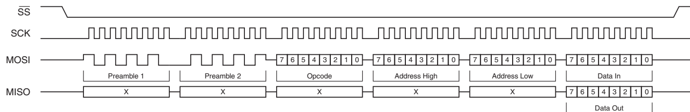
Figure 24-20. ISP Command Packet (Serial)
