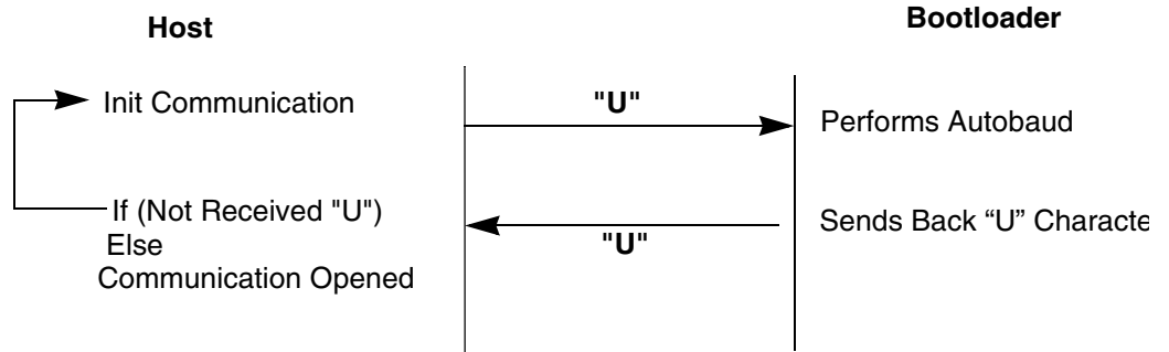
Figure 24-11. Initialization
