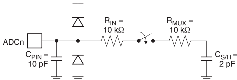
Figure 21-2. Equivalent Analog Input Model
