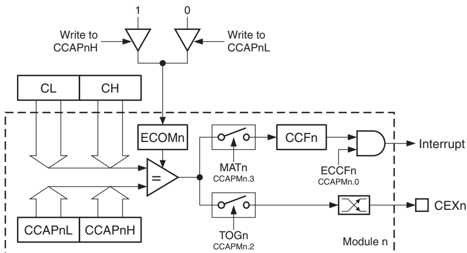
Figure 15-5. PCA High Speed Output Mode
