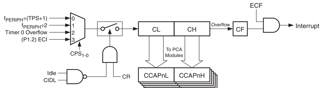
Figure 15-1. PCA Timer/Counter
