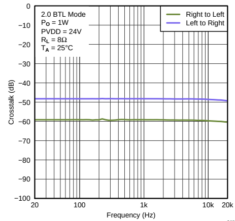
Figure 36. Crosstalk vs Frequency in 2.0 Mode
