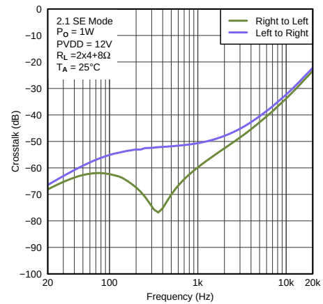
Figure 38. Crosstalk vs Frequency in 2.1 Mode
