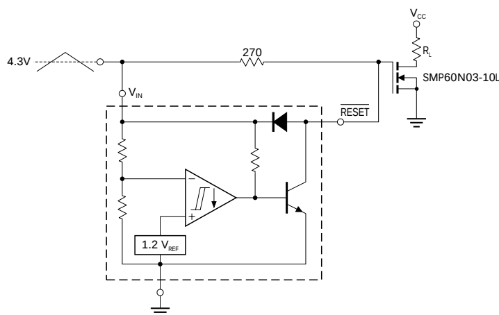
FIGURE 16. — MOSFET LOW VOLTAGE GATE DRIVE PROTECTION.
