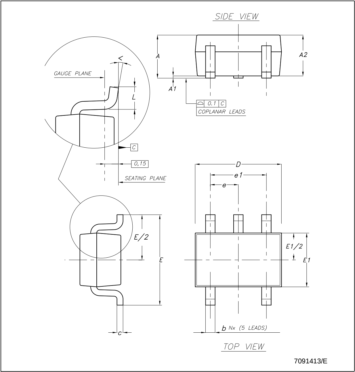
Figure 10. SOT323-5L dimensions
