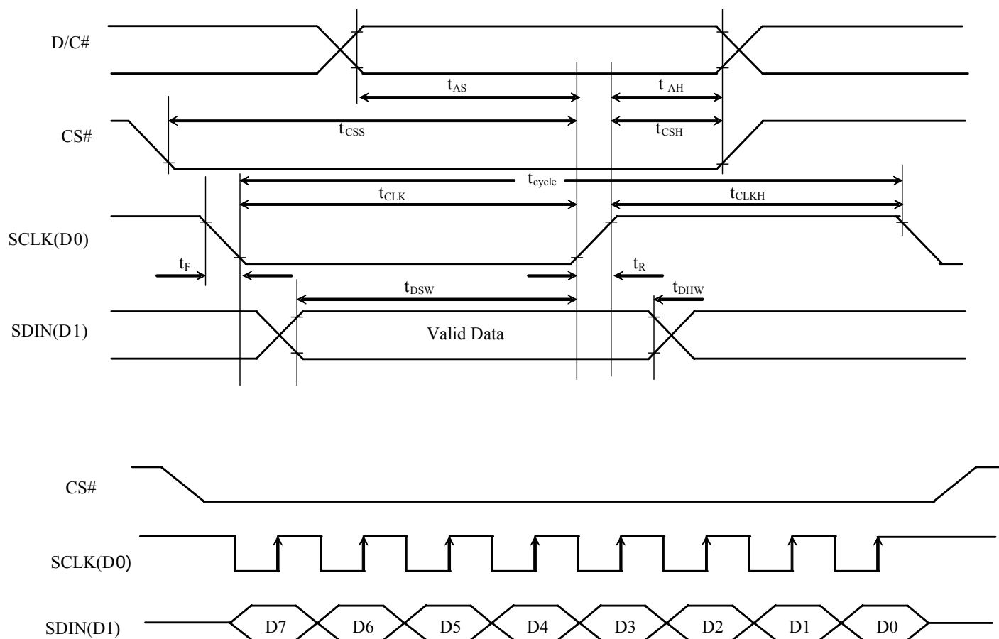
Figure 13-3 : Serial interface characteristics
