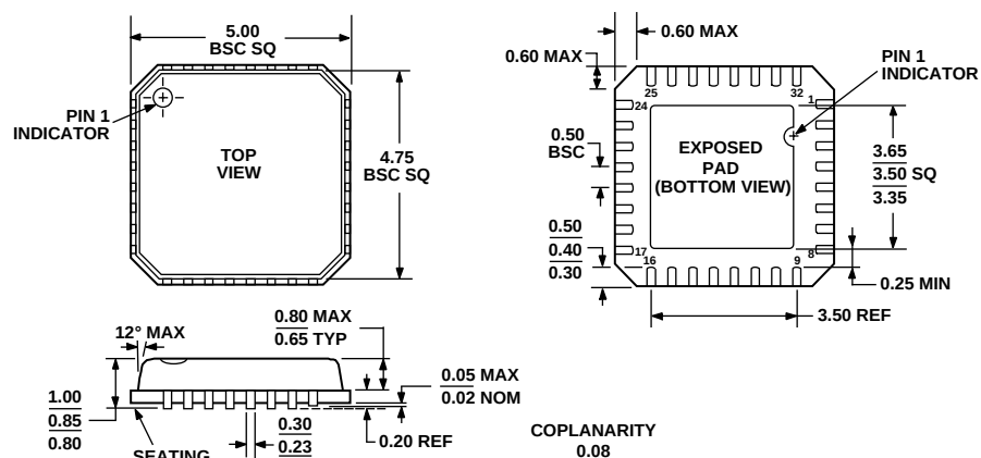
Figure 4. 32-Lead Lead Frame Chip Scale Package [LFCSP_VQ] 5 mm × 5 mm Body, Very Thin Quad (CP-32-4)
