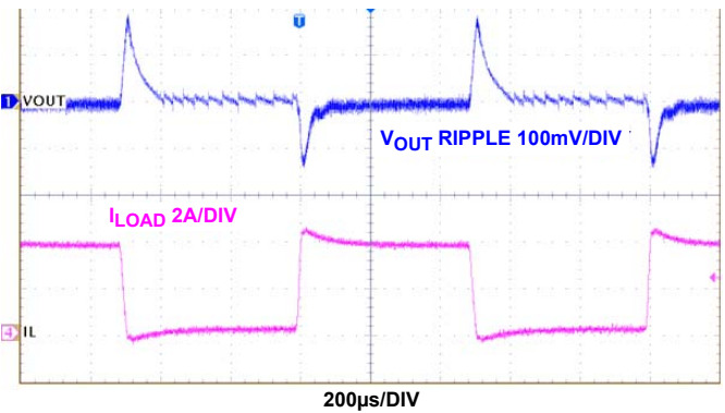
FIGURE 28. LOAD TRANSIENTS (PFM)
