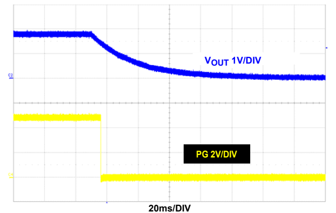
FIGURE 32. OVER-TEMPERATURE PROTECTION
