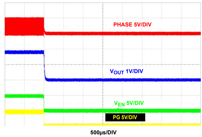
FIGURE 19. SHUTDOWN AT 4A LOAD (PWM)
