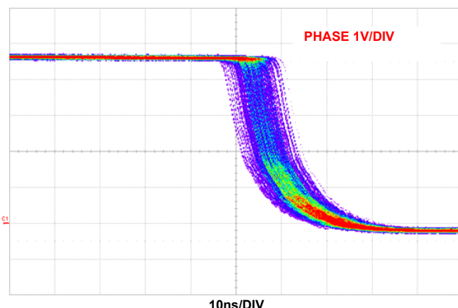
FIGURE 23. JITTER AT FULL LOAD PWM (1MHz)
