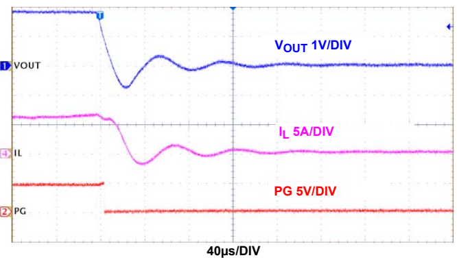
FIGURE 30. OVERCURRENT PROTECTION
