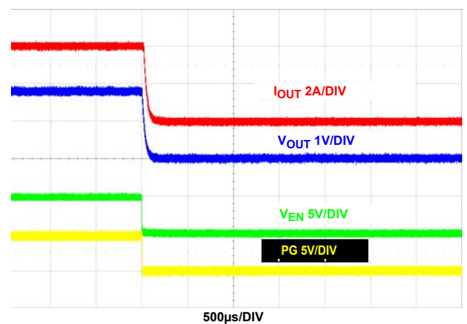
FIGURE 21. SHUTDOWN AT 4A LOAD (PFM)
