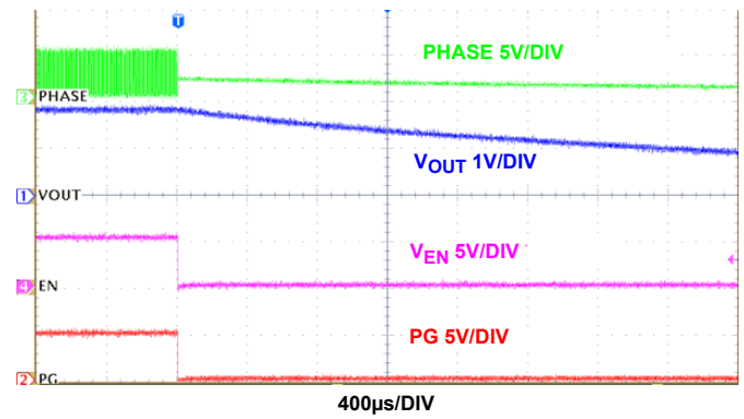
FIGURE 17. SHUTDOWN AT NO LOAD (PWM)
