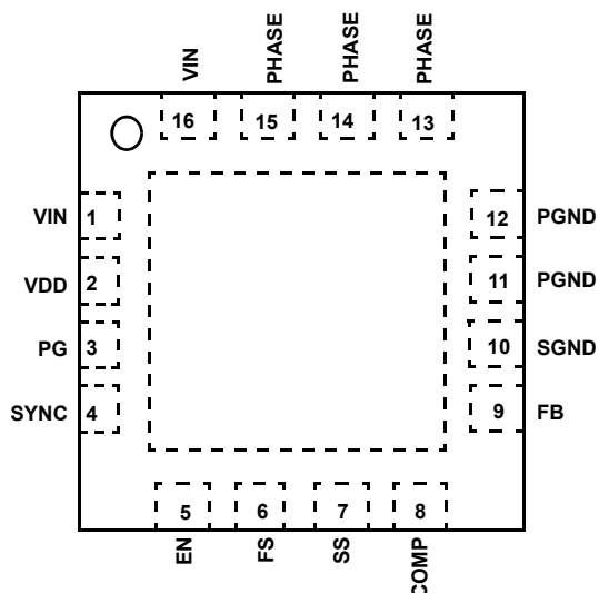
ISL78233, ISL78234 (16 LD TQFN) TOP VIEW
