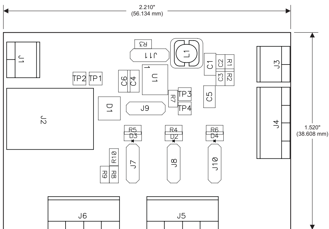
Figure 3-1. Top Assembly
