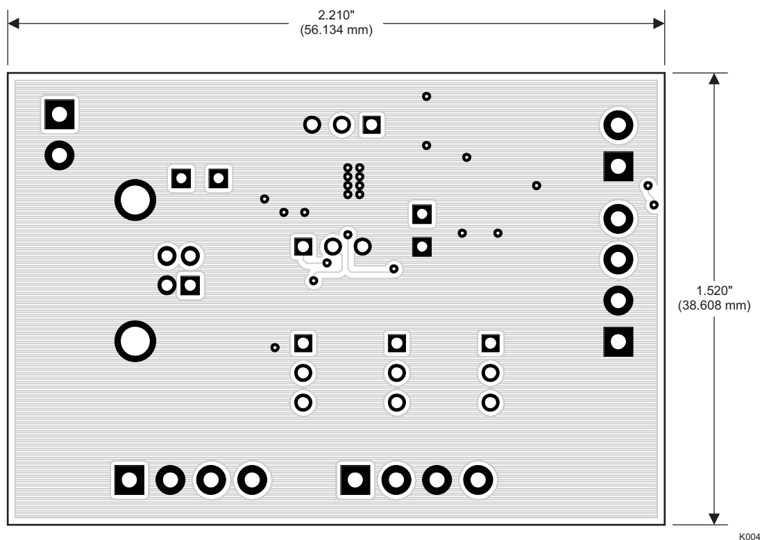
Figure 3-3. Layer 2
