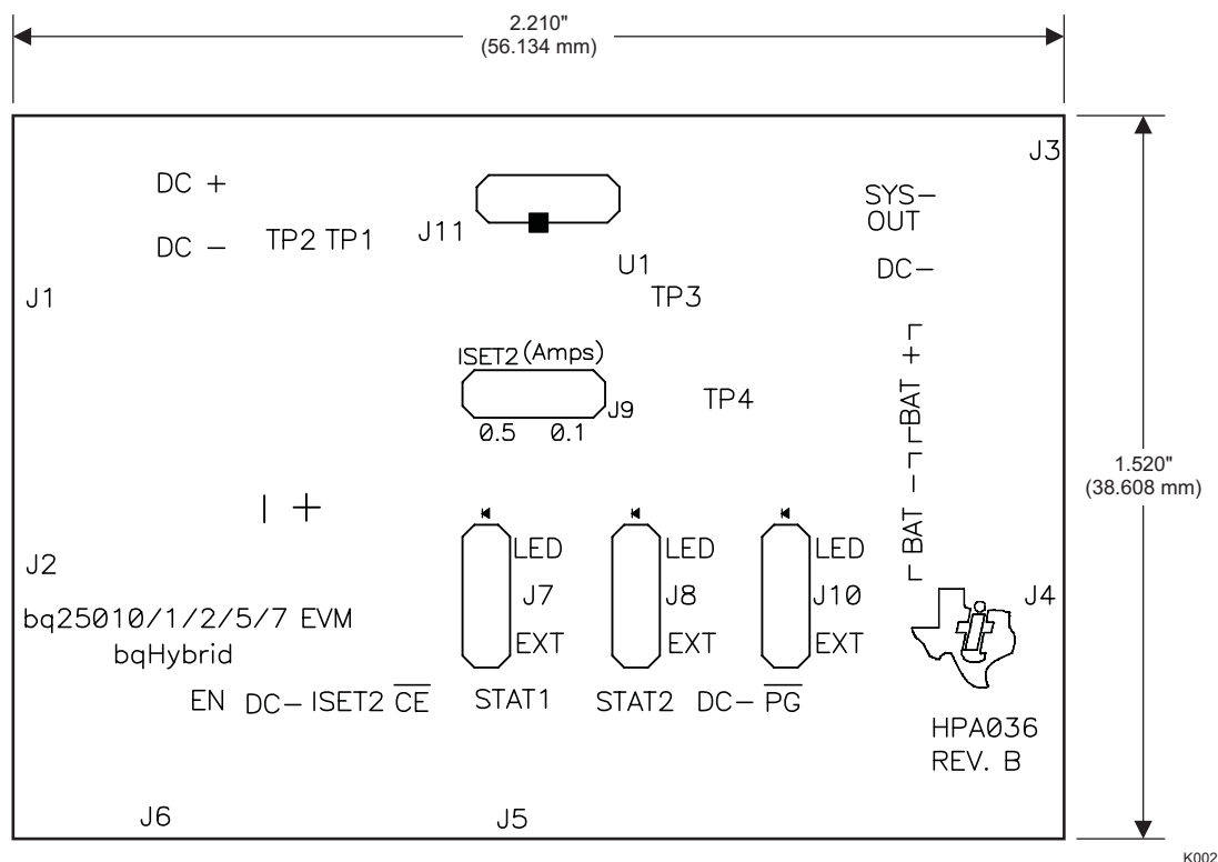
Figure 3-6. Silkscreen
