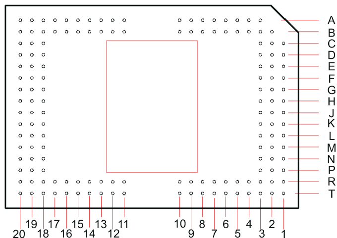
Figure 5-1. FYA Package 149-Pin CPGA Series 450 Bottom View
