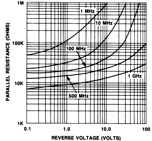
PARALLEL RESISTANCE vs FREQUENCY AND REVERSE VOLTAGE (MA4P4300 SERIES)
