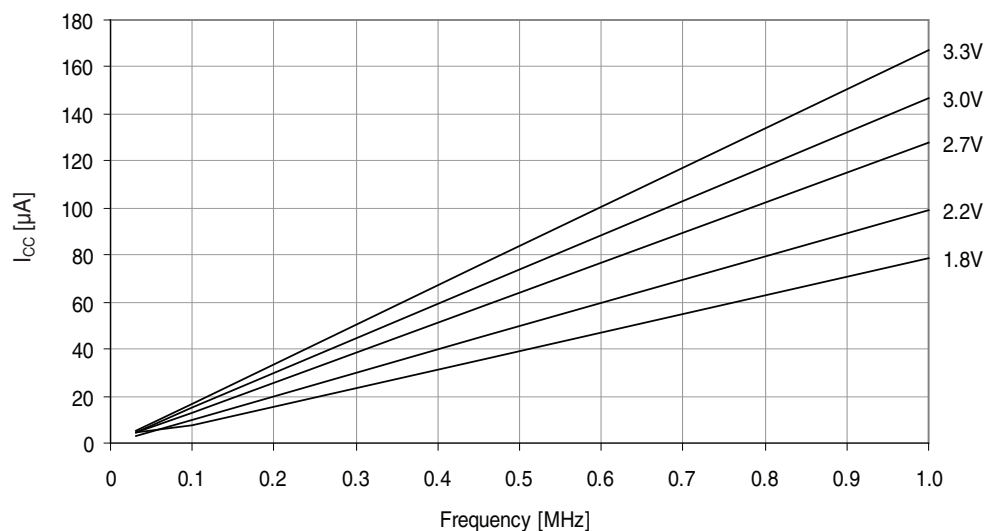
Figure 37-174. Idle mode supply current vs. frequency.
