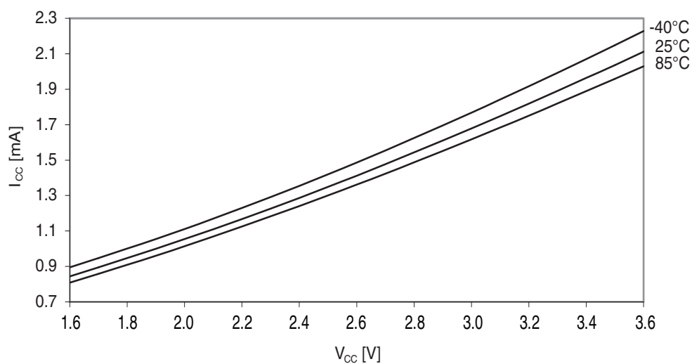
Figure 37-180. Idle mode current vs. V_{CC} .
