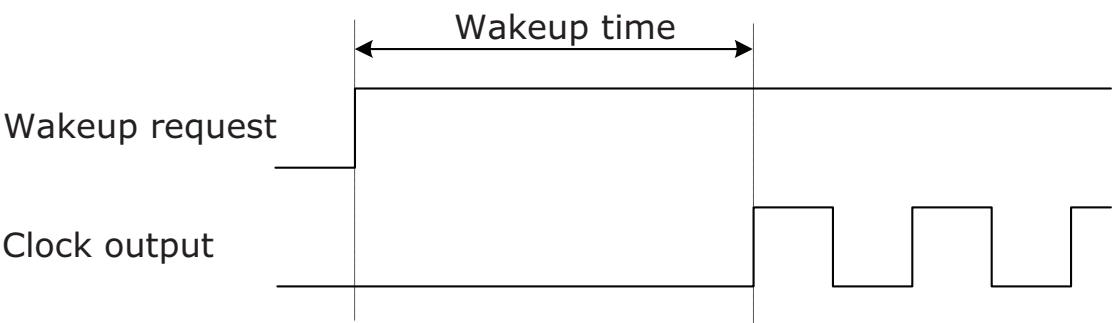
Figure 36-23.Wake-up time definition.
