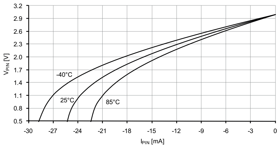
Figure 37-107. I/O pin output voltage vs. source current.
