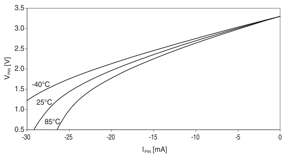
Figure 37-275. I/O pin output voltage vs. source current.
