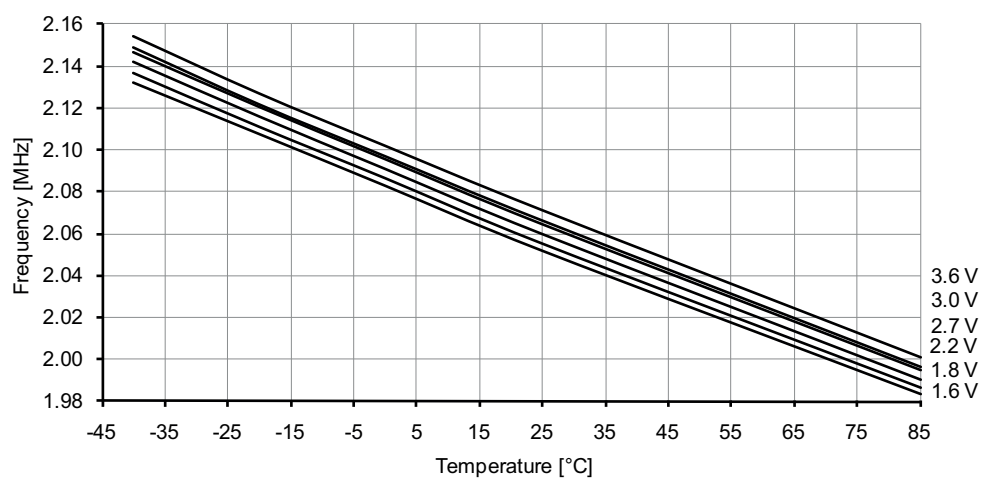
Figure 37-71. 2MHz internal oscillator frequency vs. temperature.
