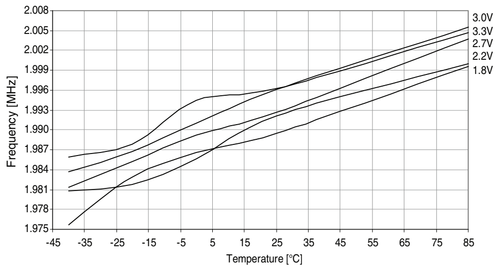
Figure 37-321. 2MHz internal oscillator frequency vs. temperature.
