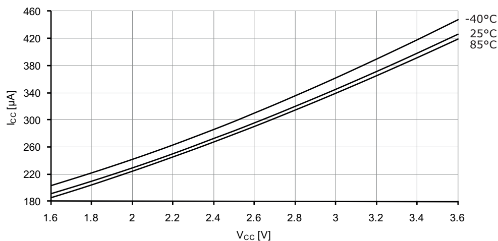
Figure 37-12. Idle mode supply current vs. V_{CC} .
