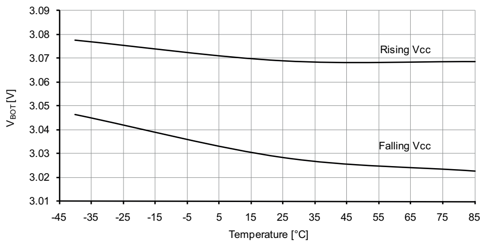
Figure 37-143. BOD thresholds vs. temperature. BOD level = 3.0V.
