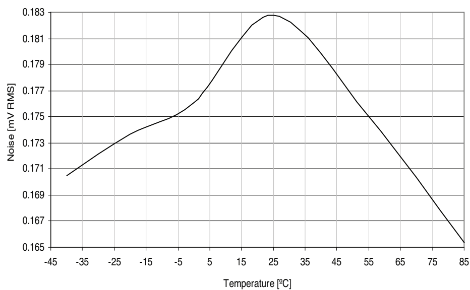
Figure 37-216. DAC noise vs. temperature.
