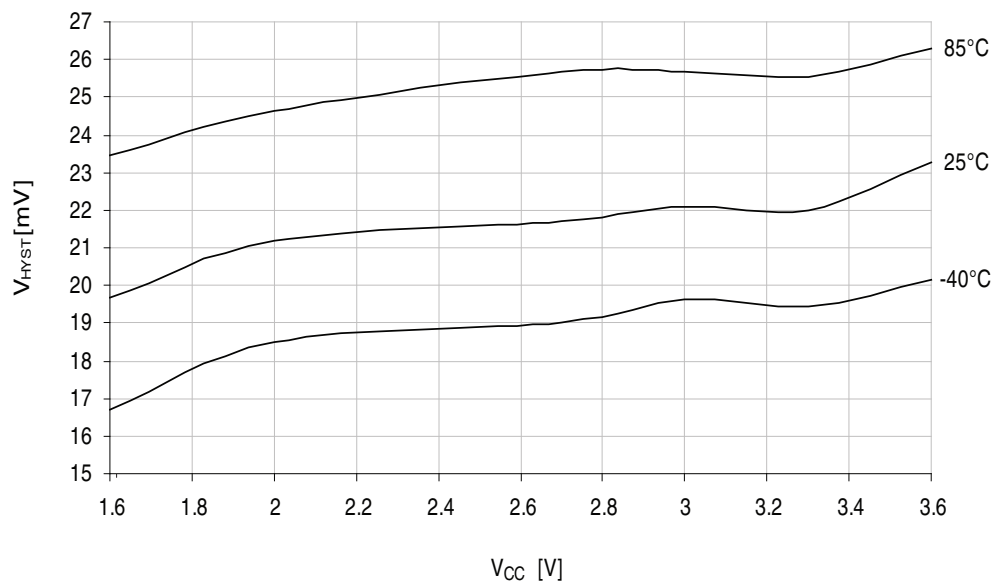
Figure 37-52. Analog comparator hysteresis vs. V_{CC} . Low power, small hysteresis.
