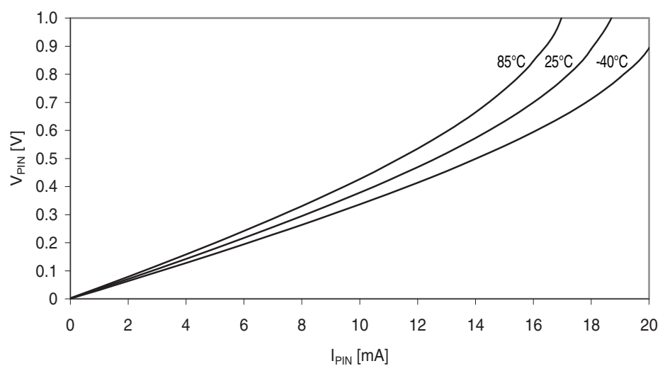
Figure 37-276. I/O pin output voltage vs. sink current.
