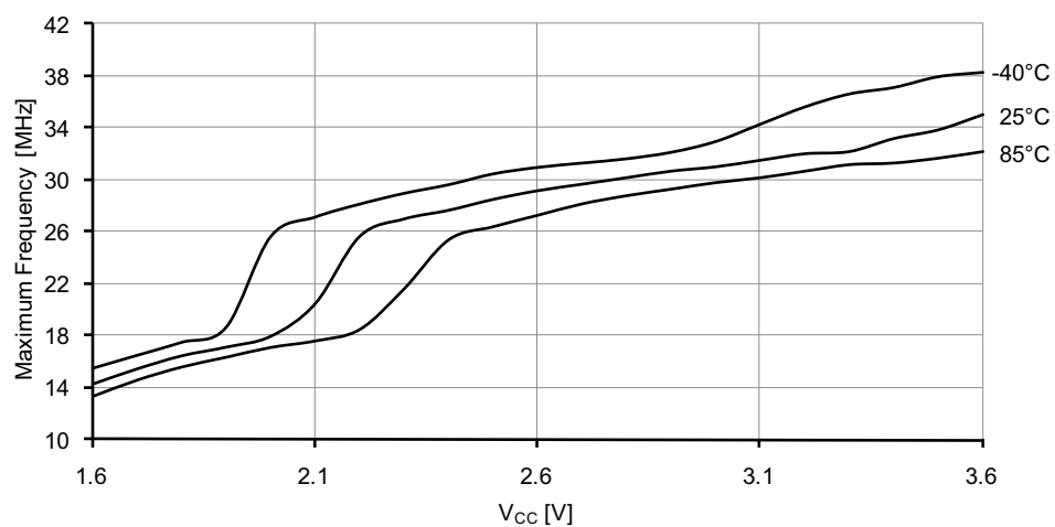
Figure 37-83. Maximum PDI frequency vs. V_{CC} .
