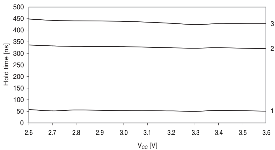
Figure 37-331. SDA hold time vs. supply voltage.
