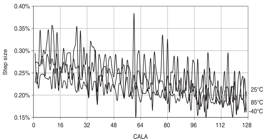
Figure 37-246. 48MHz internal oscillator CALA calibration step size.
