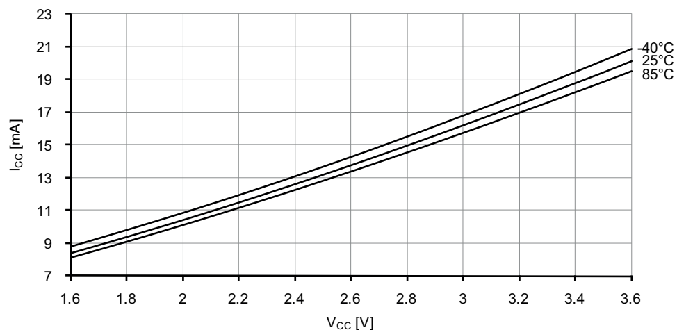
Figure 37-96. Idle mode supply current vs. V_{CC} .
