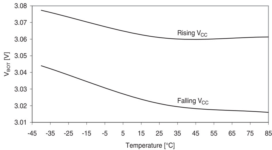
Figure 37-309. BOD thresholds vs. temperature. BOD level = 3.0V.
