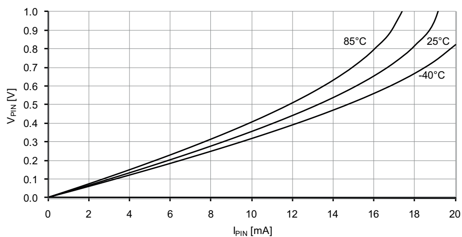
Figure 37-28. I/O pin output voltage vs. sink current.
