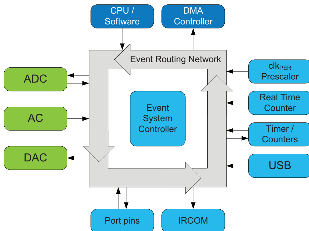
Figure 9-1. Event system overview and connected peripherals.
