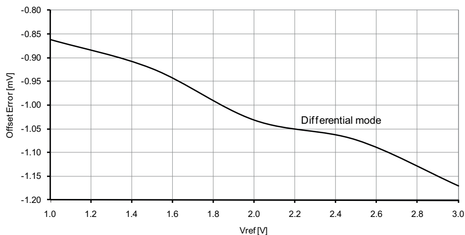
Figure 37-43. Offset error vs. V_{REF} .
