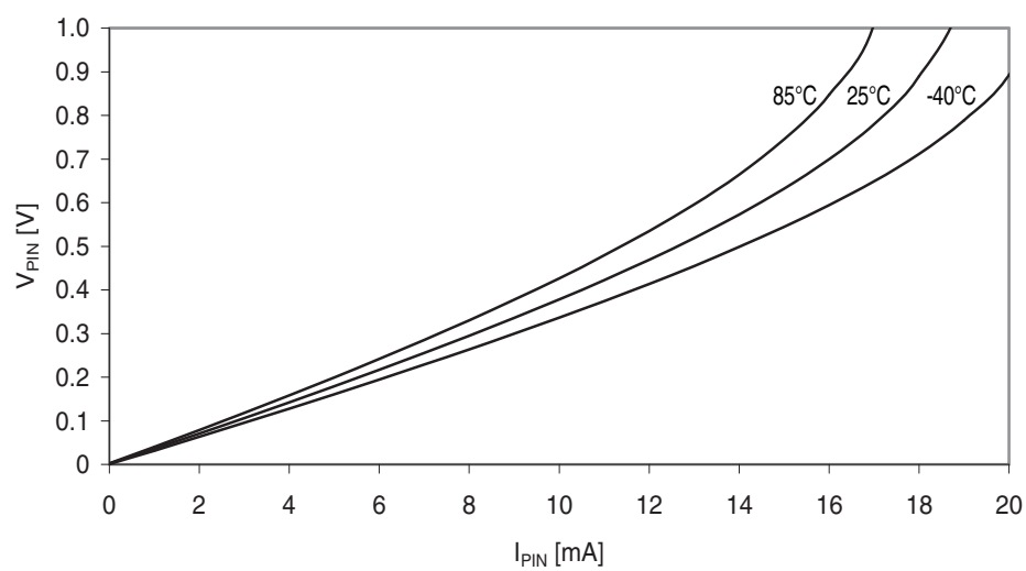
Figure 37-194. I/O pin output voltage vs. sink current.
