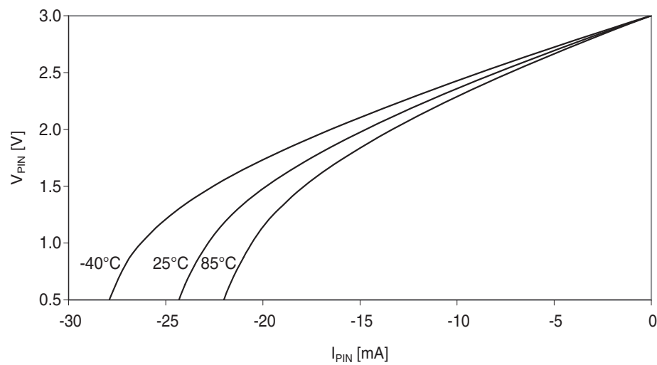
Figure 37-273. I/O pin output voltage vs. source current.
