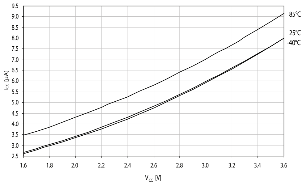
Figure 37-18. Standby supply current vs. V_{CC} .
