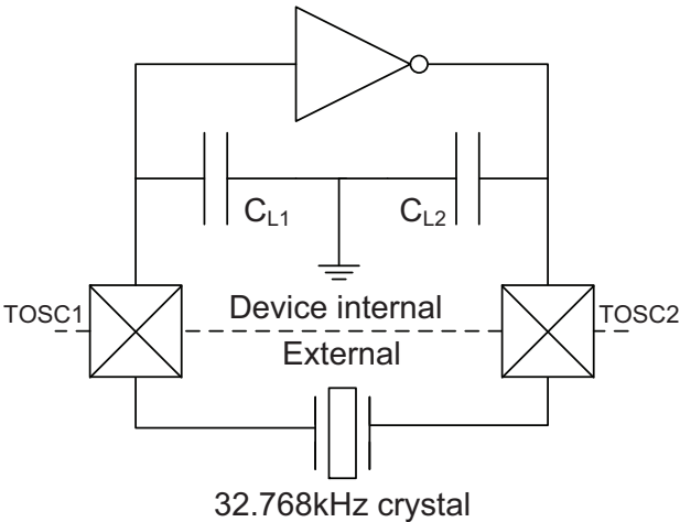
Figure 36-18.TOSC input capacitance.
