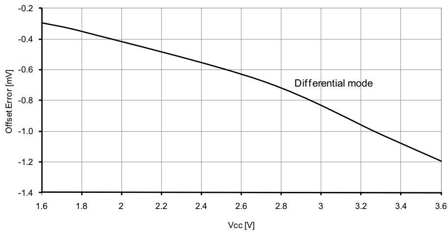
Figure 37-128. Offset error vs. V_{CC} . T = 25\text{ }^{\circ}\text{C} , V_{REF} = \text{external } 1.0\text{V} , ADC sampling speed = 500ksps.
