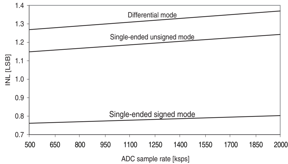
Figure 37-285. INL error vs. sample rate. T = 25\text{ }^{\circ}\text{C} , V_{CC} = 3.6\text{V} , V_{REF} = 3.0\text{V} external.
