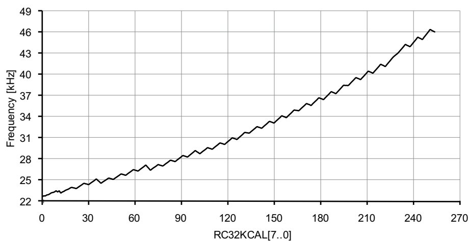
Figure 37-153. 32.768kHz internal oscillator frequency vs. calibration value.
