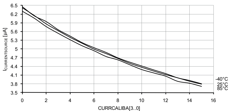
Figure 37-139. Analog comparator current source vs. calibration value.
