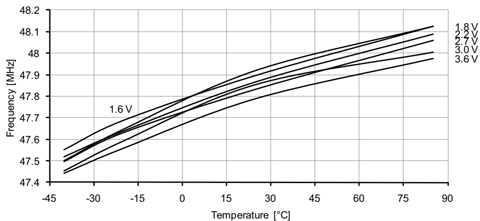
Figure 37-162. 48MHz internal oscillator frequency vs. temperature. DFLL enabled, from the 32.768kHz internal oscillator.
