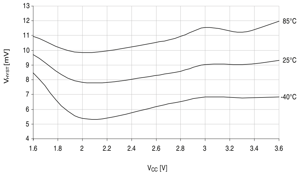
Figure 37-51. Analog comparator hysteresis vs. V_{CC} . High-speed, small hysteresis.
