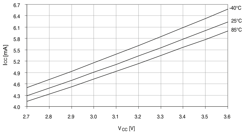
Figure 37-263. Idle mode current vs. V_{CC} .
