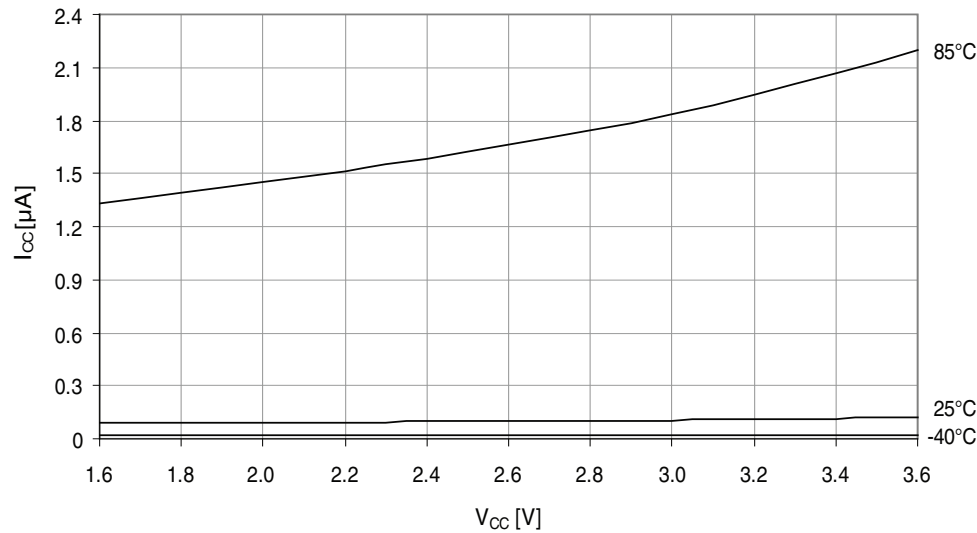
Figure 37-181. Power-down mode supply current vs. V_{CC} . All functions disabled.
