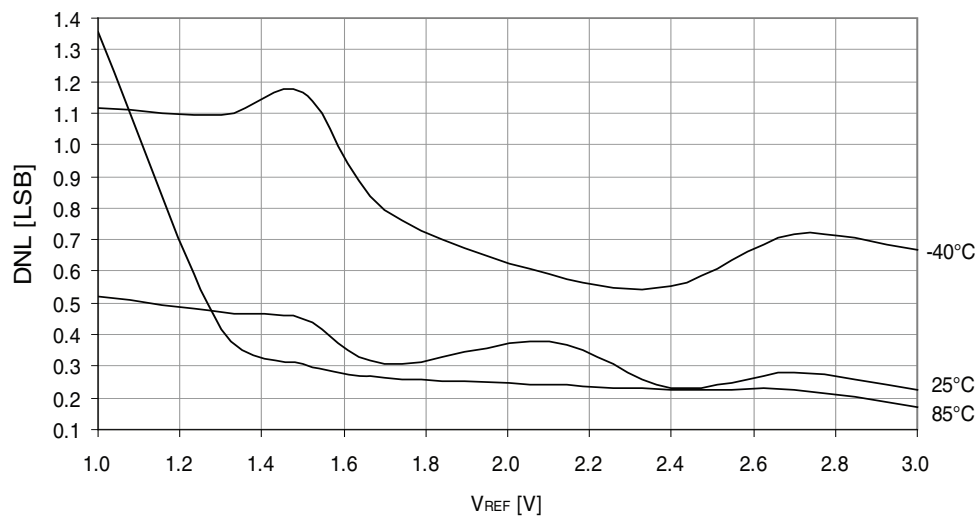
Figure 37-215. DNL error vs. V_{REF} .
