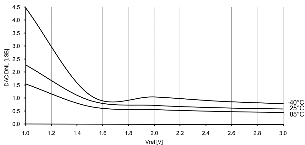
Figure 37-132. DNL error vs. V_{REF} .
