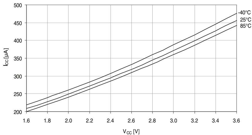
Figure 37-178. Idle mode supply current vs. V_{CC} .
