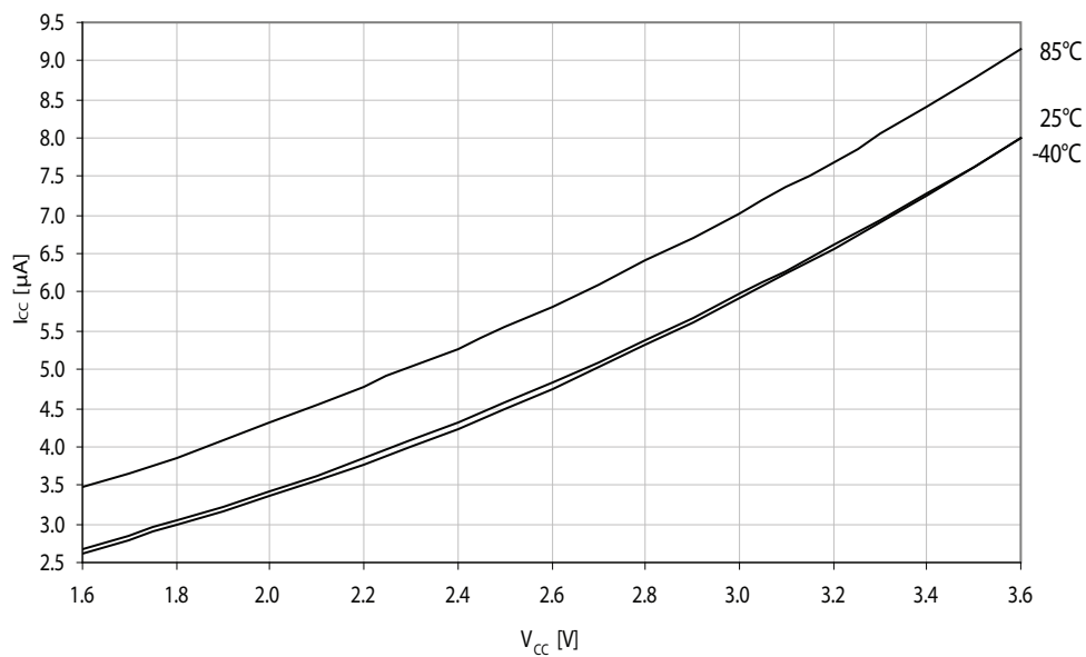
Figure 37-267. Standby supply current vs. V_{CC} .
