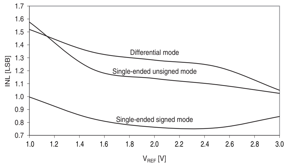
Figure 37-284. INL error vs. external V_{REF} . T = 25\text{ }^{\circ}\text{C} , V_{CC} = 3.6\text{V} , external reference.
