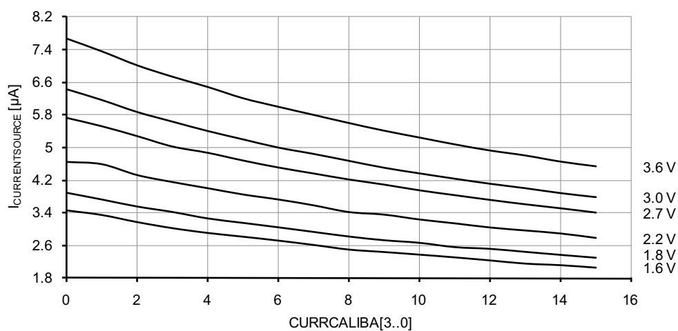
Figure 37-138. Analog comparator current source vs. calibration value.
