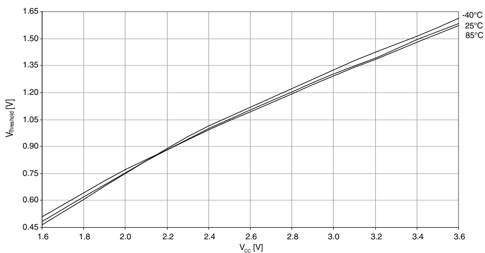
Figure 37-315. Reset pin input threshold voltage vs. V_{CC} .
