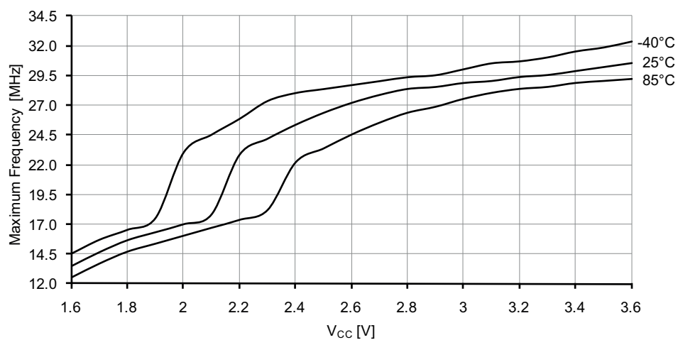
Figure 37-166. Maximum PDI frequency vs. V_{CC} .
