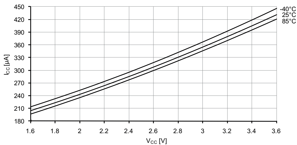
Figure 37-95. Idle mode supply current vs. V_{CC} .
