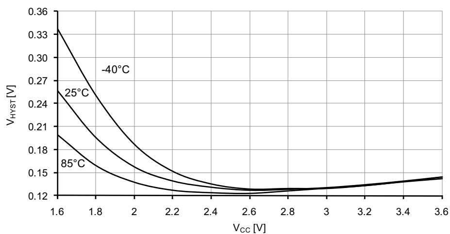
Figure 37-117. I/O pin input hysteresis vs. V_{CC} .
