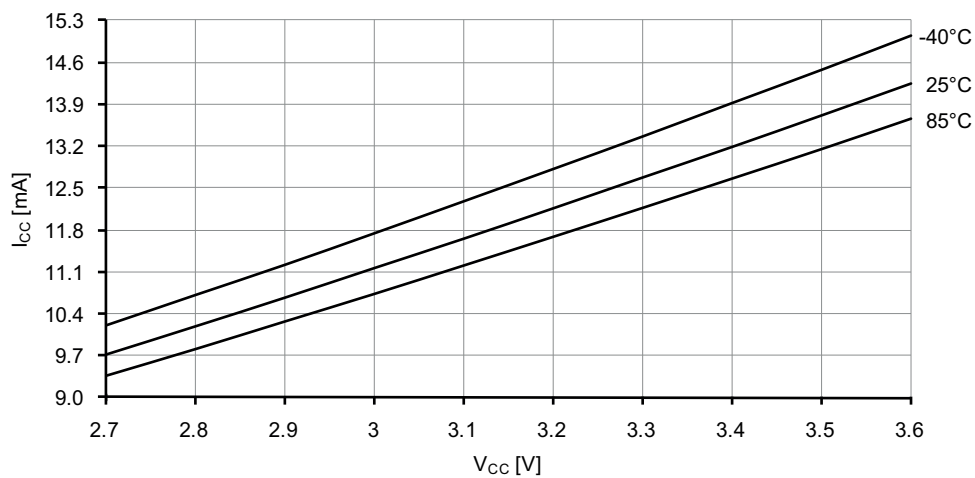
Figure 37-90. Active mode supply current vs. V_{CC} .
