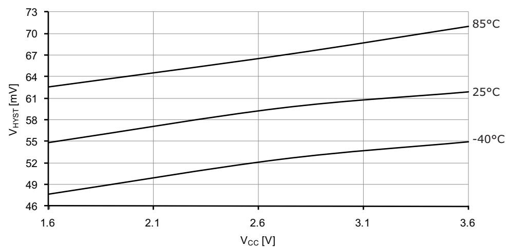
Figure 37-137. Analog comparator hysteresis vs. V_{CC} . Low power, large hysteresis.
