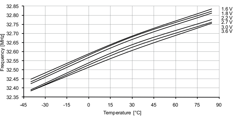
Figure 37-152. 32.768kHz internal oscillator frequency vs. temperature.
