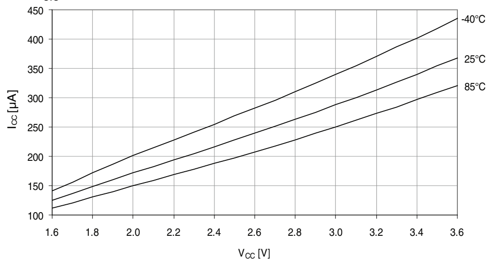
Figure 37-169. Active mode supply current vs. V_{CC} .
