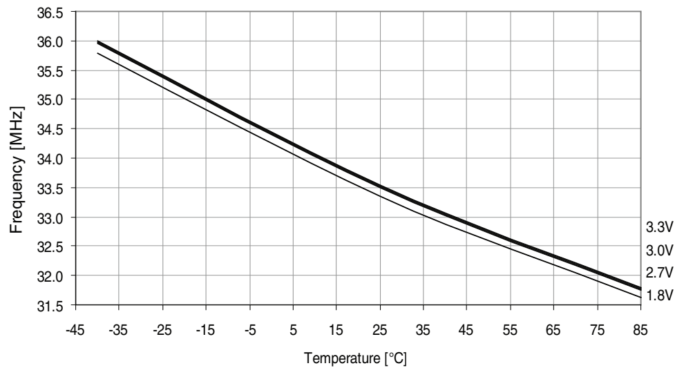
Figure 37-240. 32MHz internal oscillator frequency vs. temperature. DPLL disabled.
