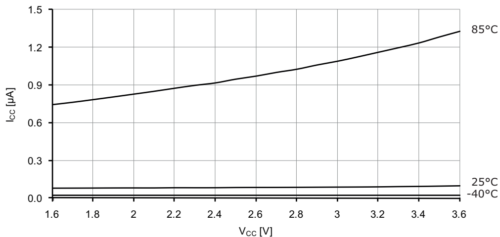
Figure 37-15. Power-down mode supply current vs. V_{CC} . All functions disabled.
