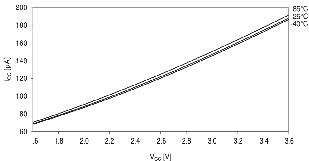
Figure 37-261. Idle mode supply current vs. V_{CC} .
