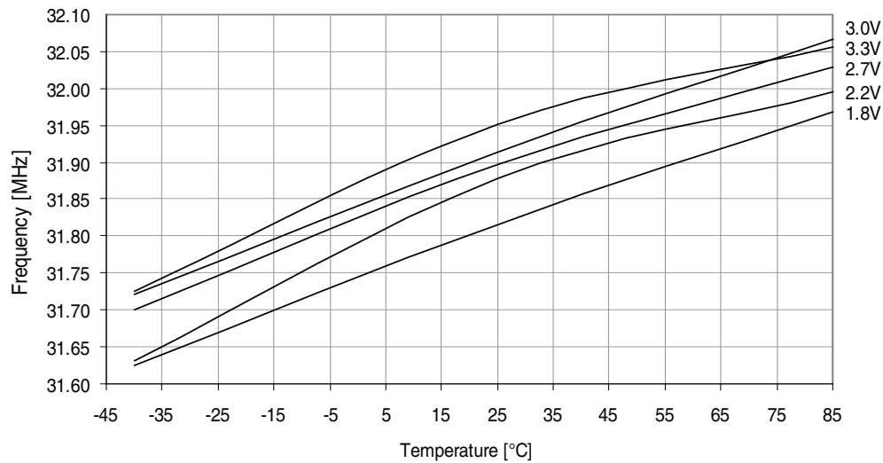
Figure 37-324. 32MHz internal oscillator frequency vs. temperature. DPLL enabled, from the 32.768kHz internal oscillator.
