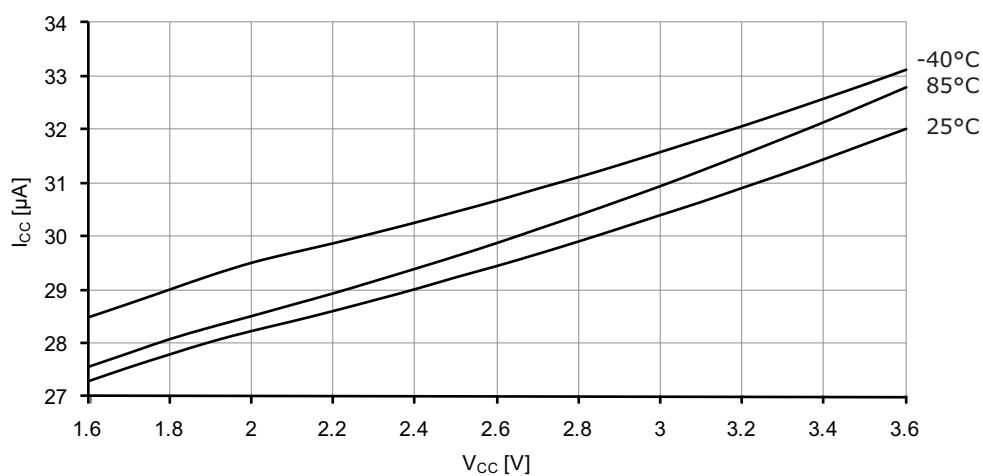
Figure 37-10. Idle mode supply current vs. V_{CC} .
