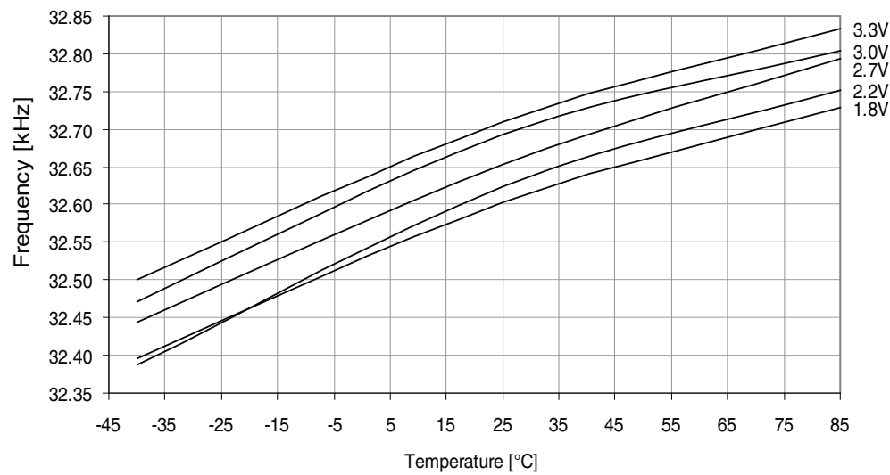
Figure 37-318. 32.768kHz internal oscillator frequency vs. temperature.
