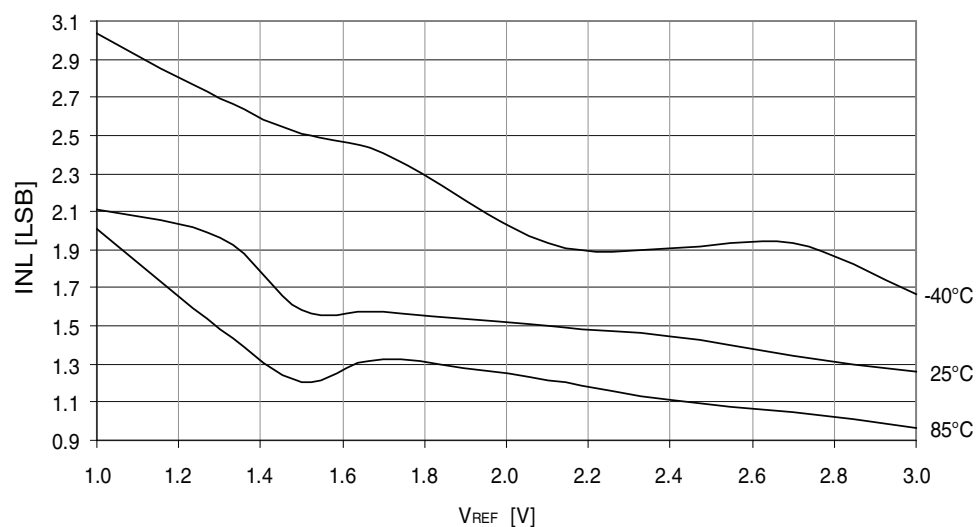
Figure 37-297. DAC INL error vs. V_{REF} .
