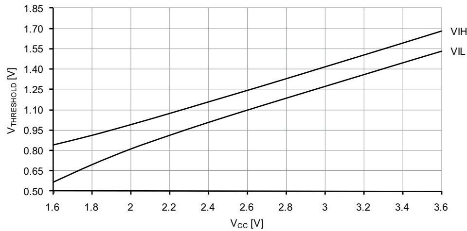
Figure 37-31. I/O pin input threshold voltage vs. V_{CC} . T = 25^{\circ}\text{C} .
