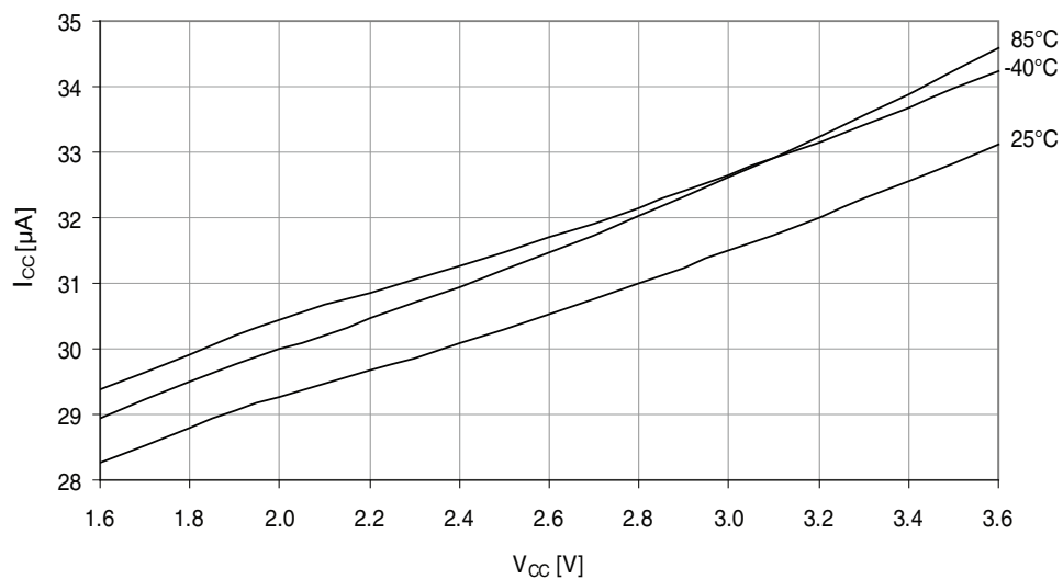
Figure 37-259. Idle mode supply current vs. V_{CC} .
