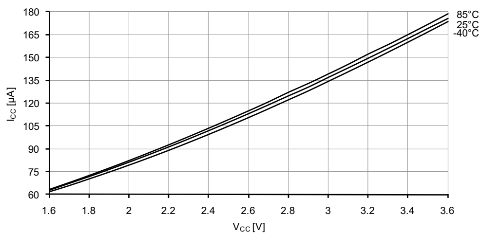
Figure 37-11. Idle mode supply current vs. V_{CC} .
