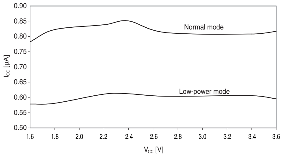
Figure 37-266. Power-save mode supply current vs. V_{CC} .
