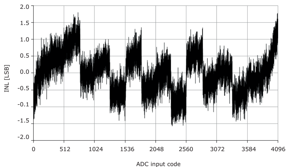
Figure 37-37. INL error vs. input code.
