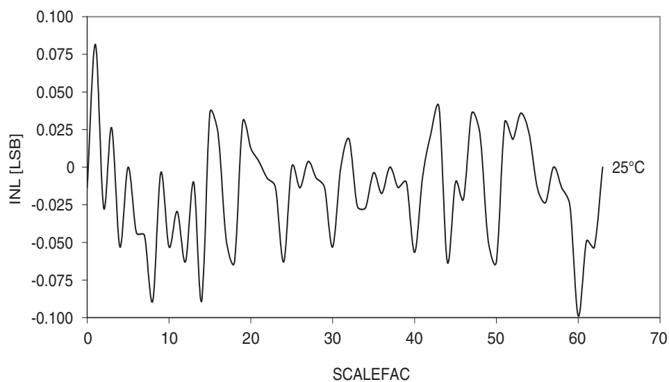
Figure 37-223. Voltage scaler INL vs. SCALEFAC.
