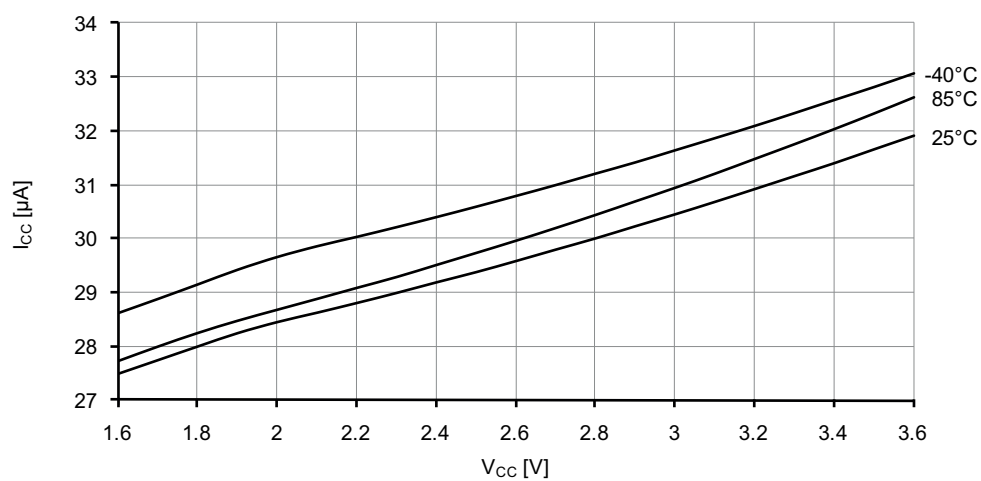
Figure 37-93. Idle mode supply current vs. V_{CC} .
