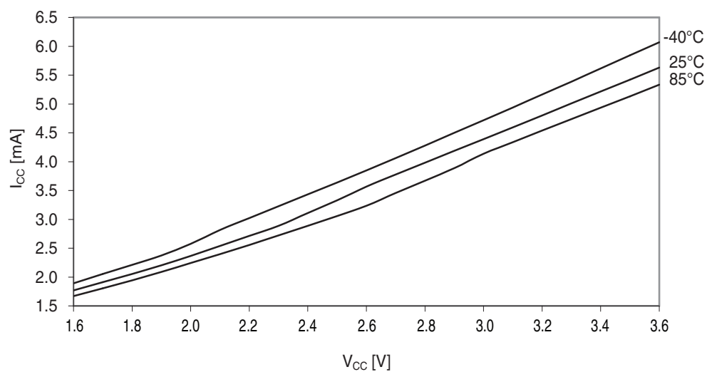
Figure 37-255. Active mode supply current vs. V_{CC} .
