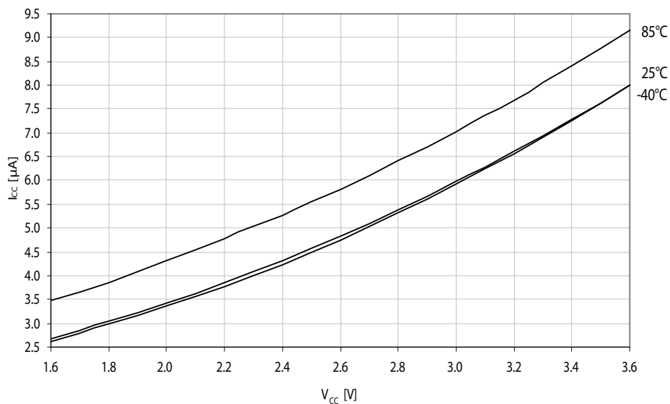
Figure 37-184. Standby supply current vs. V_{CC} .
