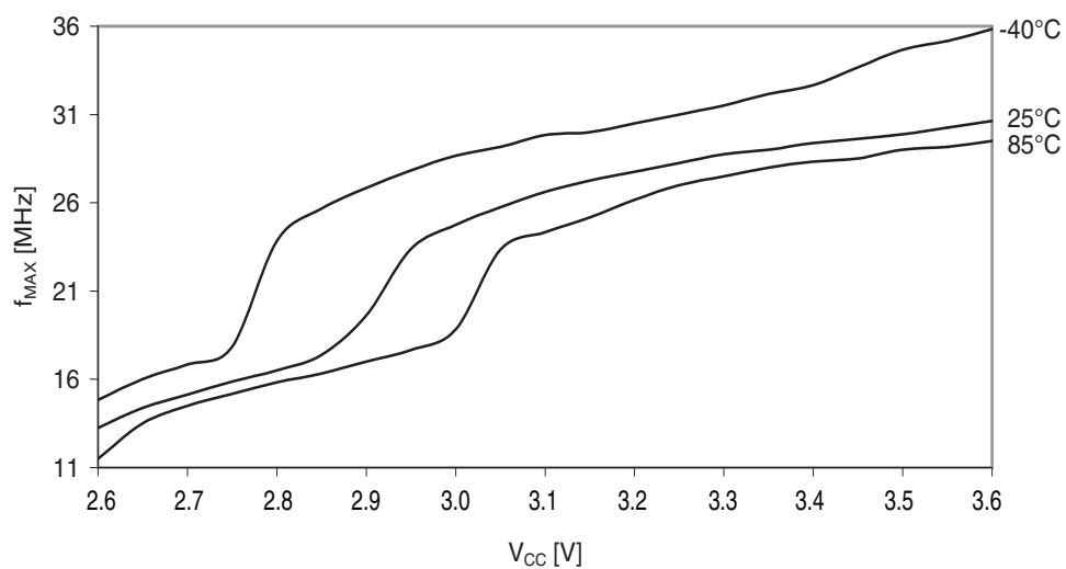
Figure 37-332. Maximum PDI frequency vs. V_{CC} .
