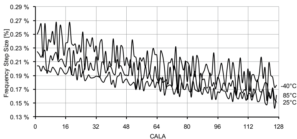
Figure 37-156. 2MHz internal oscillator CALA calibration step size.
