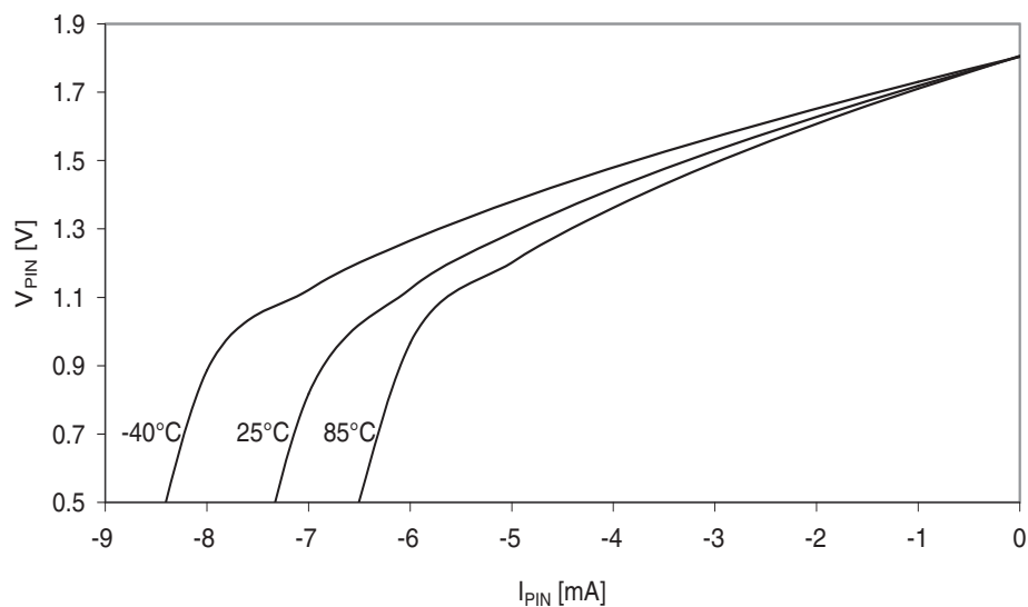
Figure 37-273. I/O pin output voltage vs. source current.
