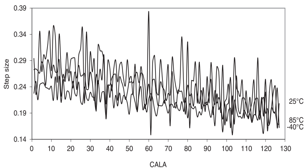
Figure 37-242. 32MHz internal oscillator CALA calibration step size.
