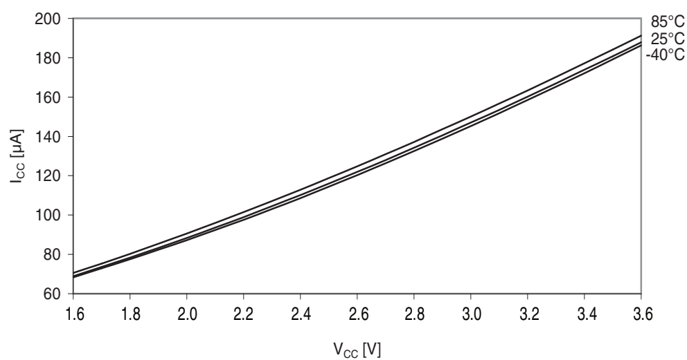
Figure 37-177. Idle mode supply current vs. V_{CC} .
