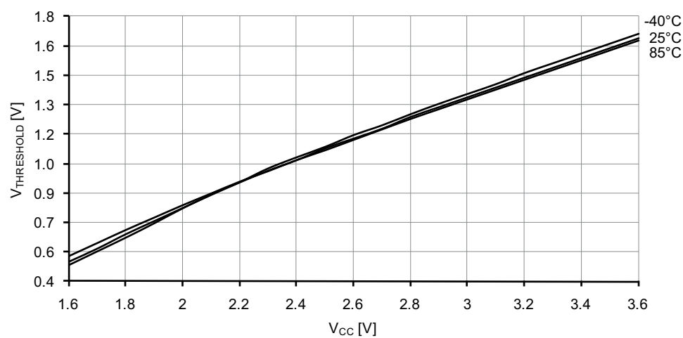
Figure 37-149. Reset pin input threshold voltage vs. V_{CC} .
