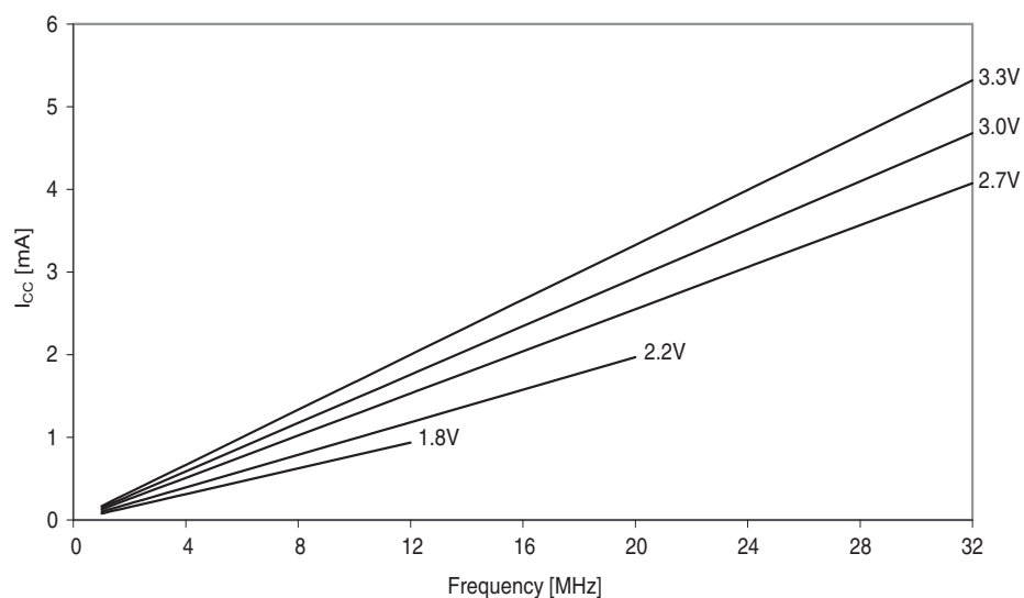
Figure 37-175. Idle mode supply current vs. frequency.
