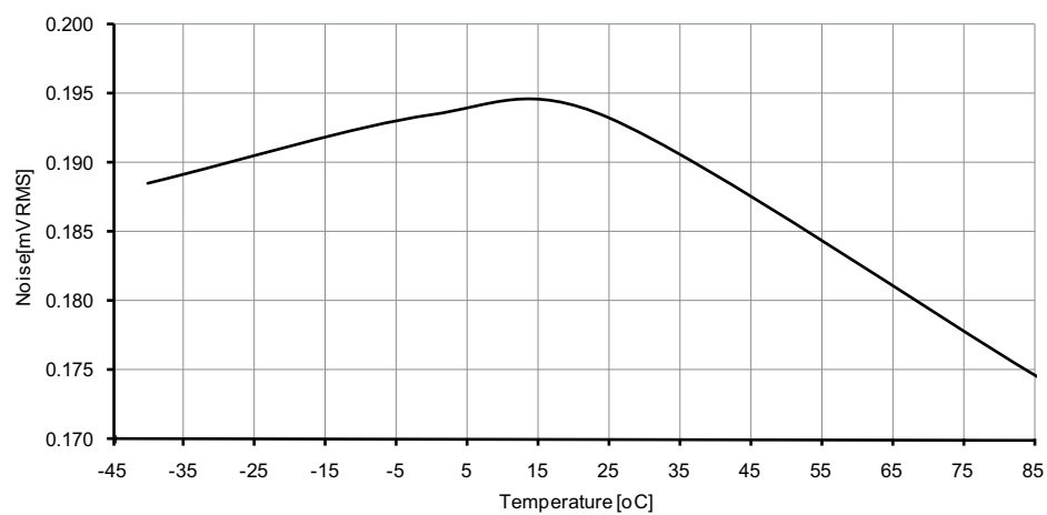
Figure 37-50. DAC noise vs. temperature.
