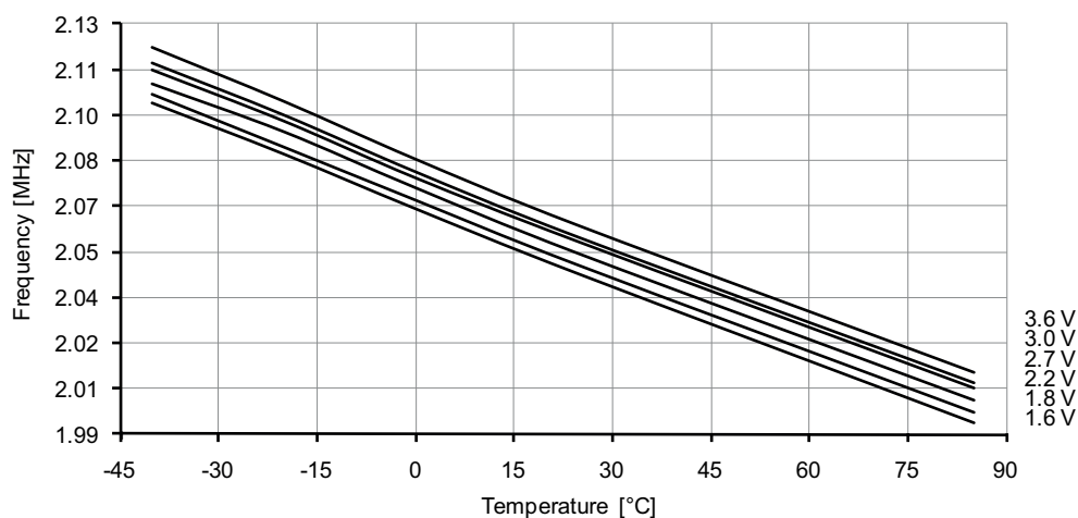
Figure 37-154. 2MHz internal oscillator frequency vs. temperature.
