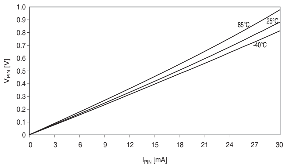
Figure 37-277. I/O pin output voltage vs. sink current.
