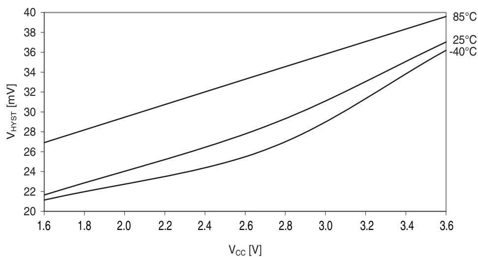
Figure 37-302. Analog comparator hysteresis vs. V_{CC} . High-speed mode, large hysteresis.
