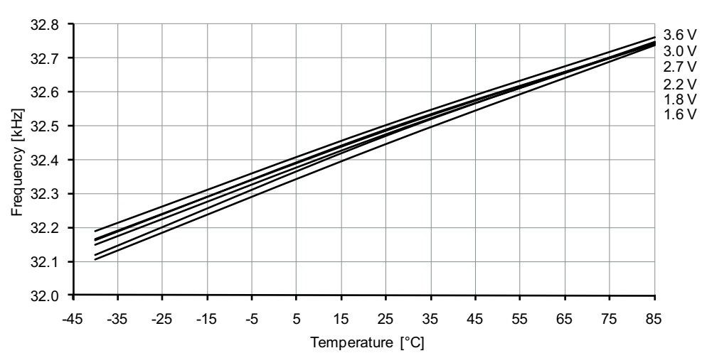
Figure 37-69. 32.768kHz internal oscillator frequency vs. temperature.
