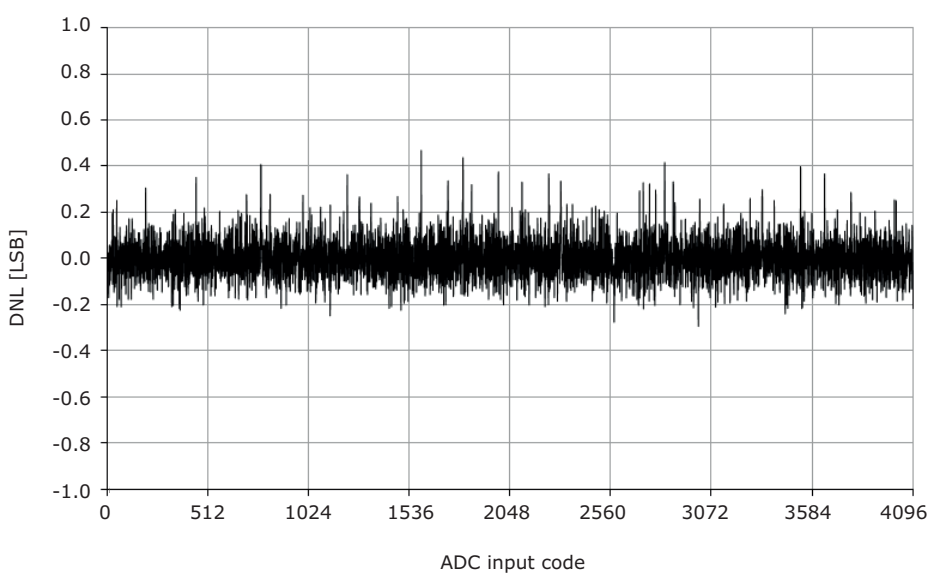
Figure 37-40. DNL error vs. input code.
