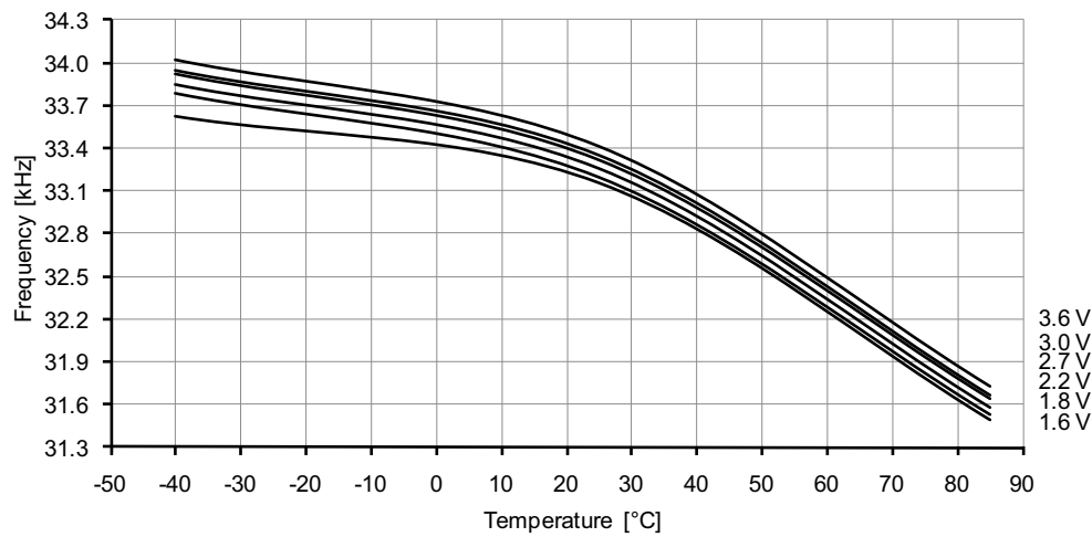
Figure 37-68. Ultra Low-Power internal oscillator frequency vs. temperature.
