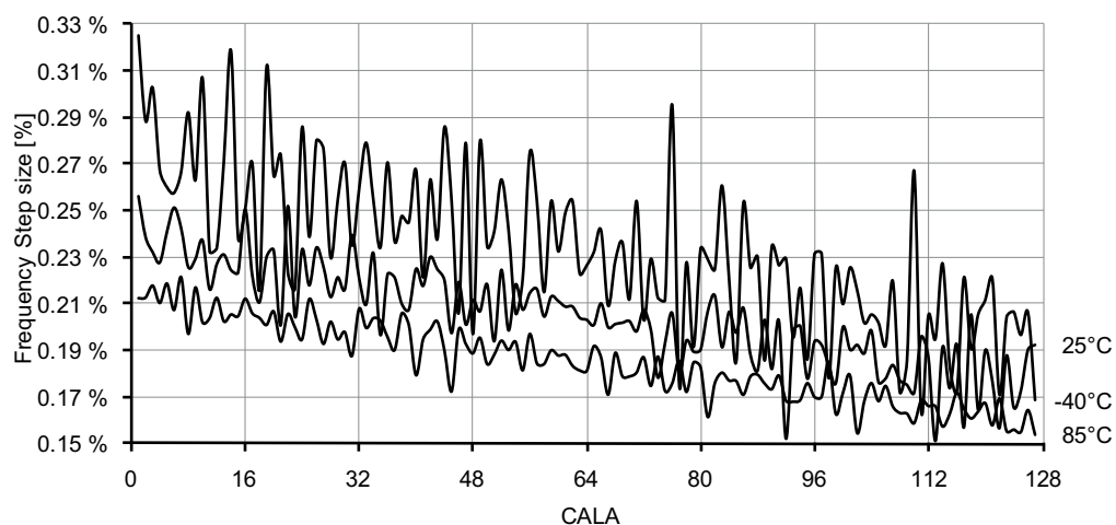
Figure 37-73. 2MHz internal oscillator CALA calibration step size.
