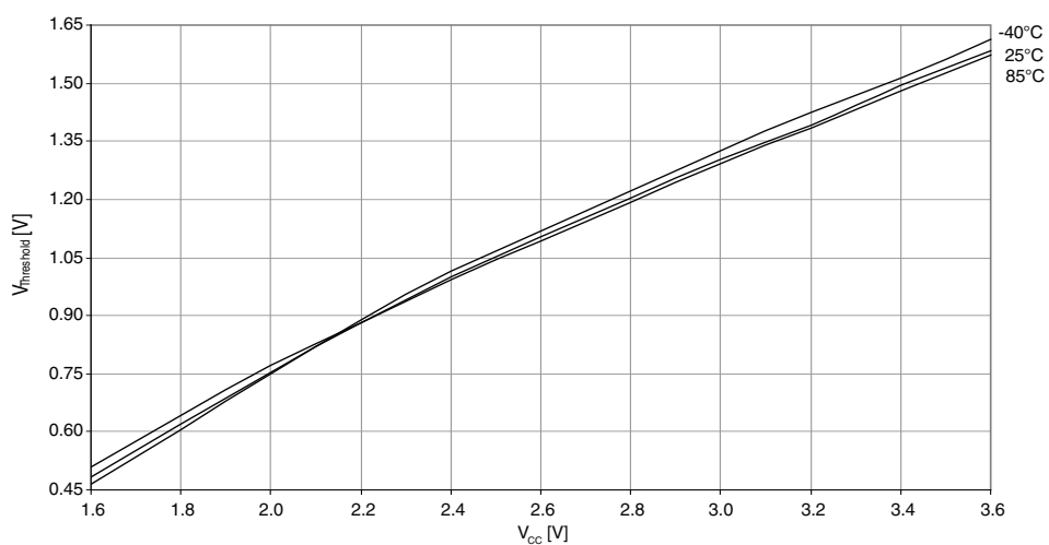
Figure 37-232. Reset pin input threshold voltage vs. V_{CC} .
