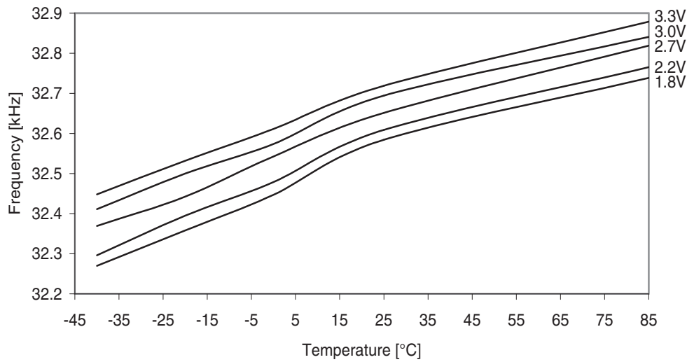
Figure 37-234. Ultra Low-Power internal oscillator frequency vs. temperature.
