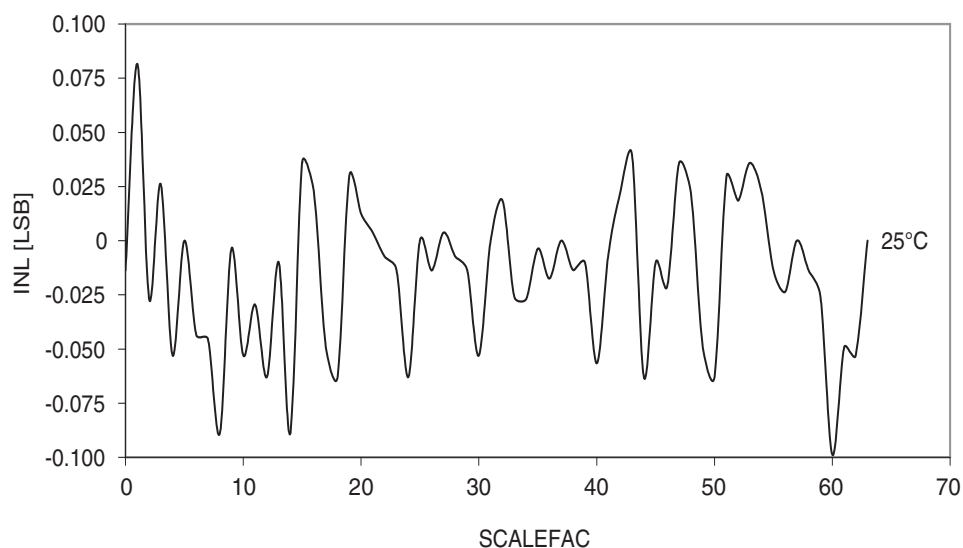
Figure 37-306. Voltage scaler INL vs. SCALEFAC.
