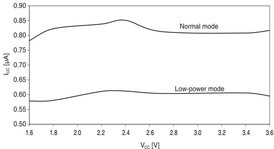
Figure 37-183. Power-save mode supply current vs. V_{CC} .
