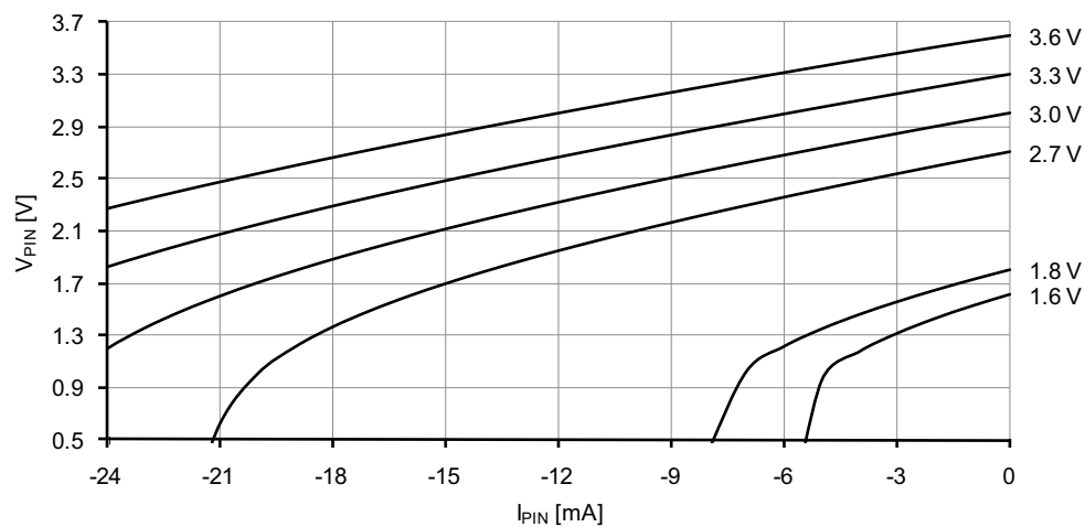
Figure 37-26. I/O pin output voltage vs. source current.
