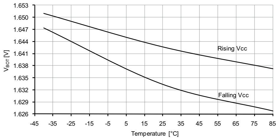
Figure 37-59. BOD thresholds vs. temperature. BOD level = 1.6V.
