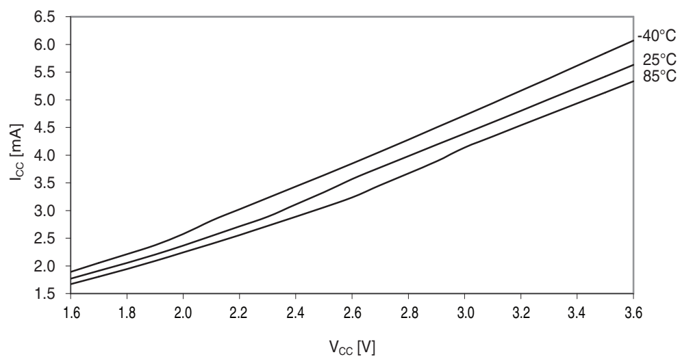
Figure 37-172. Active mode supply current vs. V_{CC} .
