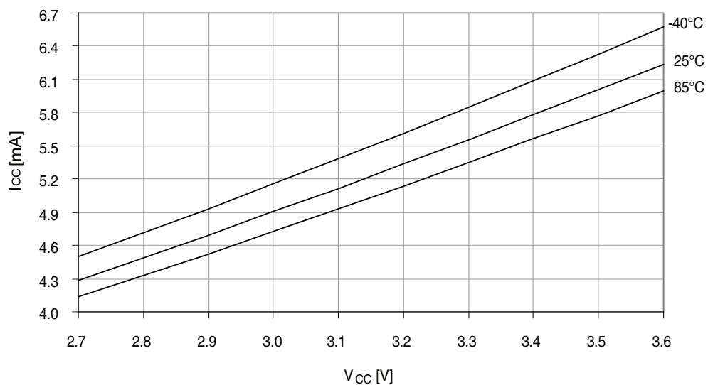
Figure 37-180. Idle mode current vs. V_{CC} .
