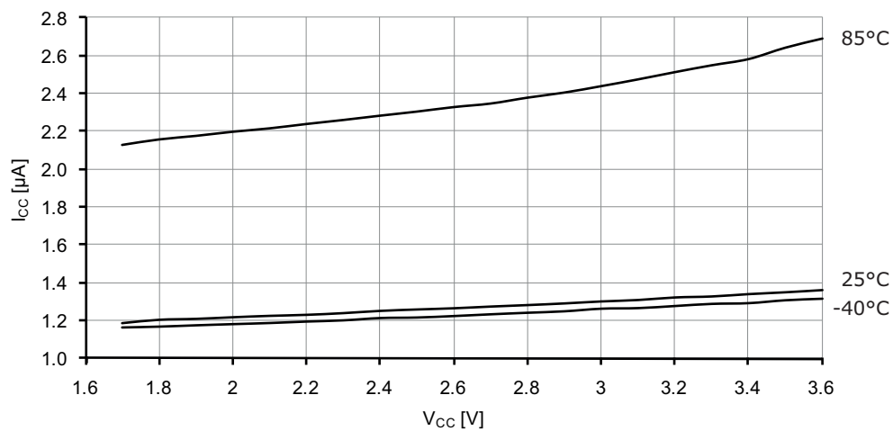
Figure 37-16. Power-down mode supply current vs. V_{CC} . Watchdog and sampled BOD enabled.
