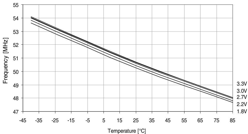
Figure 37-327. 48MHz internal oscillator frequency vs. temperature.
