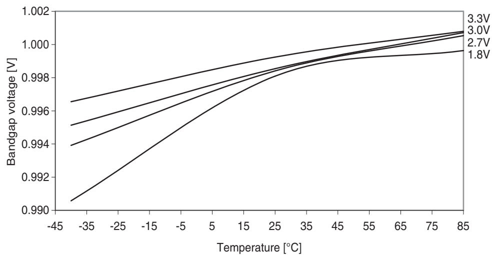
Figure 37-224. ADC/DAC Internal 1.0V reference vs. temperature.
