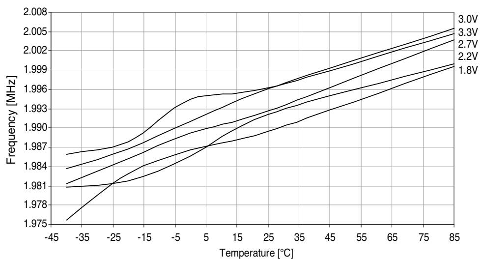
Figure 37-238. 2MHz internal oscillator frequency vs. temperature.
