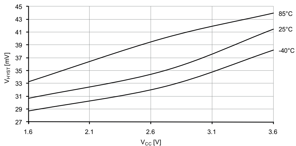
Figure 37-136. Analog comparator hysteresis vs. V_{CC} . High-speed mode, large hysteresis.
