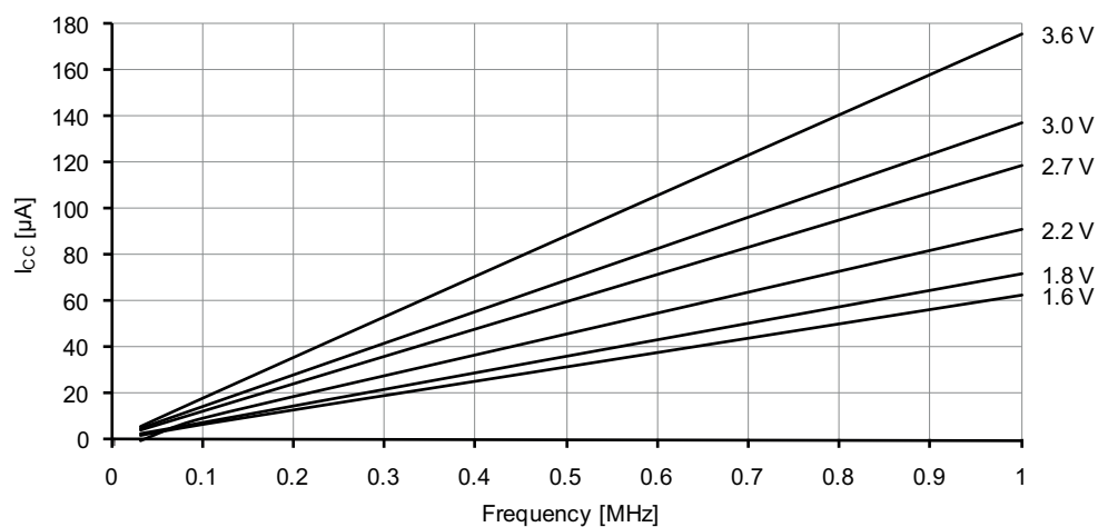
Figure 37-8. Idle mode supply current vs. frequency.
