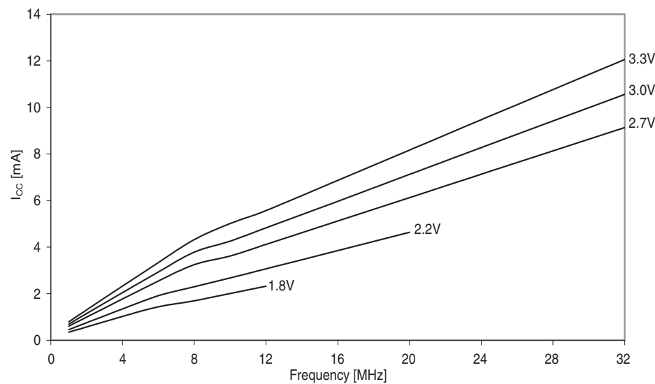
Figure 37-251. Active supply current vs. frequency.
