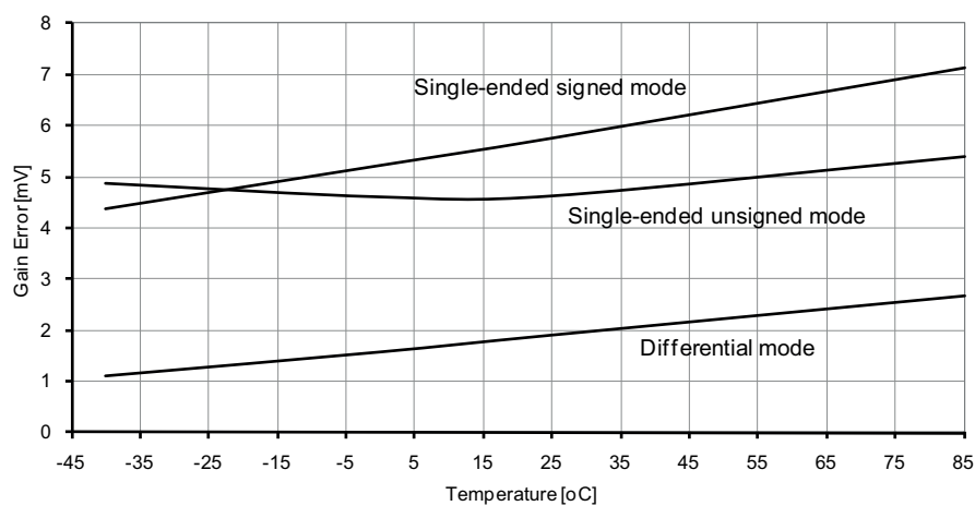
Figure 37-44. Gain error vs. temperature.
