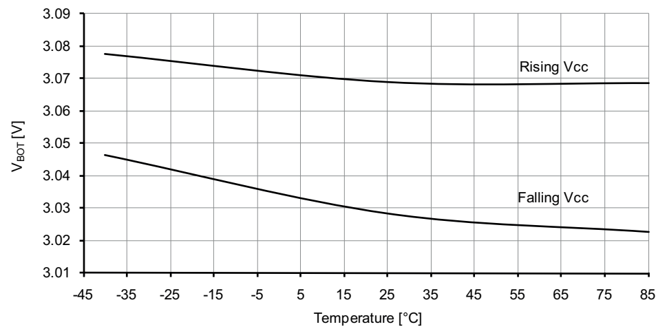
Figure 37-150. Power-on reset current consumption vs. V_{CC} . BOD level = 3.0V, enabled in continuous mode.
