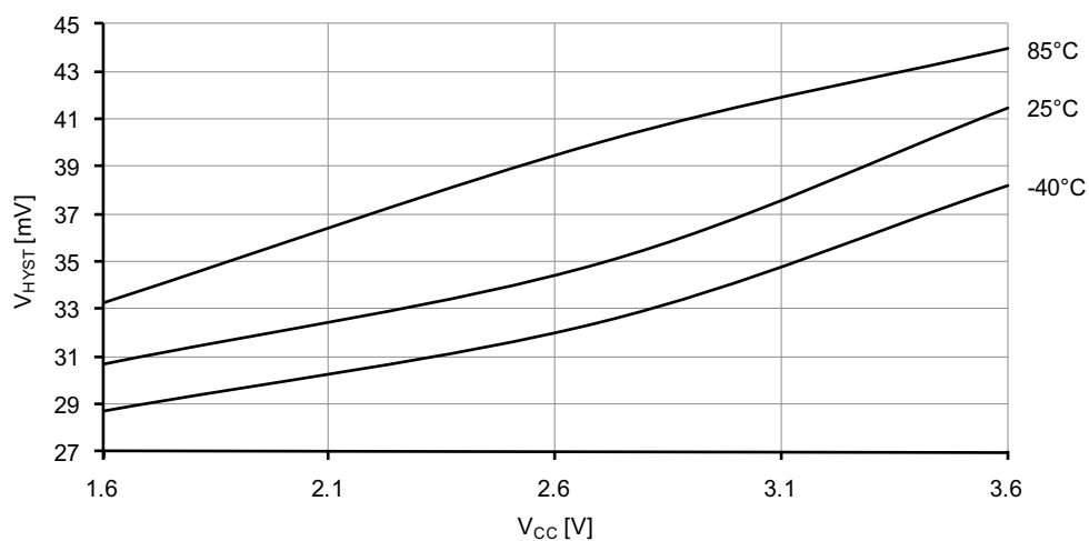
Figure 37-53. Analog comparator hysteresis vs. V_{CC} . High-speed mode, large hysteresis.
