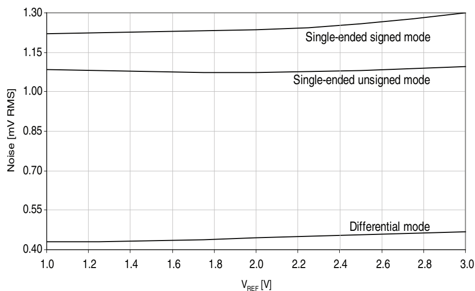
Figure 37-295. Noise vs. V_{REF} .
