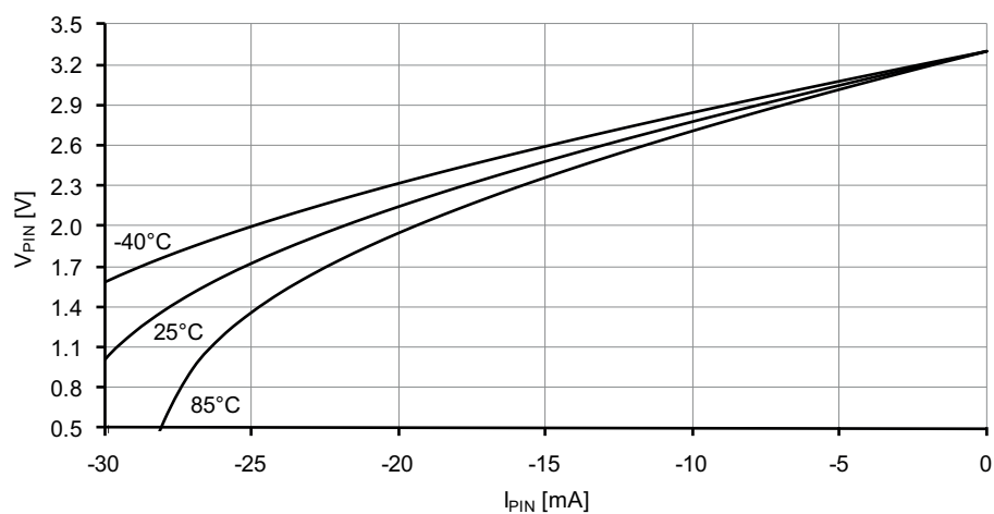
Figure 37-26. I/O pin output voltage vs. source current.
