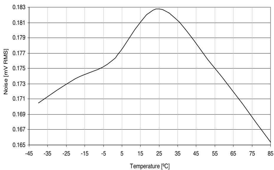
Figure 37-299. DAC noise vs. temperature.
