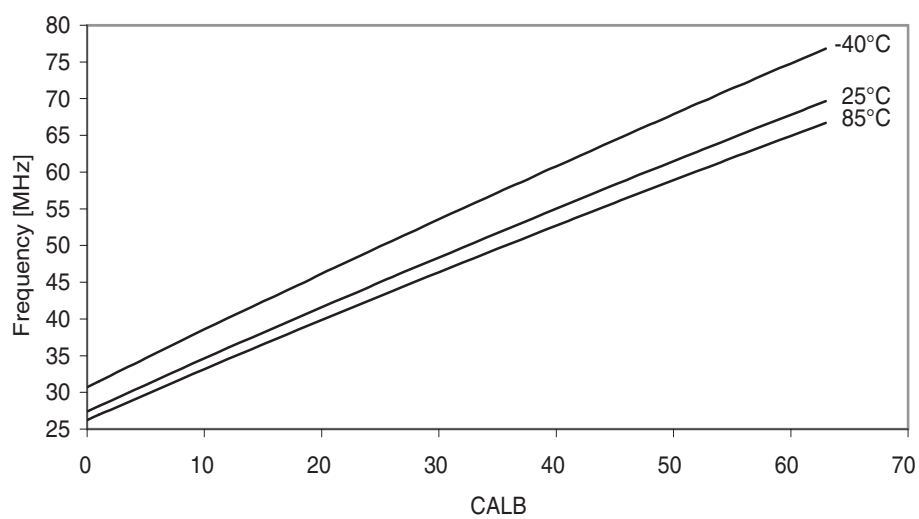
Figure 37-243. 32MHz internal oscillator frequency vs. CALB calibration value.
