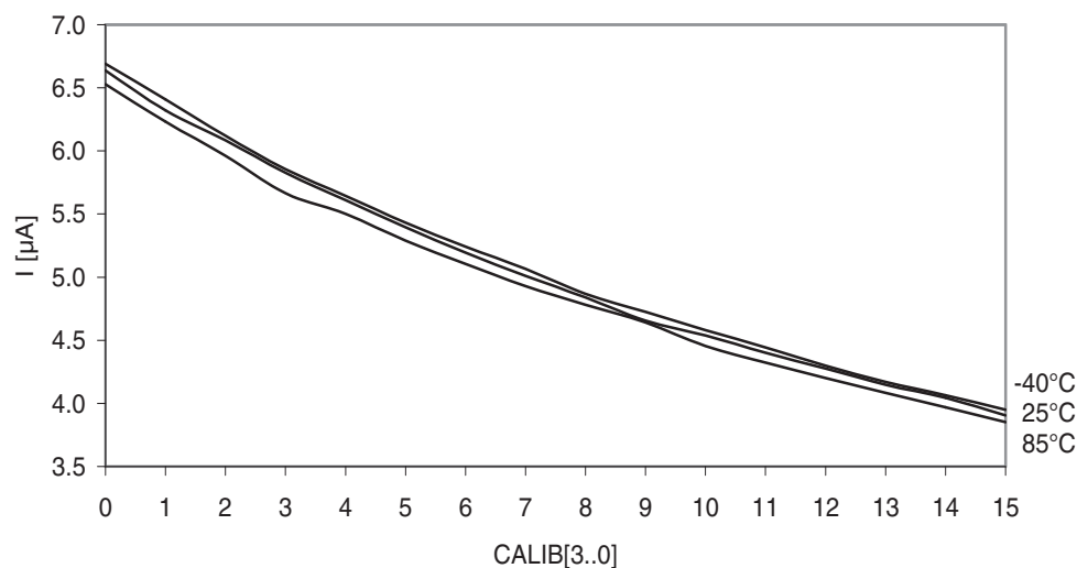
Figure 37-305. Analog comparator current source vs. calibration value.
