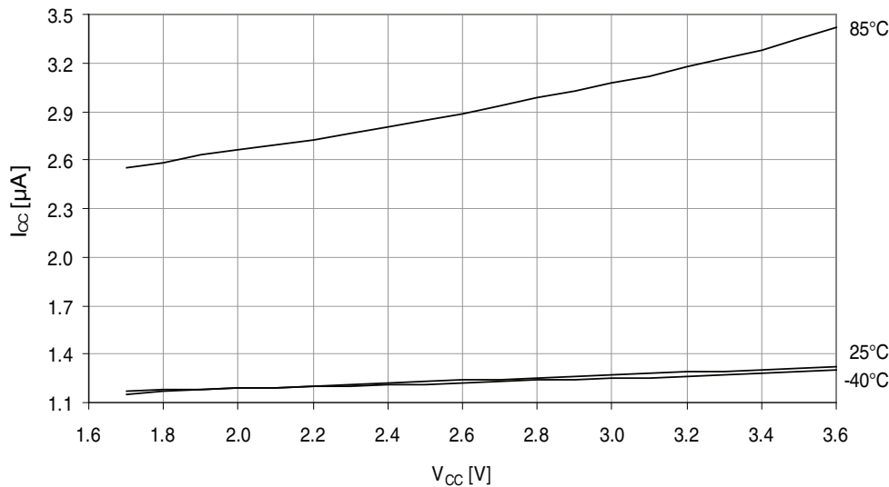
Figure 37-182. Power-down mode supply current vs. V_{CC} . Watchdog and sampled BOD enabled.
