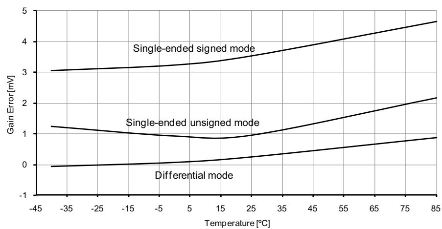
Figure 37-127. Gain error vs. temperature.
