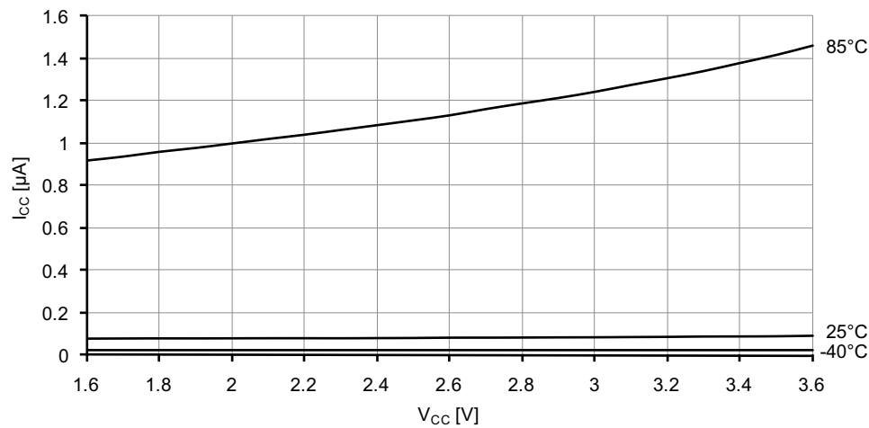
Figure 37-98. Power-down mode supply current vs. V_{CC} . All functions disabled.
