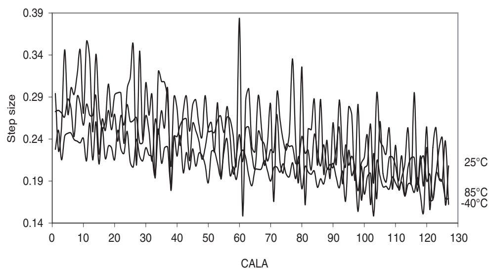
Figure 37-325. 32MHz internal oscillator CALA calibration step size.
