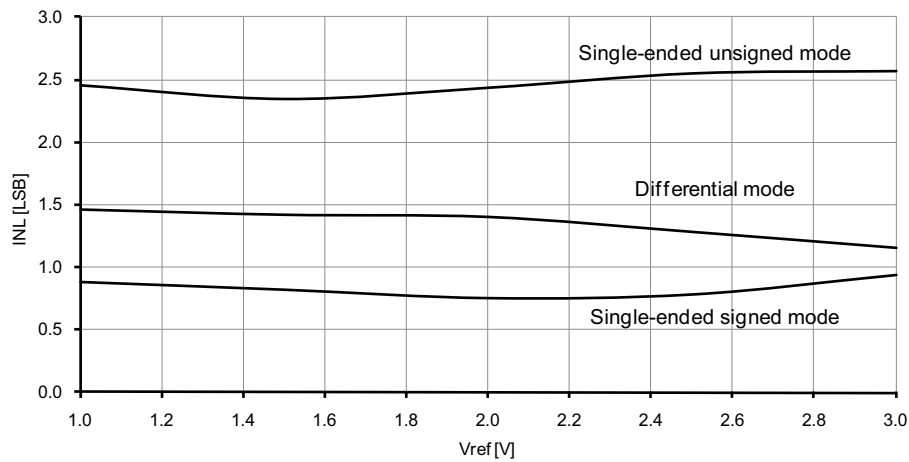
Figure 37-118. INL error vs. external V_{REF} . T = 25\text{ }^{\circ}\text{C} , V_{CC} = 3.6\text{V} , external reference.
