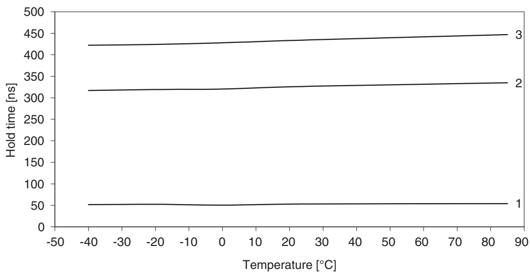
Figure 37-164. SDA hold time vs. temperature.
