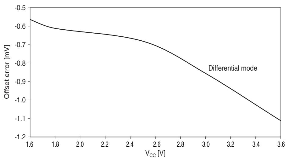
Figure 37-294. Offset error vs. V_{CC} .
