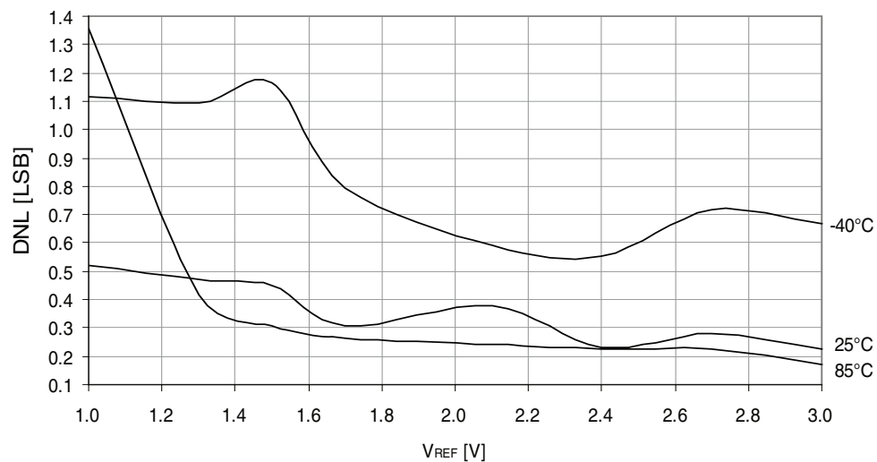
Figure 37-298. DNL error vs. V_{REF} .
