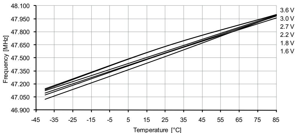
Figure 37-79. 48MHz internal oscillator frequency vs. temperature. DFLL enabled, from the 32.768kHz internal oscillator.
