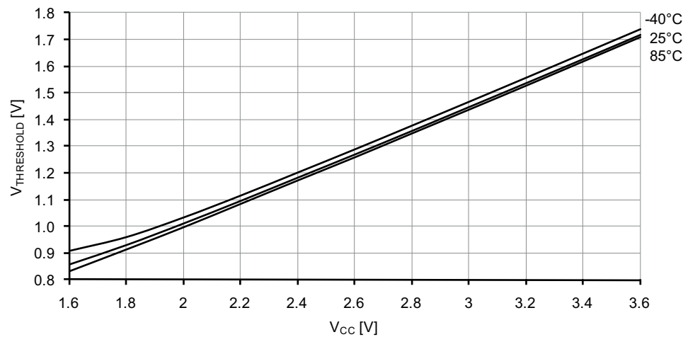
Figure 37-32. I/O pin input threshold voltage vs. V_{CC} . V_{IH} I/O pin read as "1".
