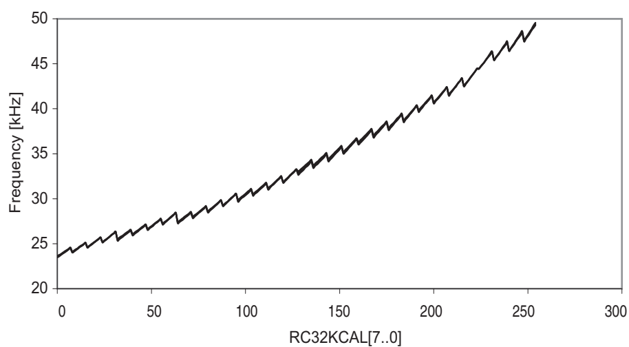
Figure 37-319. 32.768kHz internal oscillator frequency vs. calibration value.
