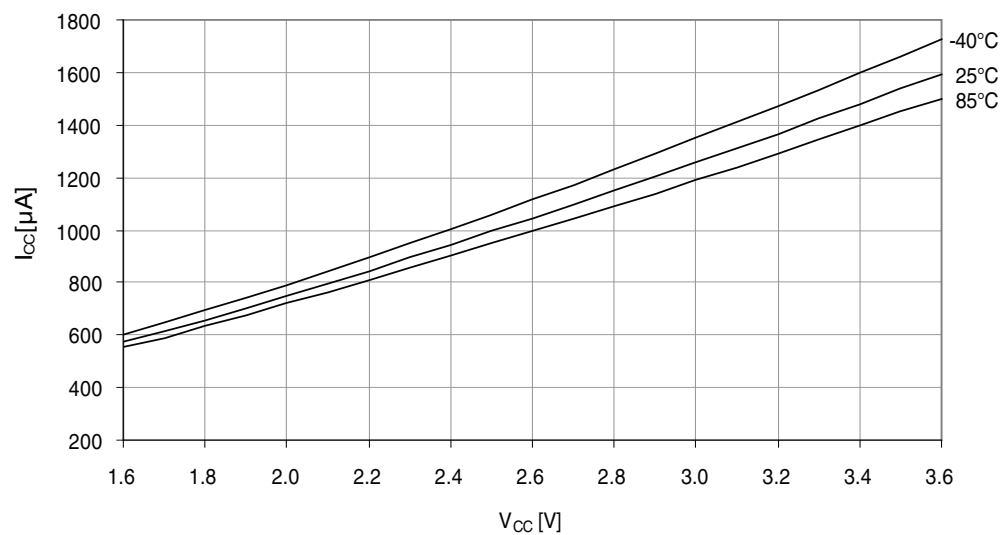
Figure 37-171. Active mode supply current vs. V_{CC} .
