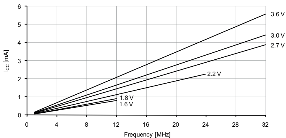
Figure 37-92. Idle mode supply current vs. frequency.
