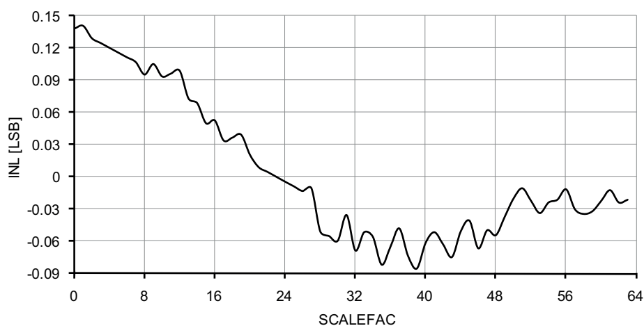
Figure 37-140. Voltage scaler INL vs. SCALEFAC.
