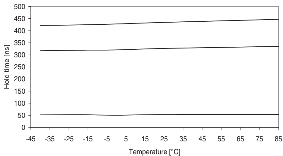
Figure 37-330. SDA hold time vs. temperature.
