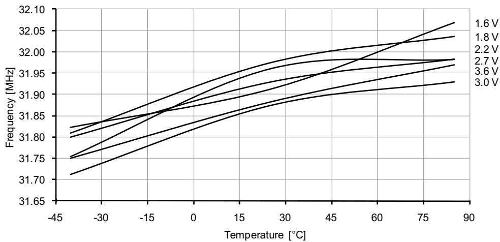
Figure 37-158. 32MHz internal oscillator frequency vs. temperature. DFLL enabled, from the 32.768kHz internal oscillator.
