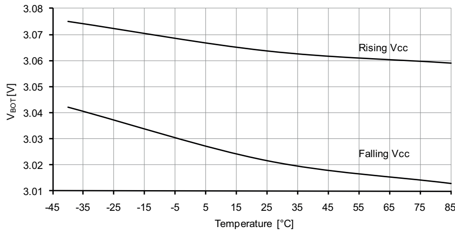
Figure 37-60. BOD thresholds vs. temperature. BOD level = 3.0V.
