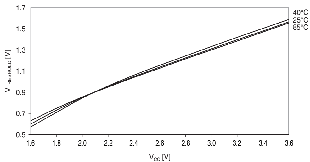
Figure 37-282. I/O pin input threshold voltage vs. V_{CC} .
