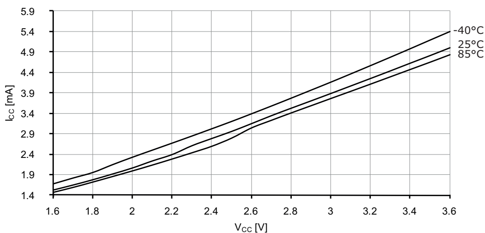
Figure 37-6. Active mode supply current vs. V_{CC} .
