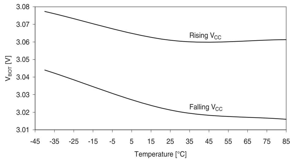
Figure 37-226. BOD thresholds vs. temperature.
