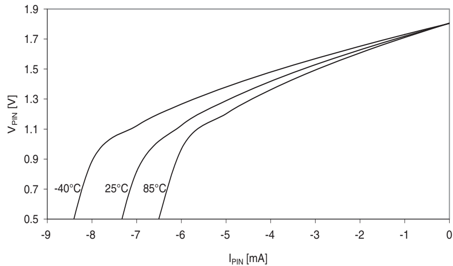
Figure 37-189. I/O pin output voltage vs. source current. V_{CC} = 1.8V .
