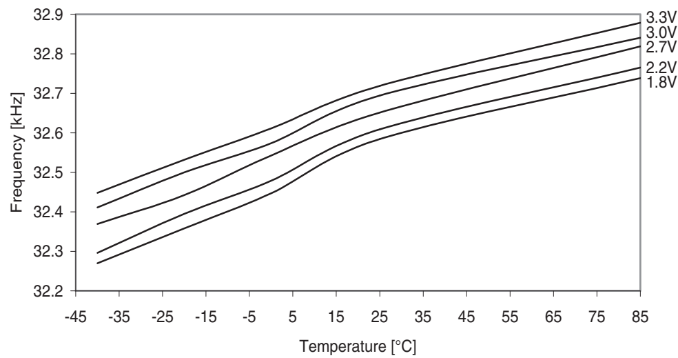
Figure 37-317. Ultra Low-Power internal oscillator frequency vs. temperature.
