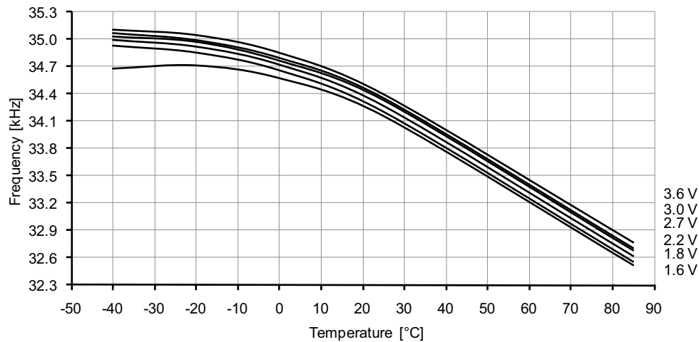
Figure 37-151. Ultra Low-Power internal oscillator frequency vs. temperature.
