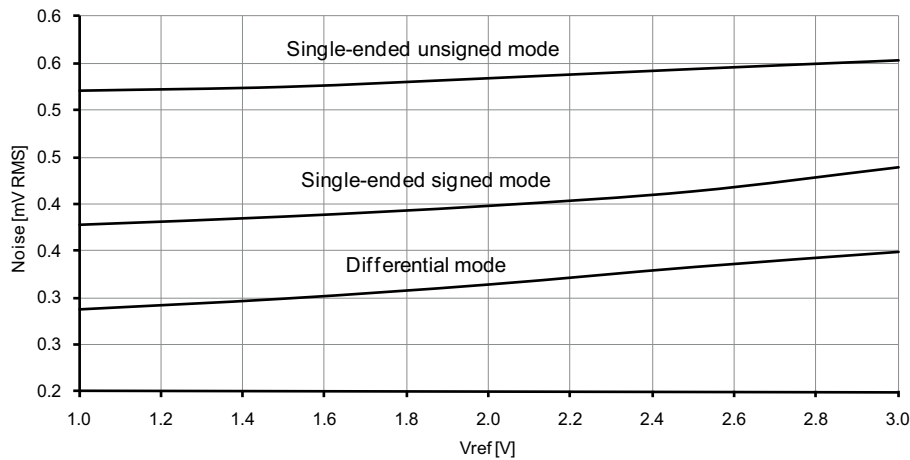
Figure 37-129. Noise vs. V_{REF} . T = 25\text{ }^{\circ}\text{C} , V_{CC} = 3.6\text{V} , ADC sampling speed = 500ksps.
