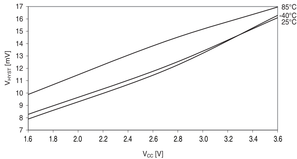
Figure 37-217. Analog comparator hysteresis vs. V_{CC} . High-speed, small hysteresis.
