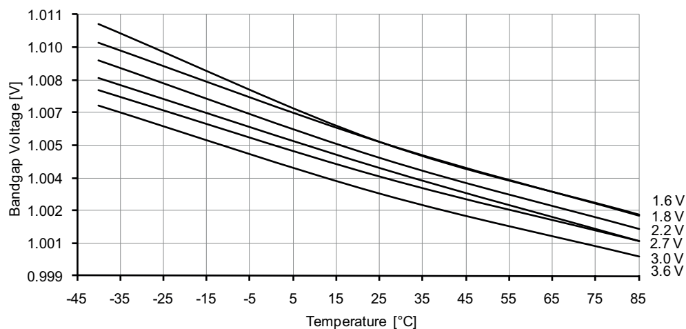
Figure 37-58. ADC/DAC Internal 1.0V reference vs. temperature.
