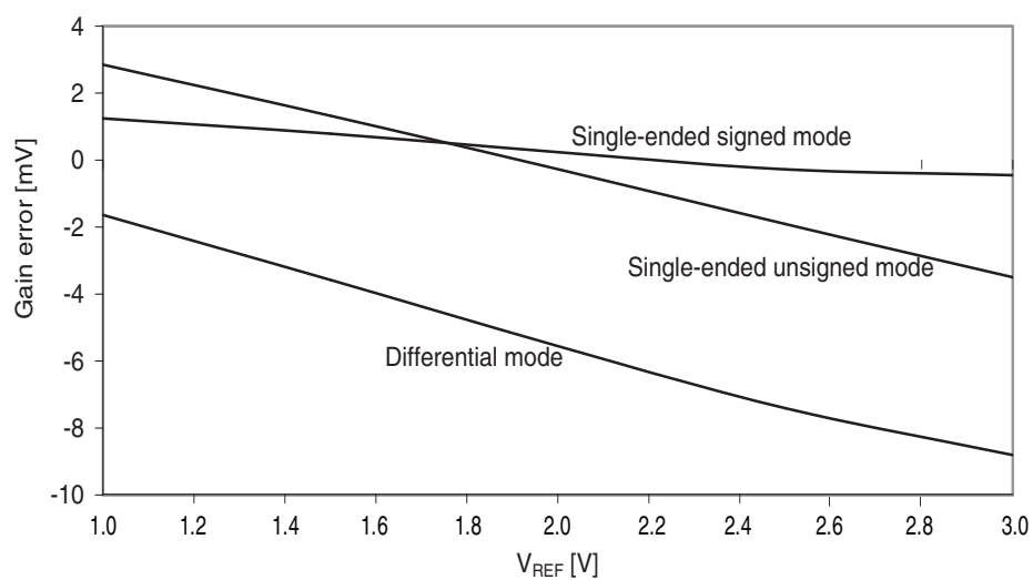
Figure 37-290. Gain error vs. V_{REF} .
