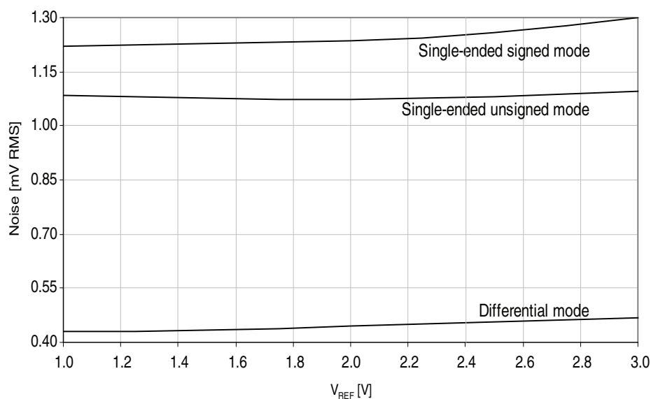
Figure 37-212. Noise vs. V_{REF} .
