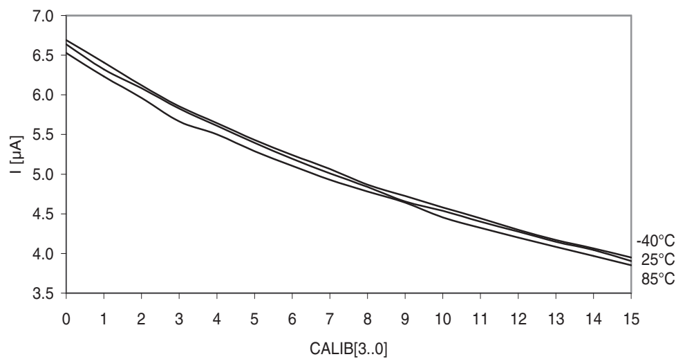
Figure 37-222. Analog comparator current source vs. calibration value.
