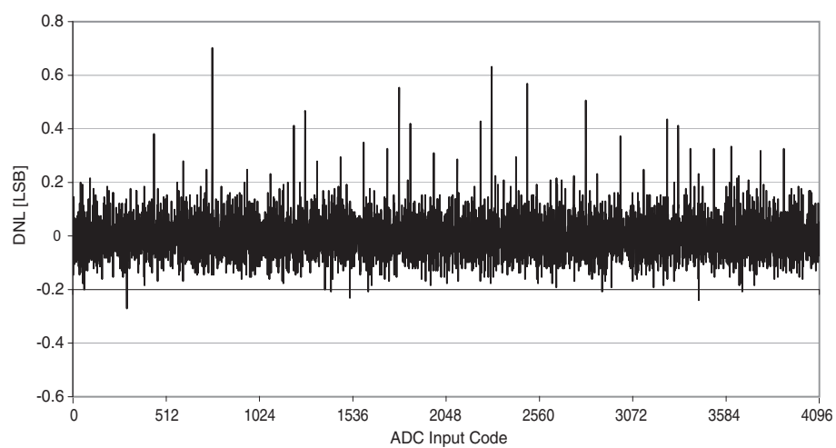
Figure 37-289. DNL error vs. input code.
