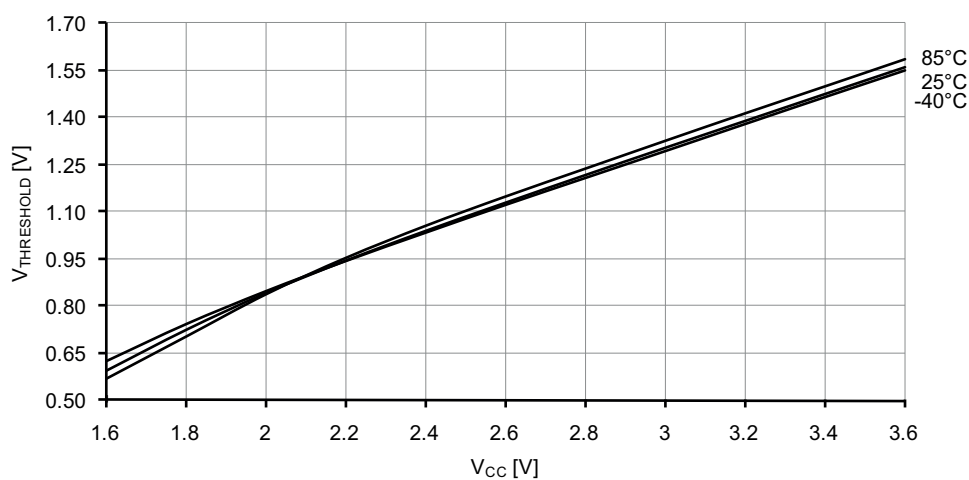
Figure 37-116. I/O pin input threshold voltage vs. V_{CC} .
