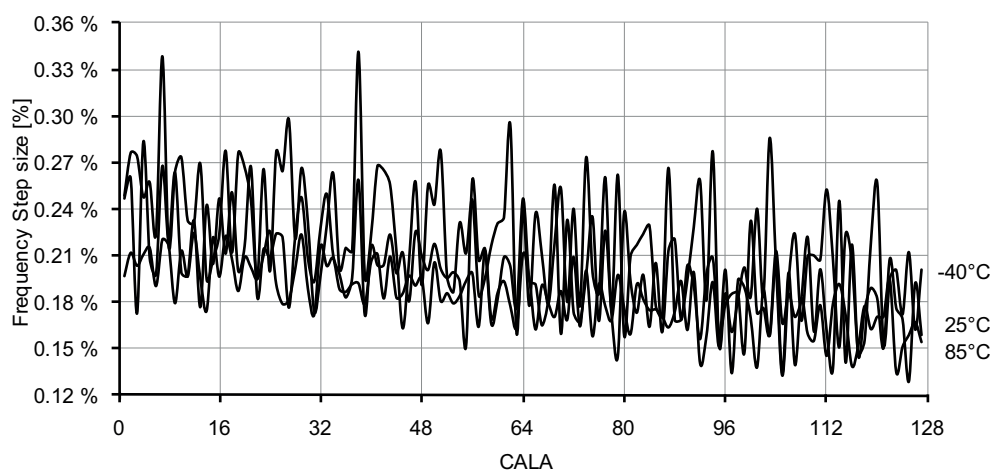
Figure 37-80. 48MHz internal oscillator CALA calibration step size.
