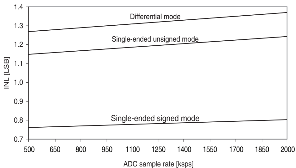
Figure 37-202. INL error vs. sample rate.
