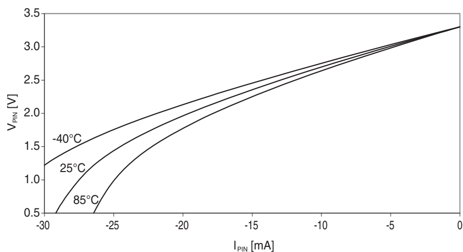
Figure 37-191. I/O pin output voltage vs. source current.
