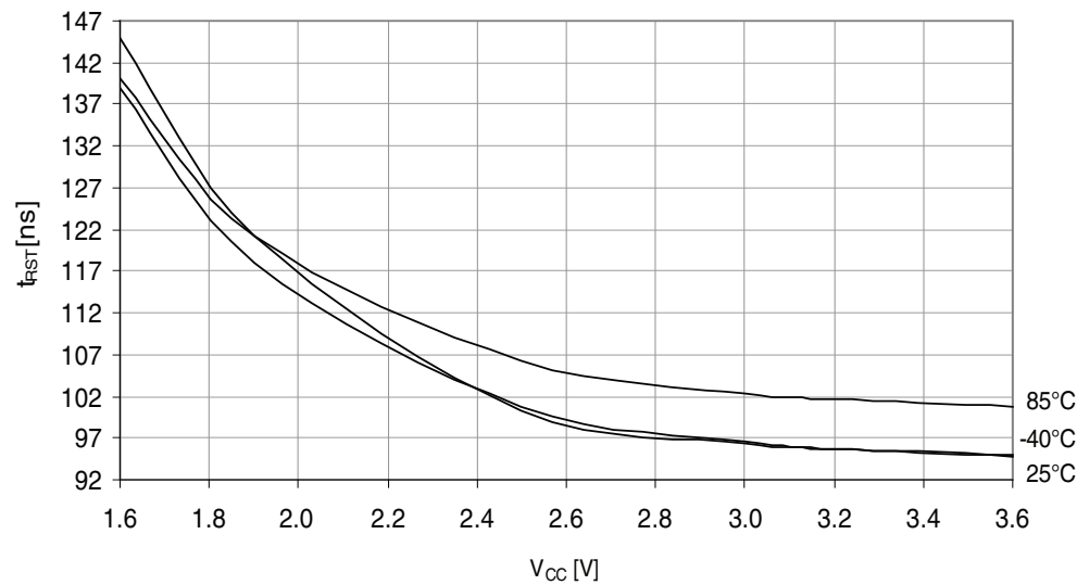
Figure 37-227. Minimum Reset pin pulse width vs. V_{CC} .
