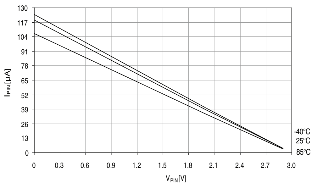
Figure 37-230. Reset pin pull-up resistor current vs. reset pin voltage.
