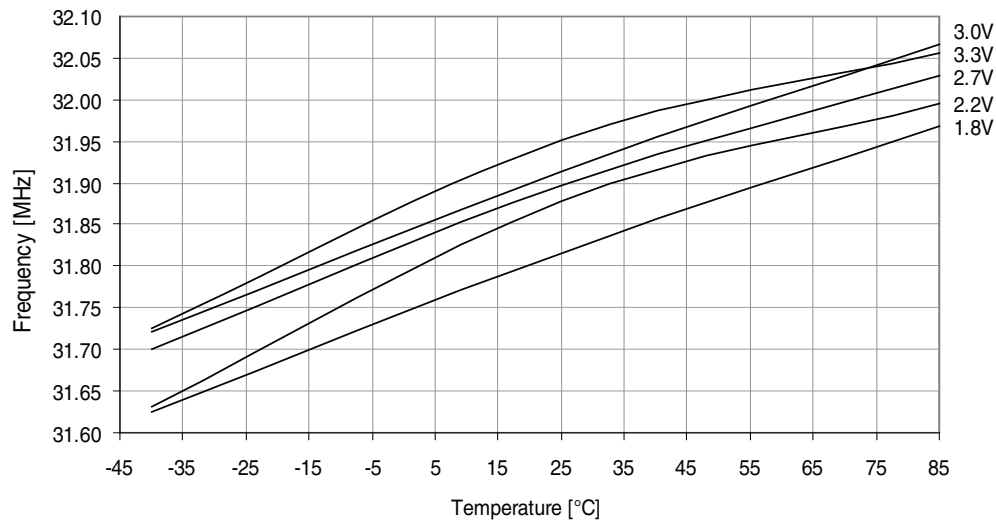
Figure 37-241. 32MHz internal oscillator frequency vs. temperature. DPLL enabled, from the 32.768kHz internal oscillator.
