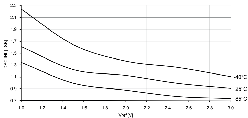
Figure 37-48. DAC INL error vs. V_{REF} .
