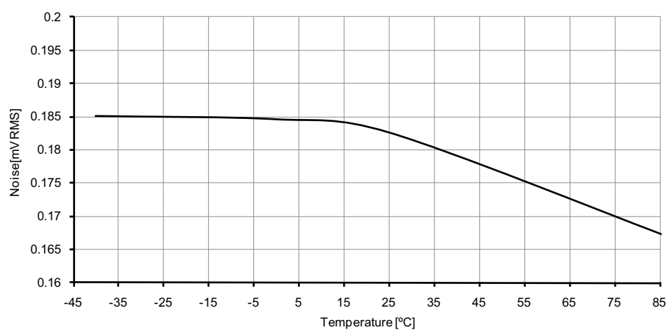
Figure 37-133. DAC noise vs. temperature.
