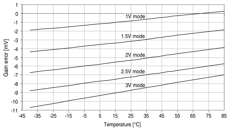
Figure 37-210. Gain error vs. temperature.
