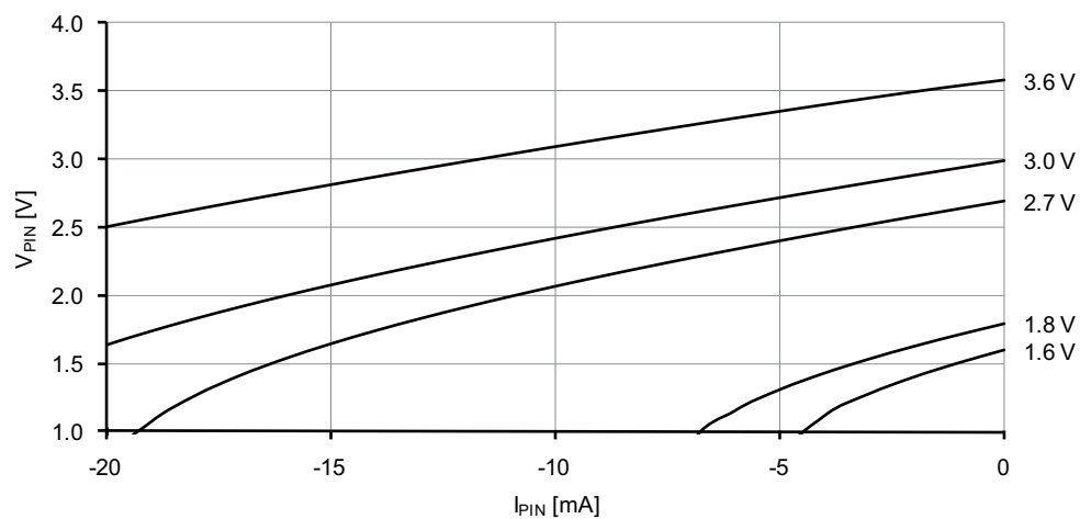
Figure 37-109. I/O pin output voltage vs. source current.
