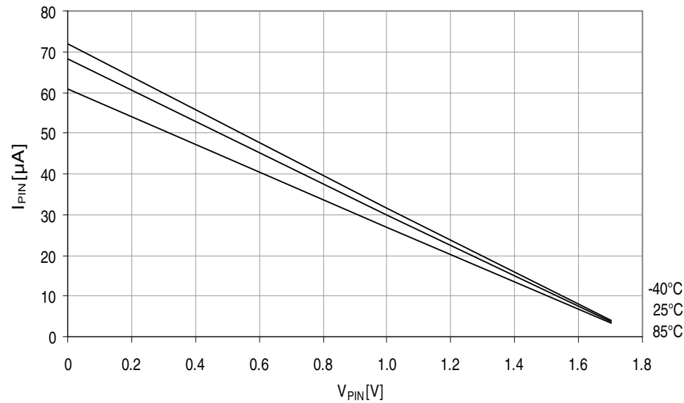
Figure 37-311. Reset pin pull-up resistor current vs. reset pin voltage.
