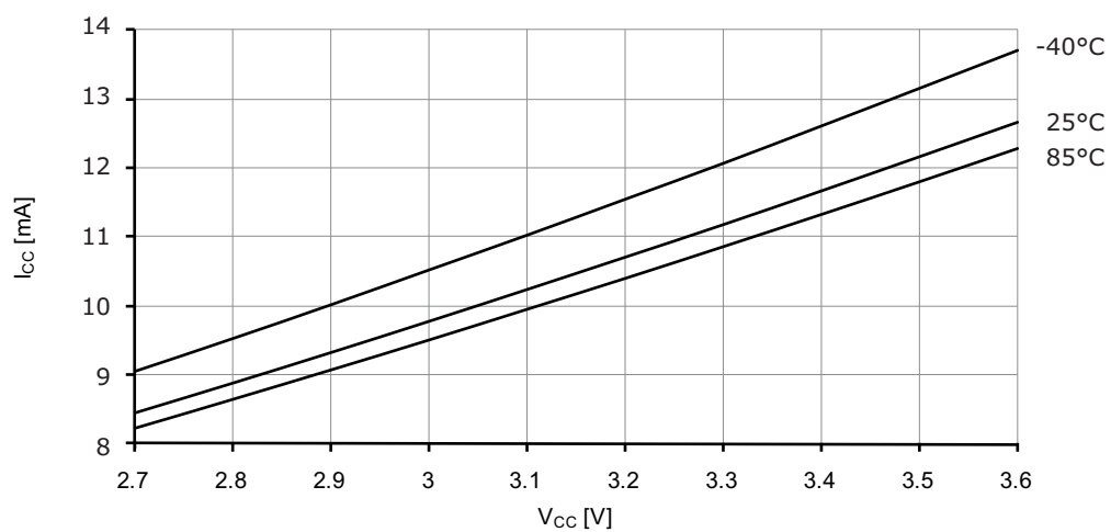
Figure 37-14. Idle mode current vs. V_{CC} .
