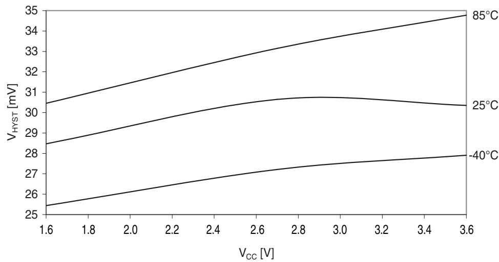
Figure 37-301. Analog comparator hysteresis vs. V_{CC} . Low power, small hysteresis.
