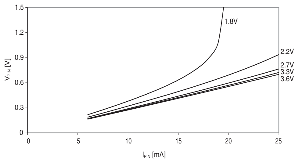
Figure 37-196. I/O pin output voltage vs. sink current.
