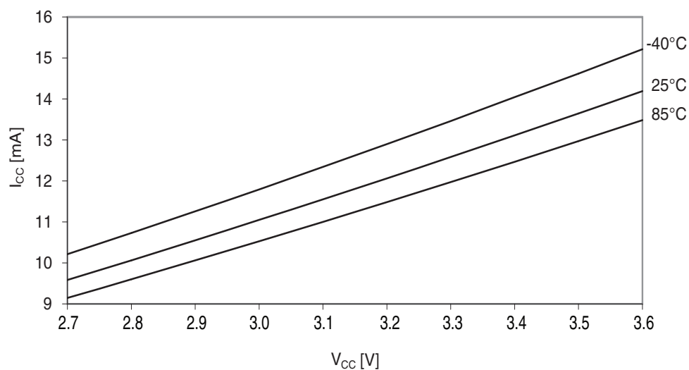
Figure 37-173. Active mode supply current vs. V_{CC} .
