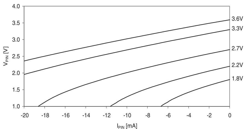
Figure 37-192. I/O pin output voltage vs. source current.
