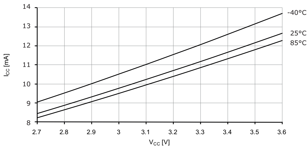
Figure 37-7. Active mode supply current vs. V_{CC} .
