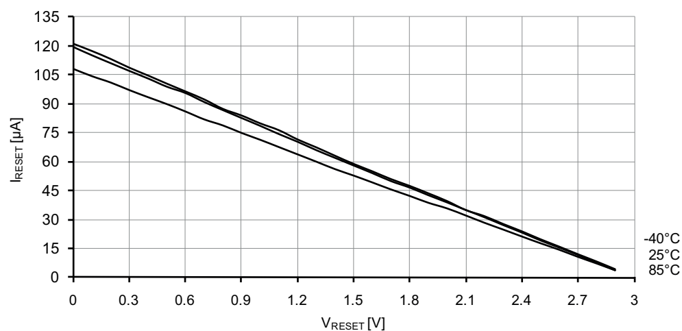
Figure 37-147. Reset pin pull-up resistor current vs. reset pin voltage.
