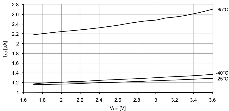
Figure 37-99. Power-down mode supply current vs. V_{CC} . Watchdog and sampled BOD enabled.
