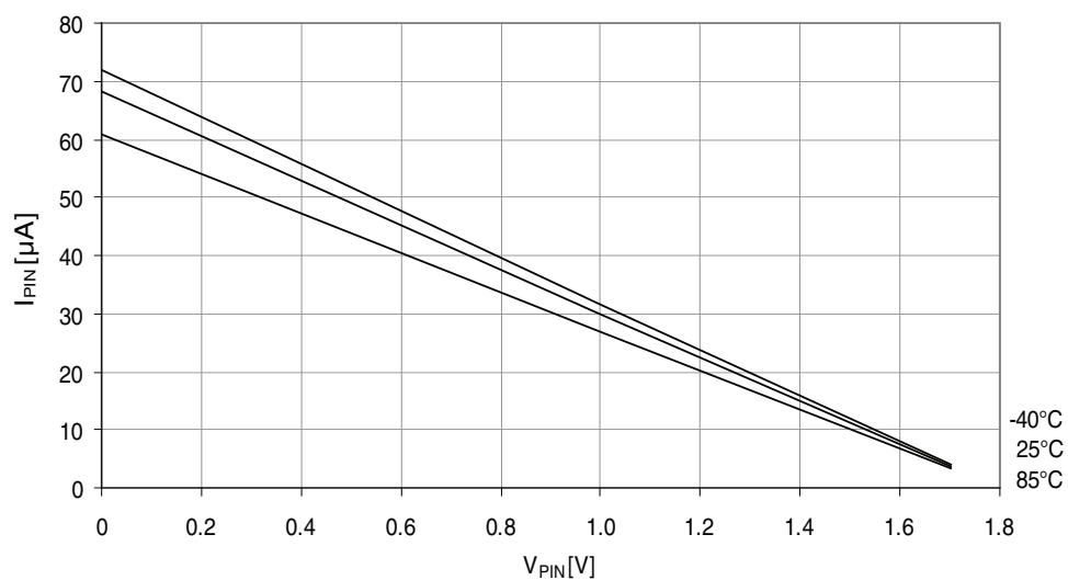
Figure 37-186. I/O pin pull-up resistor current vs. input voltage. V_{CC} = 1.8V .
