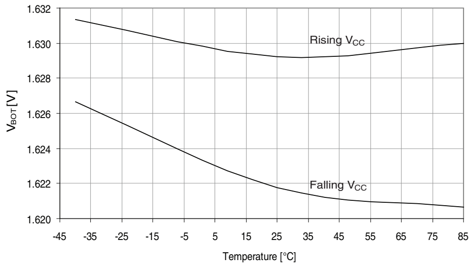
Figure 37-308. BOD thresholds vs. temperature. BOD level = 1.6V.
