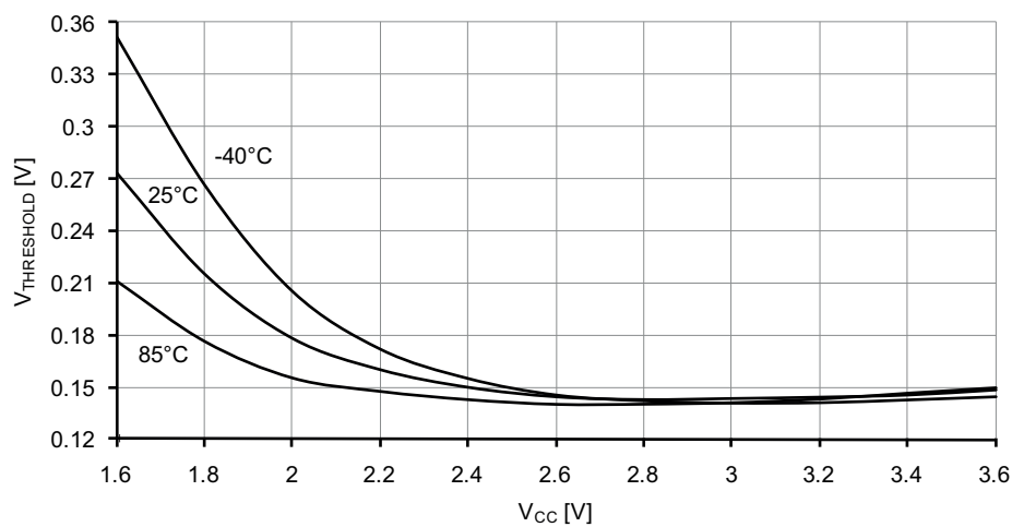
Figure 37-34. I/O pin input hysteresis vs. V_{CC} .
