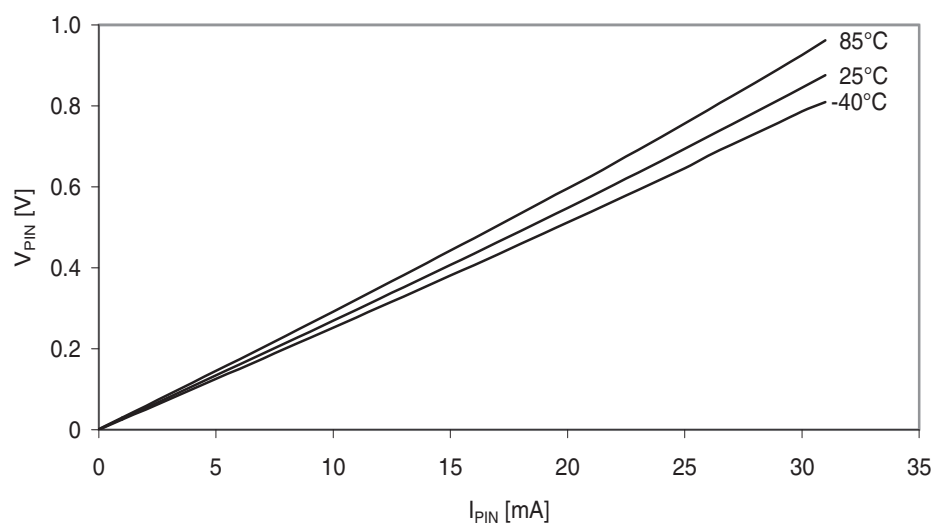
Figure 37-279. I/O pin output voltage vs. sink current.
