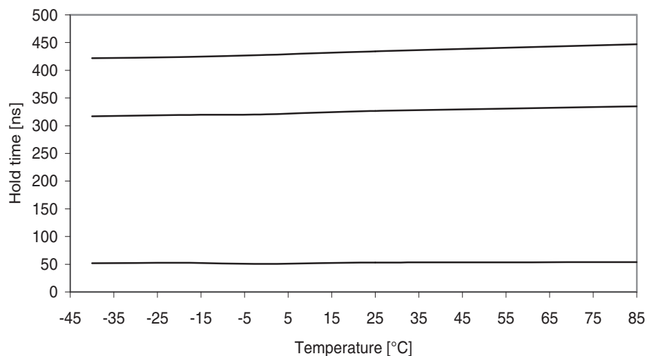
Figure 37-247. SDA hold time vs. temperature.
