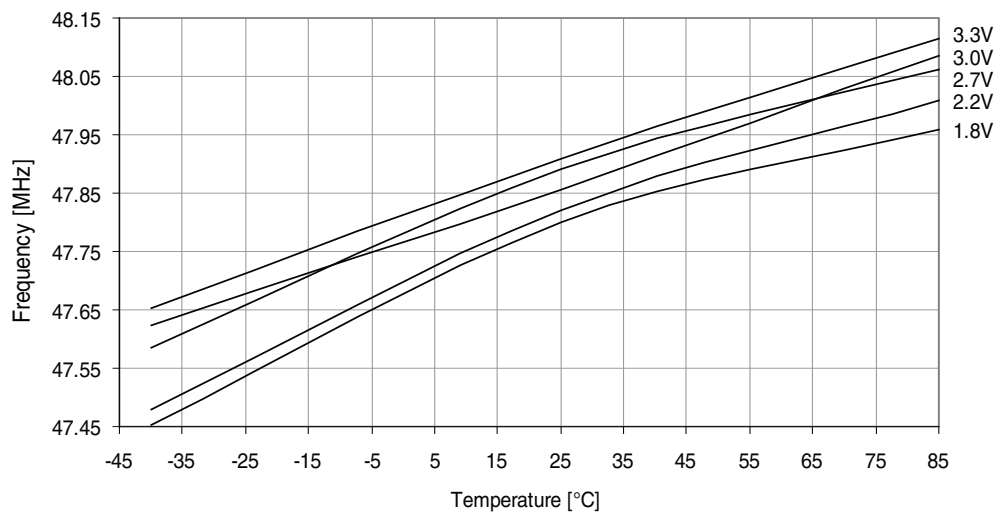
Figure 37-245. 48MHz internal oscillator frequency vs. temperature.
