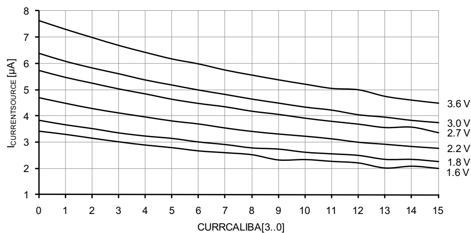
Figure 37-56. Analog comparator current source vs. calibration value.
