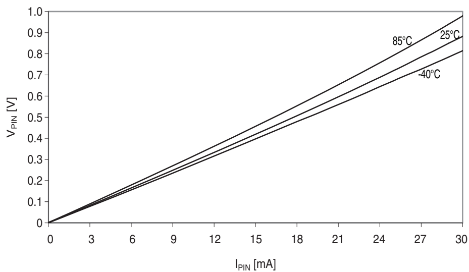
Figure 37-194. I/O pin output voltage vs. sink current.
