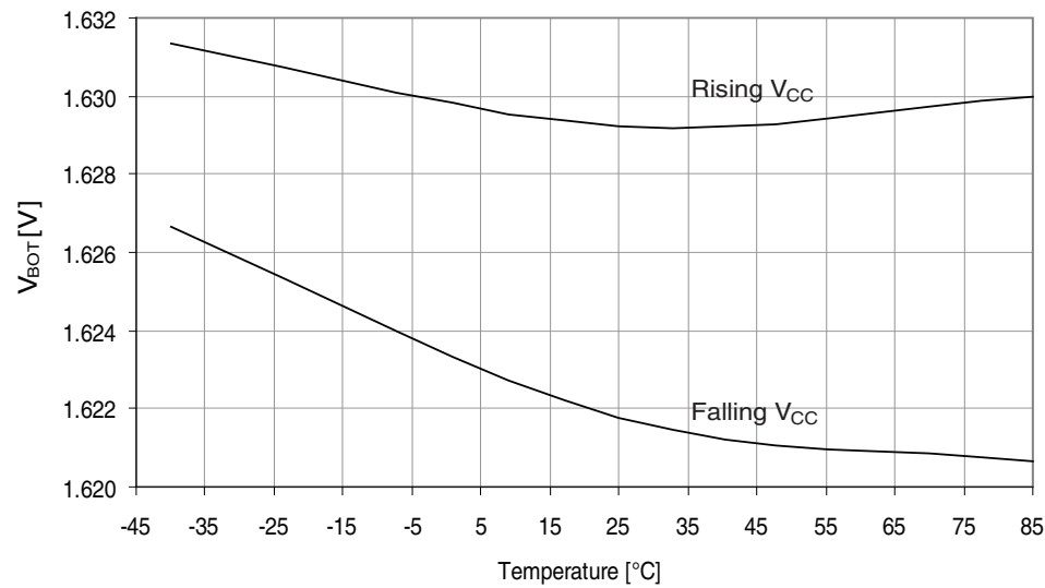
Figure 37-225. BOD thresholds vs. temperature.
