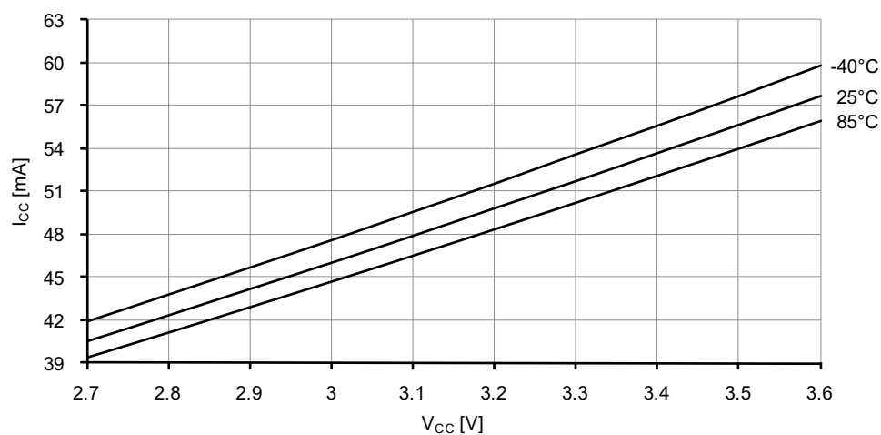
Figure 37-97. Idle mode current vs. V_{CC} .
