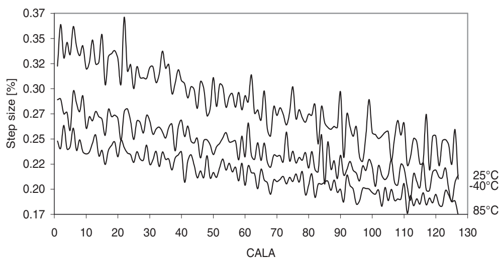
Figure 37-239. 2MHz internal oscillator CALA calibration step size.
