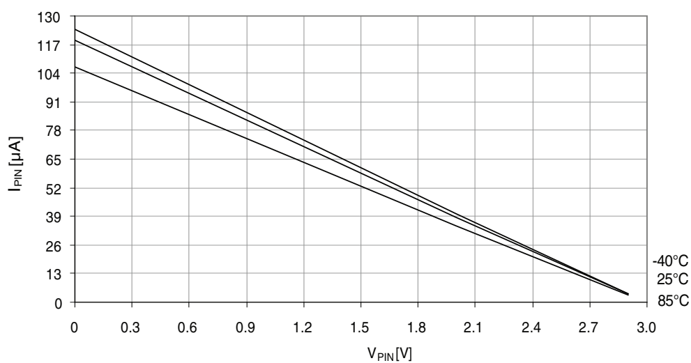
Figure 37-270. I/O pin pull-up resistor current vs. input voltage.
