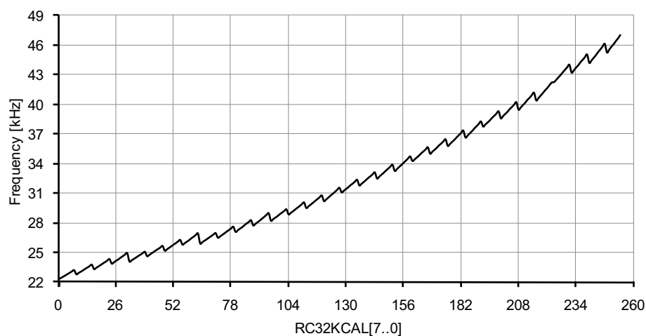
Figure 37-70. 32.768kHz internal oscillator frequency vs. calibration value.
