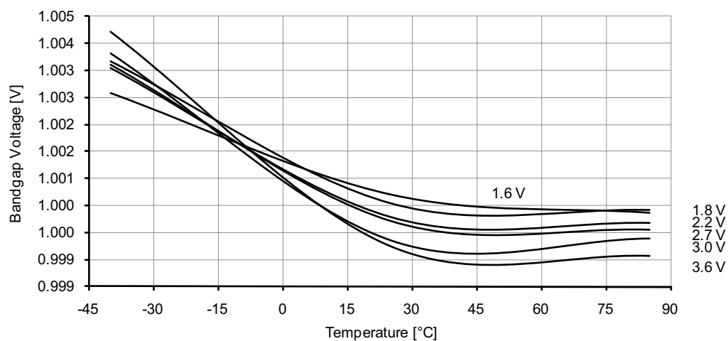
Figure 37-141. ADC/DAC Internal 1.0V reference vs. temperature.
