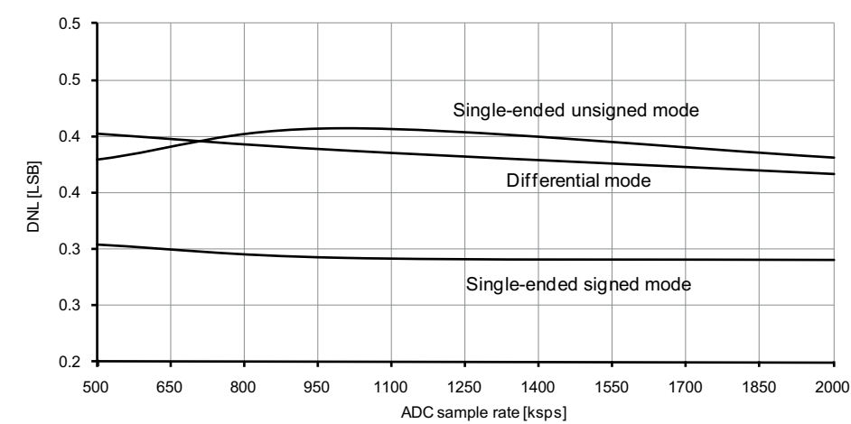
Figure 37-39. DNL error vs. sample rate. T = 25\text{ }^{\circ}\text{C} , V_{CC} = 2.7\text{V} , V_{REF} = 1.0\text{V external} .
