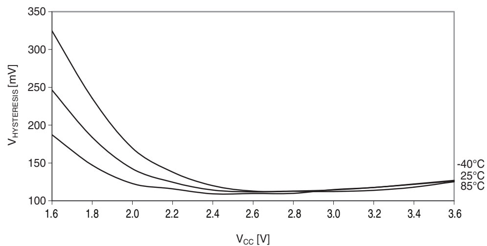
Figure 37-200. I/O pin input hysteresis vs. V_{CC} .
