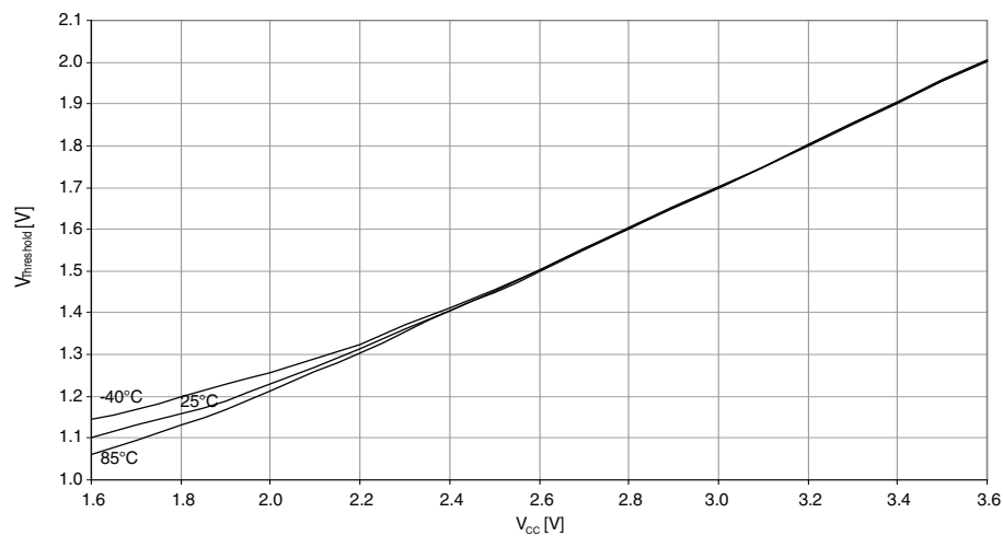
Figure 37-231. Reset pin input threshold voltage vs. V_{CC} .
