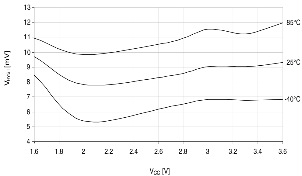
Figure 37-135. Analog comparator hysteresis vs. V_{CC} .
