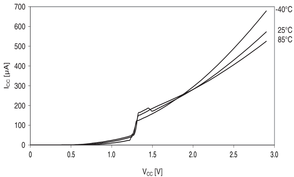
Figure 37-233. Power-on reset current consumption vs. V_{CC} . BOD level = 3.0V, enabled in continuous mode.
