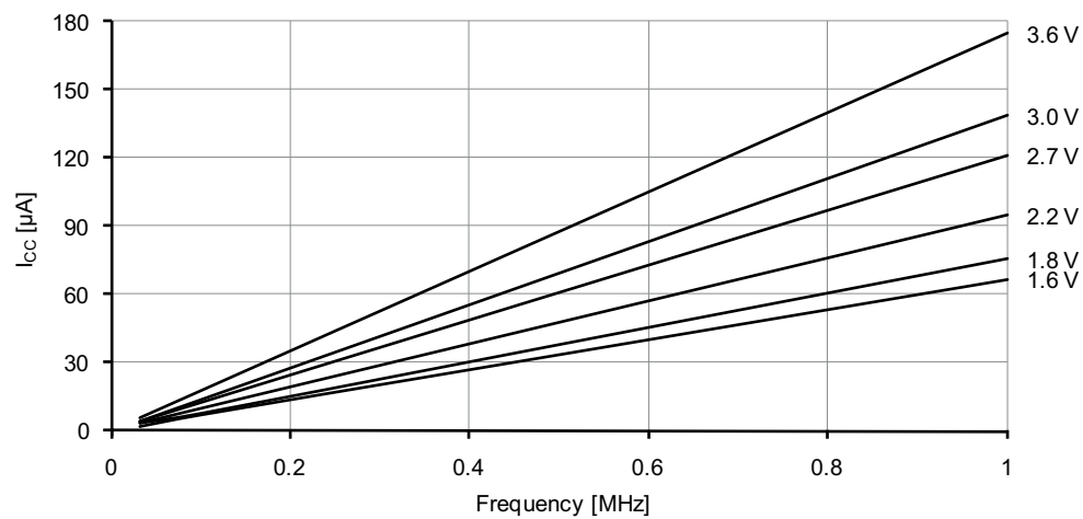
Figure 37-91. Idle mode supply current vs. frequency.
