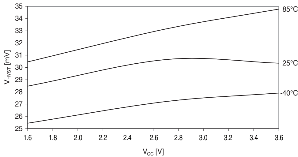
Figure 37-218. Analog comparator hysteresis vs. V_{CC} . Low power, small hysteresis.
