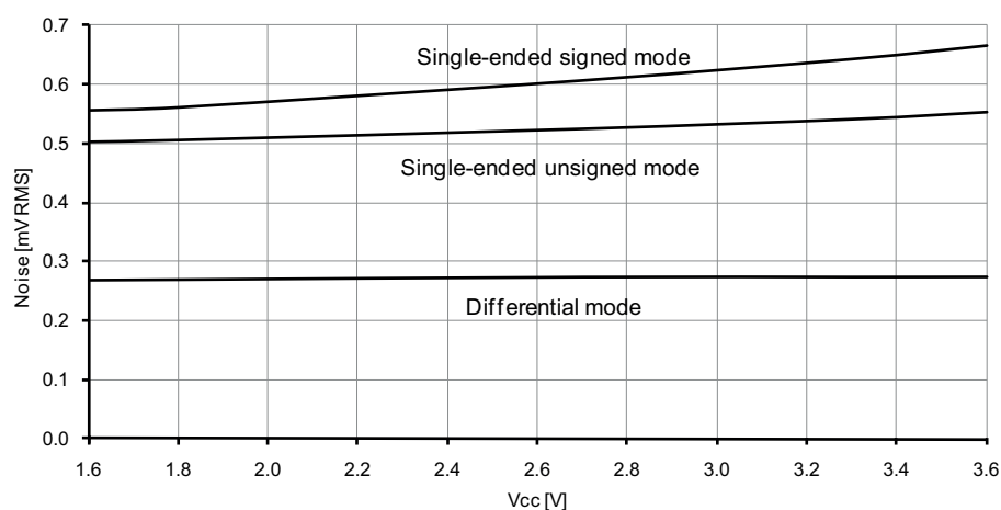
Figure 37-47. Noise vs. V_{CC} .
