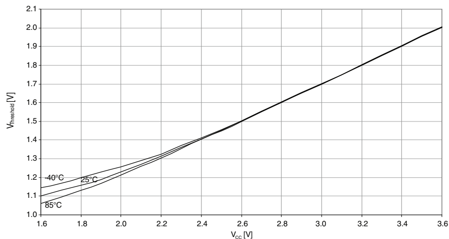
Figure 37-314. Reset pin input threshold voltage vs. V_{CC} .
