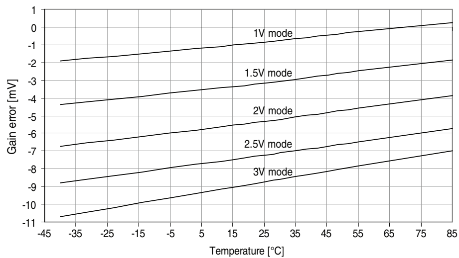
Figure 37-293. Gain error vs. temperature.
