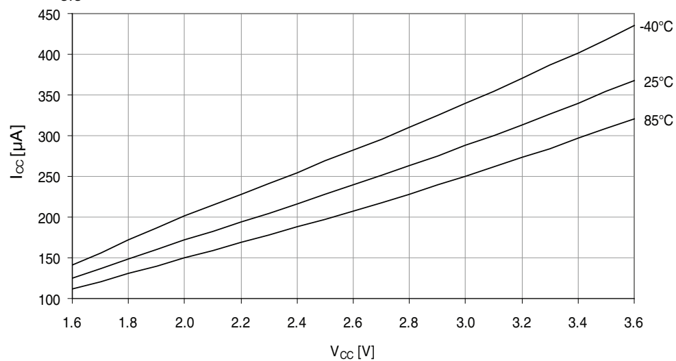
Figure 37-252. Active mode supply current vs. V_{CC} .
