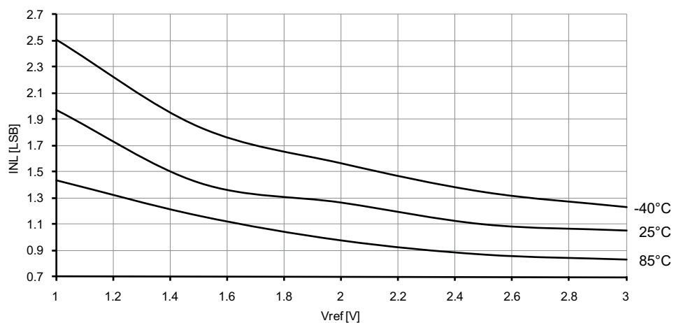
Figure 37-131. DAC INL error vs. V_{REF} .
