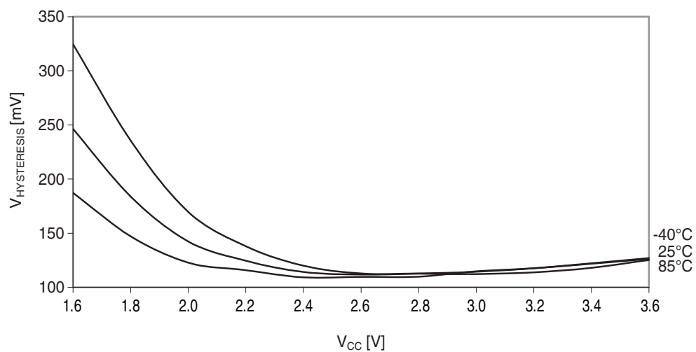
Figure 37-283. I/O pin input hysteresis vs. V_{CC} .
