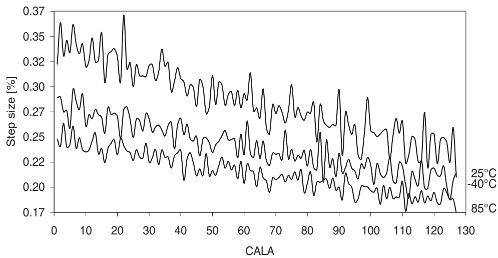
Figure 37-322. 2MHz internal oscillator CALA calibration step size.
