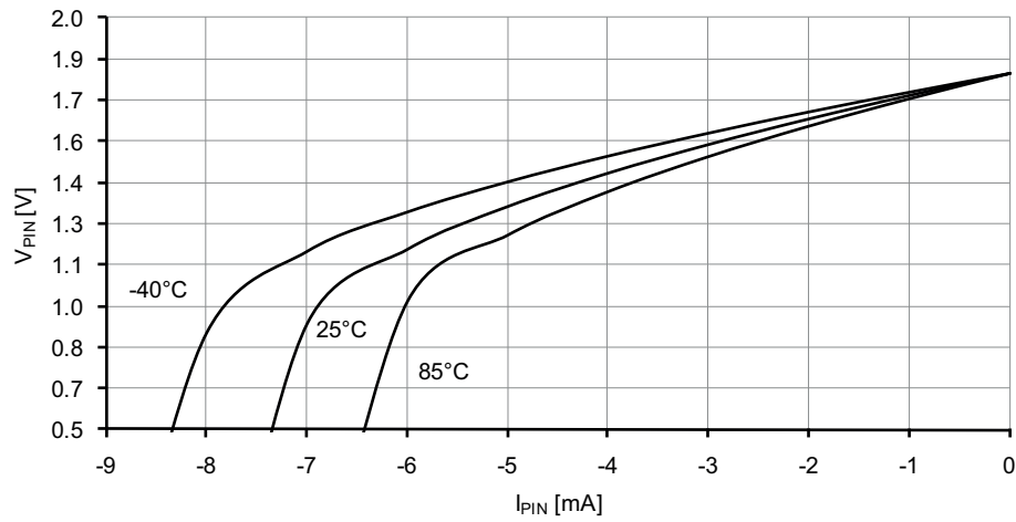
Figure 37-107. I/O pin output voltage vs. source current.
