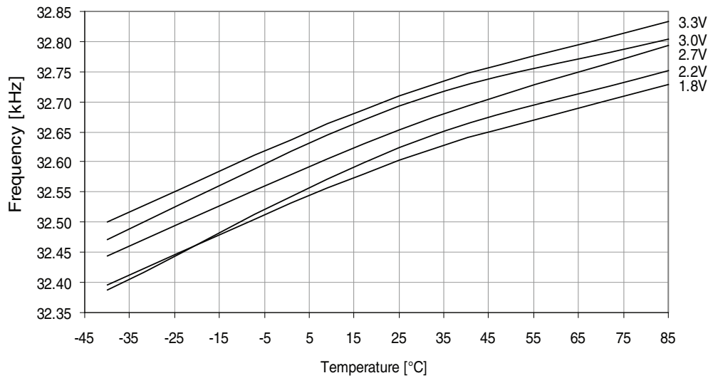
Figure 37-235. 32.768kHz internal oscillator frequency vs. temperature.
