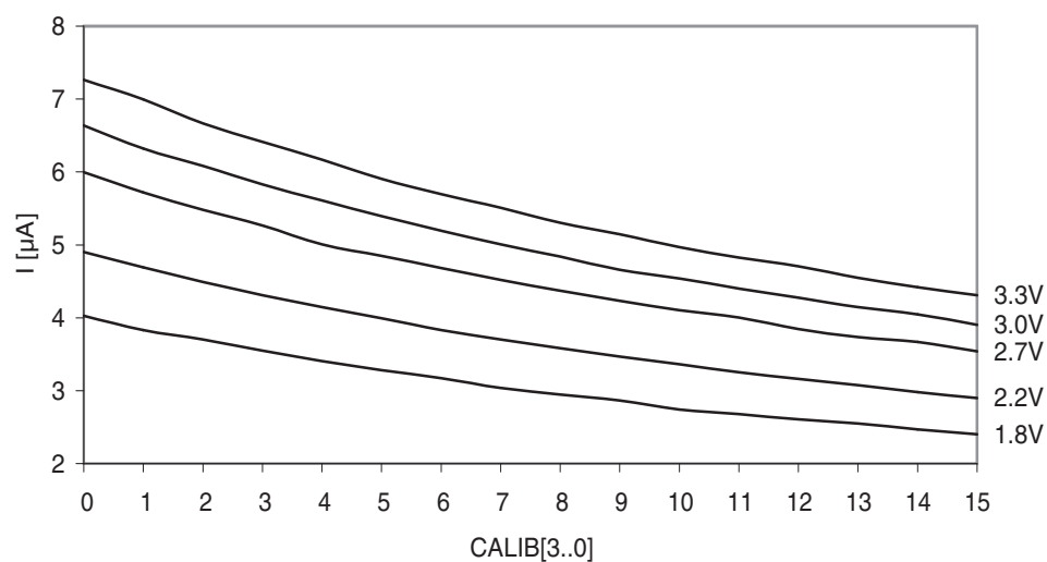
Figure 37-221. Analog comparator current source vs. calibration value.
