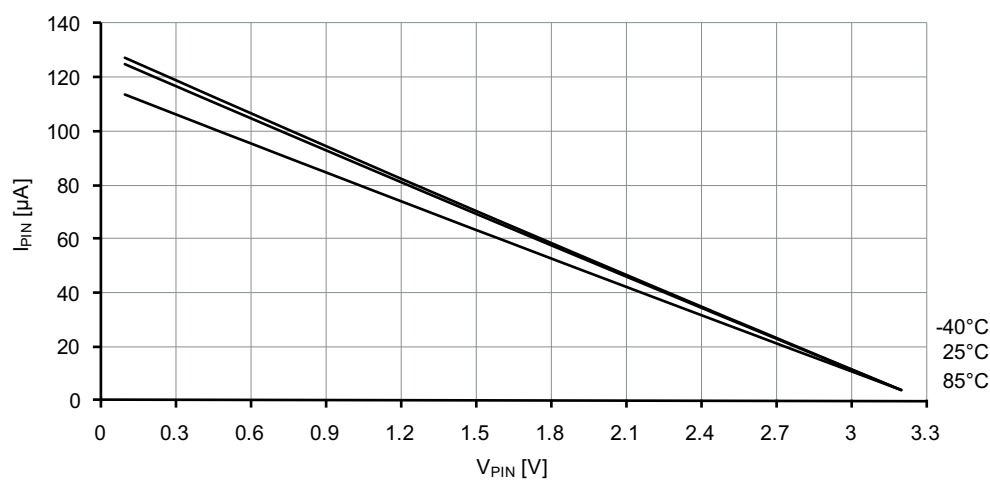
Figure 37-105. I/O pin pull-up resistor current vs. input voltage.
