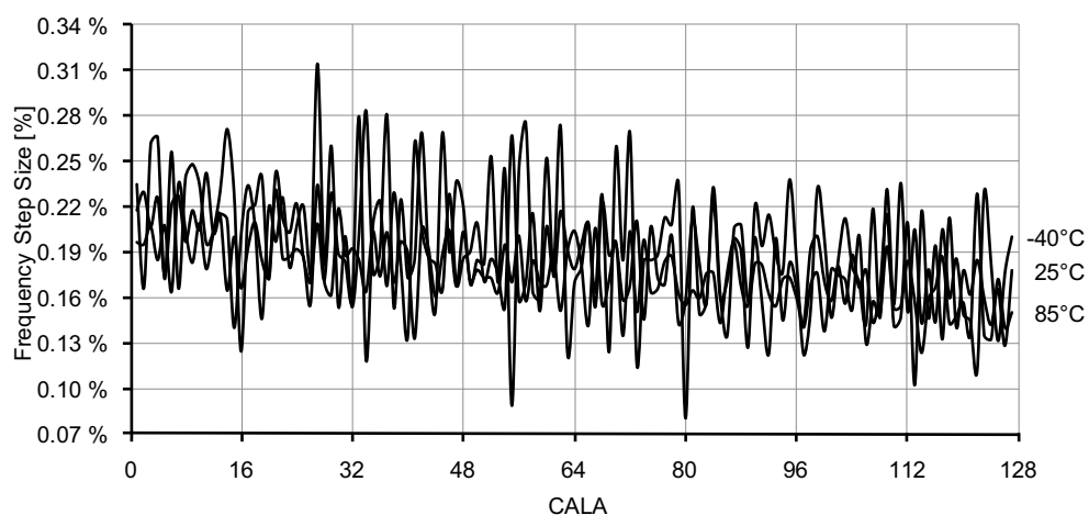
Figure 37-163. 48MHz internal oscillator CALA calibration step size.
