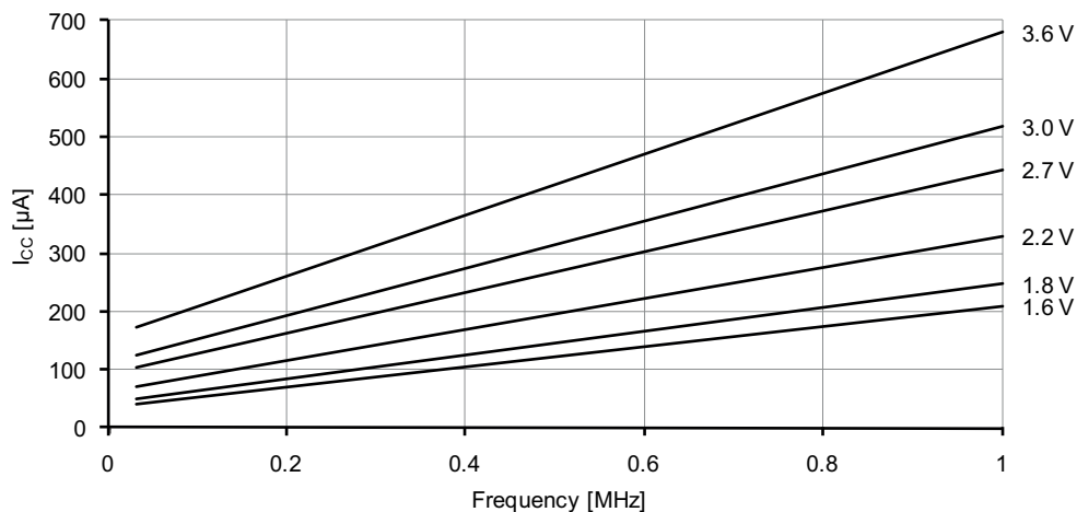
Figure 37-2. Active supply current vs. frequency.
