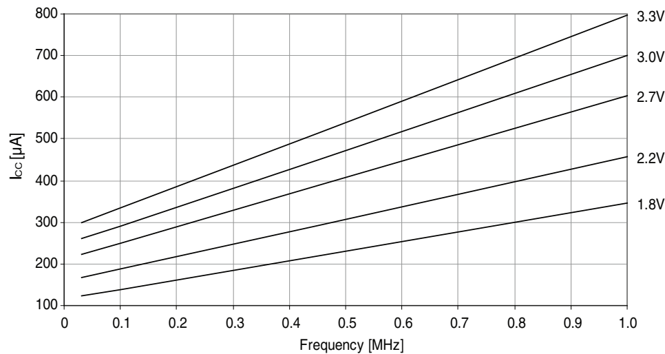
Figure 37-250. Active supply current vs. frequency.
