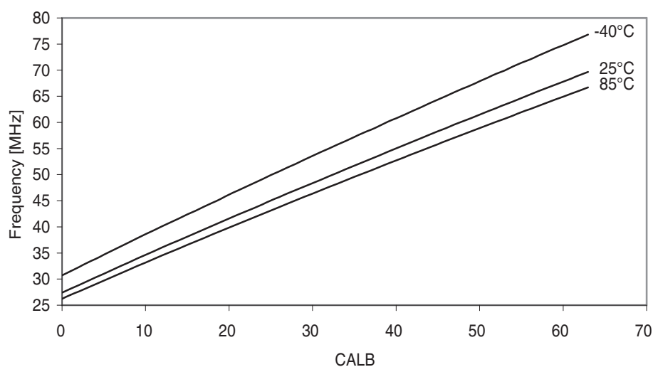
Figure 37-326. 32MHz internal oscillator frequency vs. CALB calibration value.
