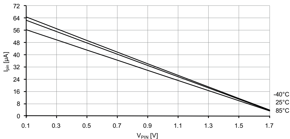
Figure 37-20. I/O pin pull-up resistor current vs. input voltage. V_{CC} = 1.8V .
