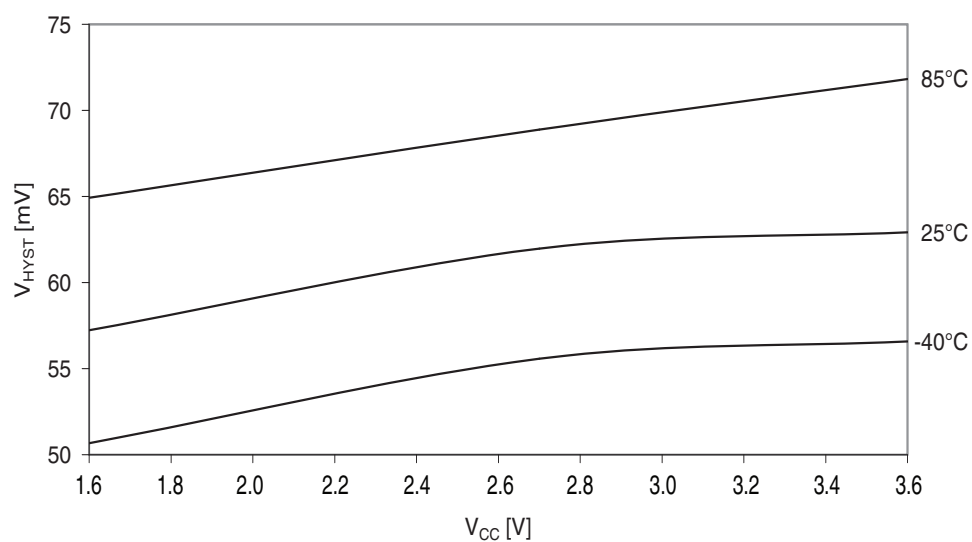
Figure 37-303. Analog comparator hysteresis vs. V_{CC} . Low power, large hysteresis.
