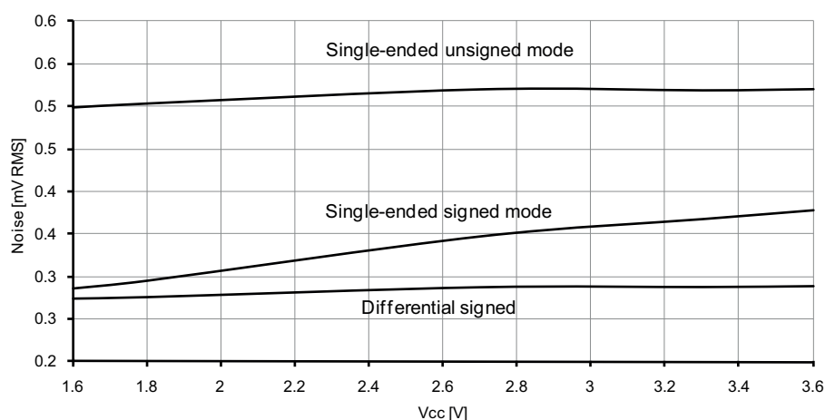
Figure 37-130. Noise vs. V_{CC} .
