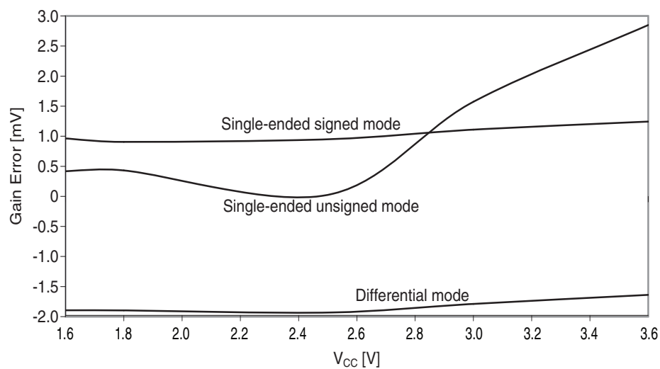
Figure 37-291. Gain error vs. V_{CC} .
