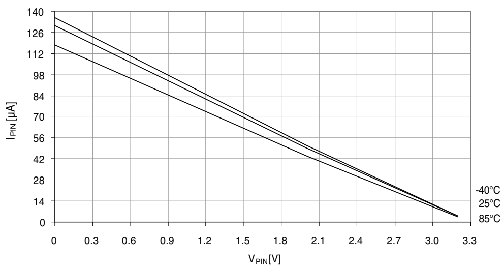
Figure 37-188. I/O pin pull-up resistor current vs. input voltage.
