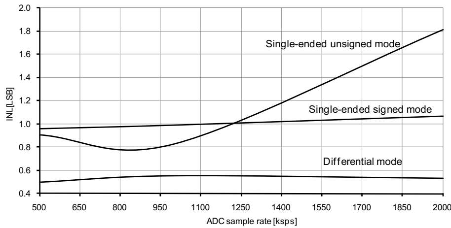
Figure 37-36. INL error vs. sample rate. T = 25\text{ }^{\circ}\text{C} , V_{CC} = 2.7\text{V} , V_{REF} = 1.0\text{V} external.
