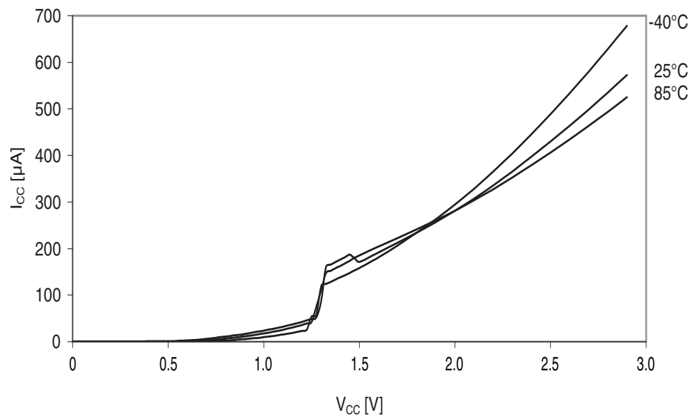
Figure 37-316. Power-on reset current consumption vs. V_{CC} . BOD level = 3.0V, enabled in continuous mode.
