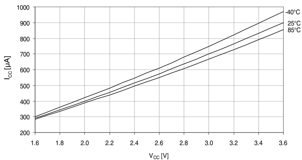
Figure 37-170. Active mode supply current vs. V_{CC} .
