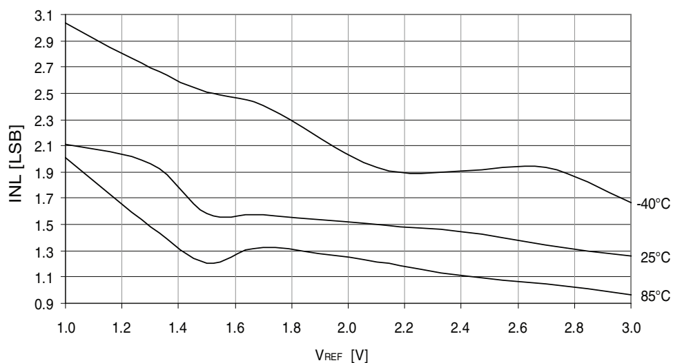
Figure 37-214. DAC INL error vs. V_{REF} .
