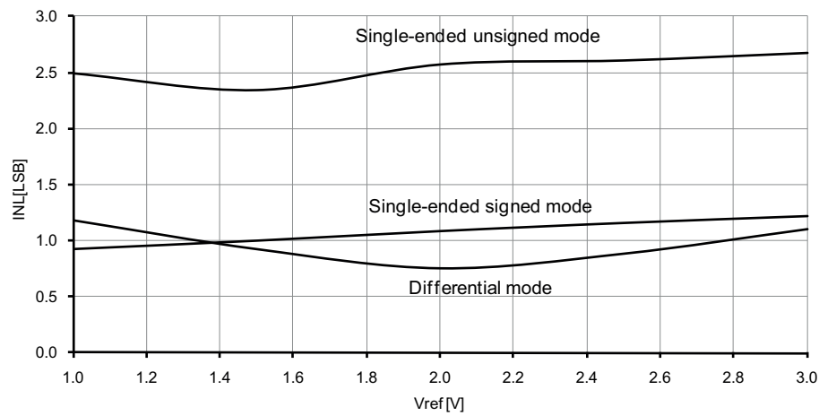
Figure 37-35. INL error vs. external V_{REF} . T = 25\text{ }^{\circ}\text{C} , V_{CC} = 3.6\text{V} , external reference.
