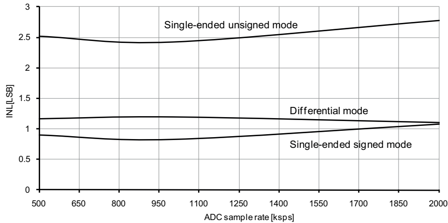
Figure 37-119. INL error vs. sample rate. T = 25\text{ }^{\circ}\text{C} , V_{CC} = 3.6\text{V} , V_{REF} = 3.0\text{V} external.
