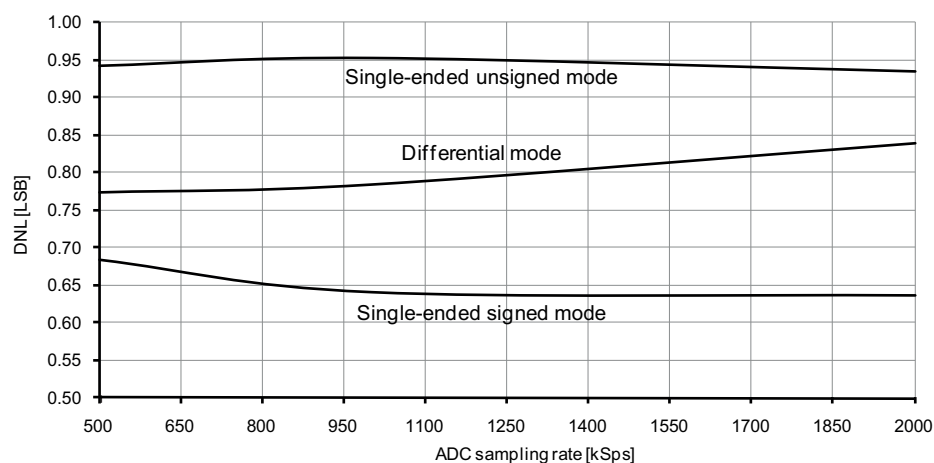
Figure 37-122. DNL error vs. sample rate.
