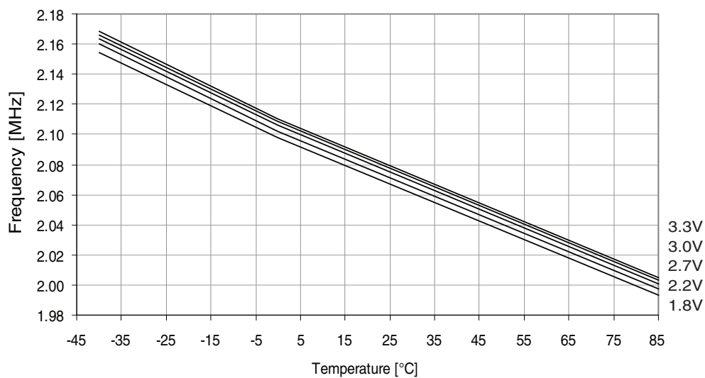
Figure 37-237. 2MHz internal oscillator frequency vs. temperature.
