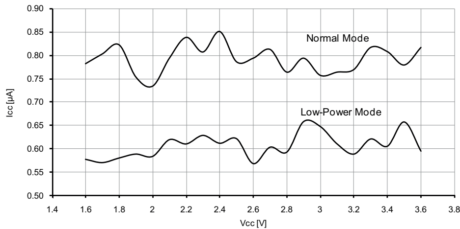
Figure 37-17. Power-save mode supply current vs. V_{CC} .
