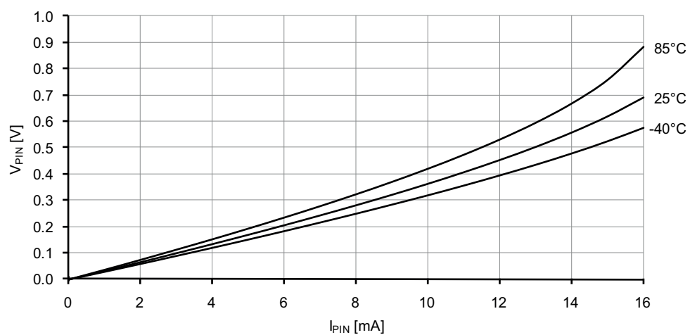
Figure 37-111. I/O pin output voltage vs. sink current.
