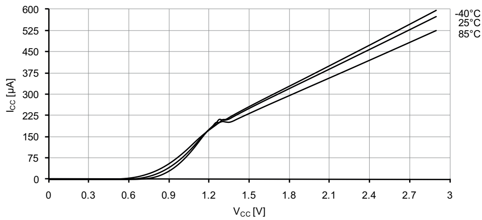
Figure 37-67. Power-on reset current consumption vs. V_{CC} . BOD level = 3.0V, enabled in continuous mode.
