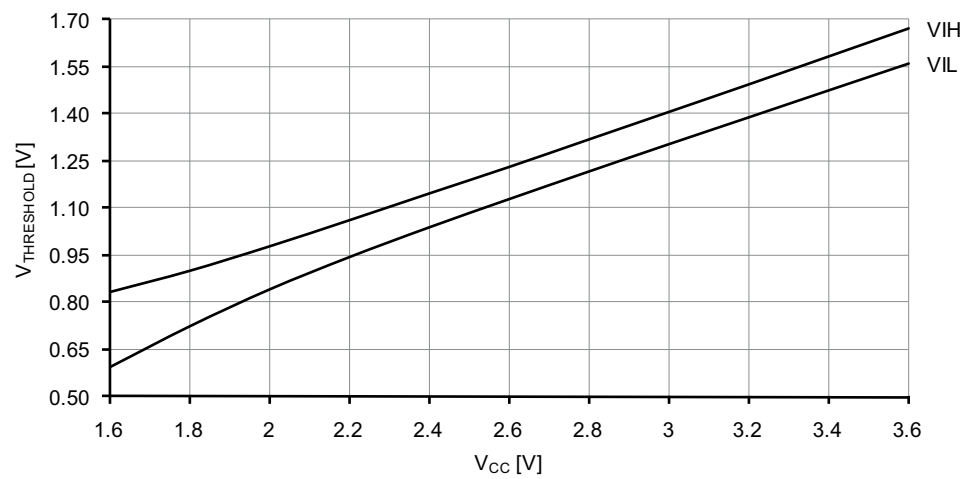
Figure 37-114. I/O pin input threshold voltage vs. V_{CC} . T = 25^{\circ}\text{C} .
