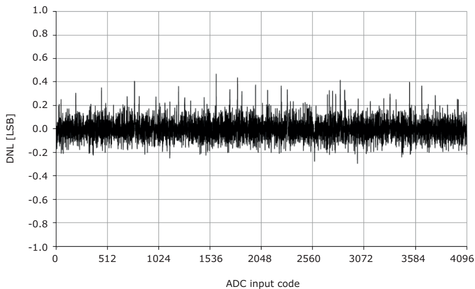
Figure 37-123. DNL error vs. input code.
