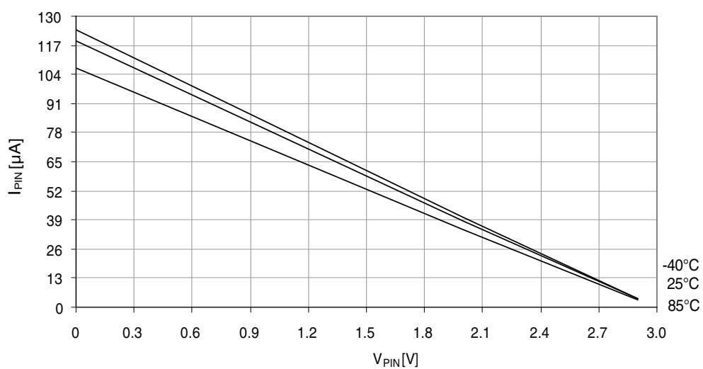
Figure 37-187. I/O pin pull-up resistor current vs. input voltage.
