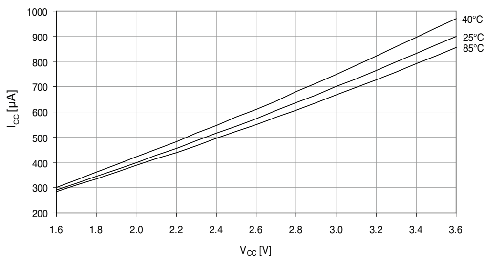
Figure 37-253. Active mode supply current vs. V_{CC} .
