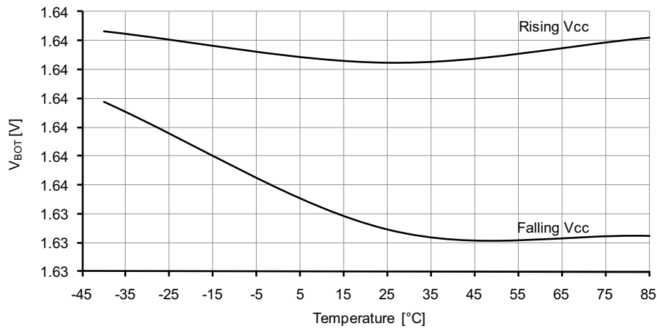
Figure 37-142. BOD thresholds vs. temperature. BOD level = 1.6V.
