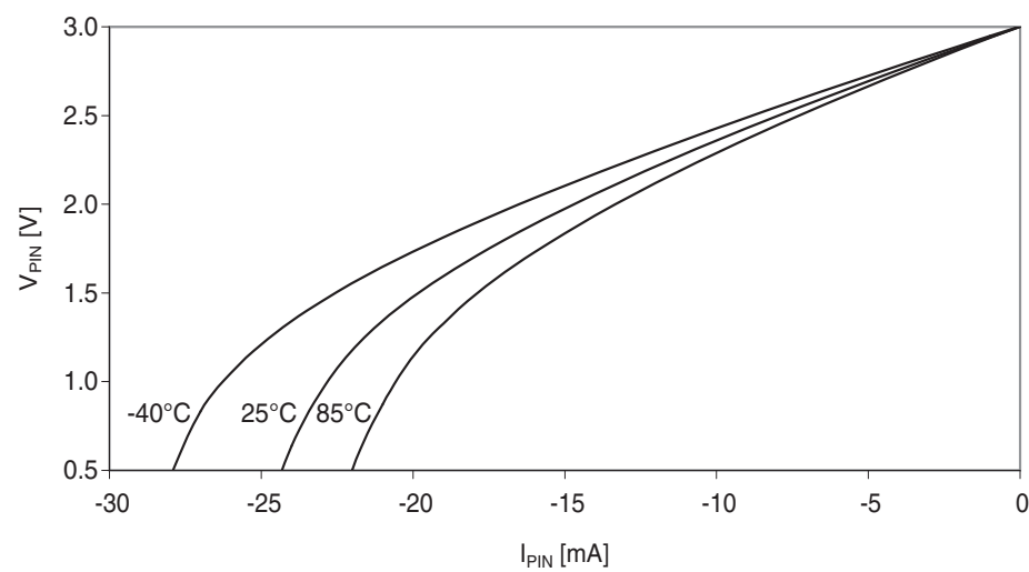
Figure 37-190. I/O pin output voltage vs. source current. V_{CC} = 3.0V .
