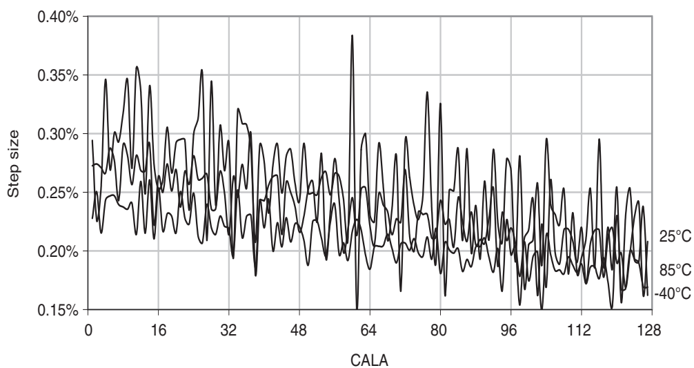
Figure 37-329. 48MHz internal oscillator CALA calibration step size.
