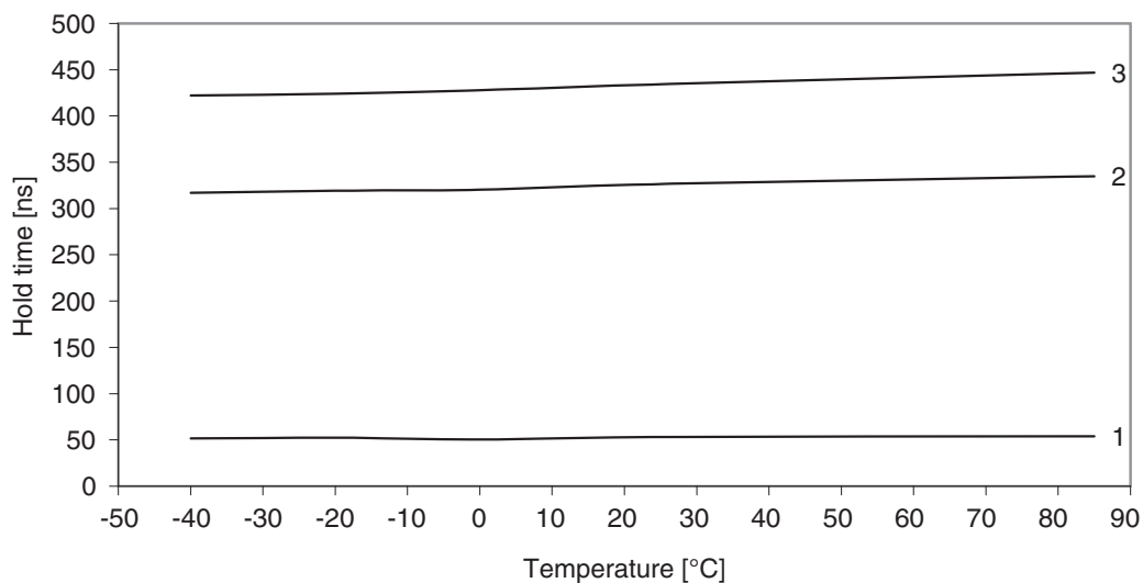
Figure 37-81. SDA hold time vs. temperature.
