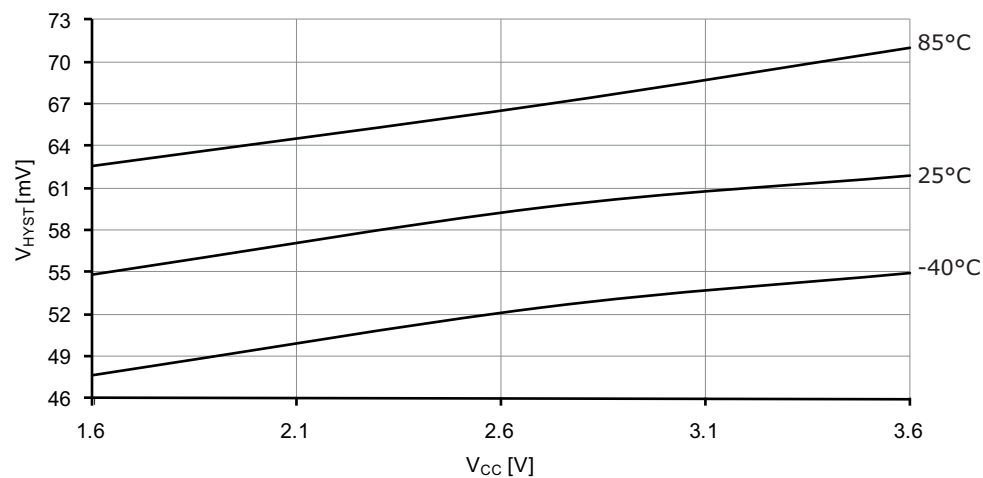
Figure 37-54. Analog comparator hysteresis vs. V_{CC} . Low power, large hysteresis.
