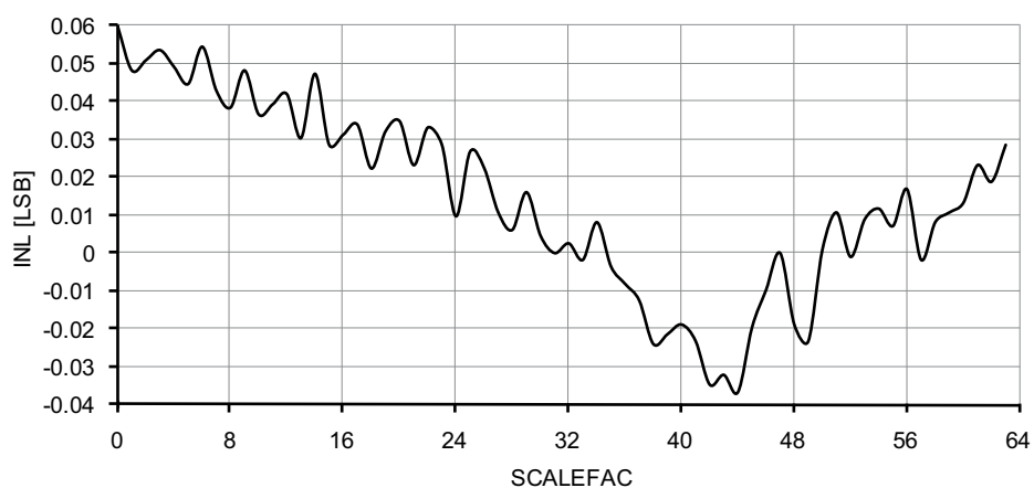
Figure 37-57. Voltage scaler INL vs. SCALEFAC.
