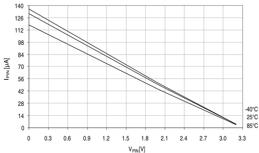
Figure 37-313. Reset pin pull-up resistor current vs. reset pin voltage.
